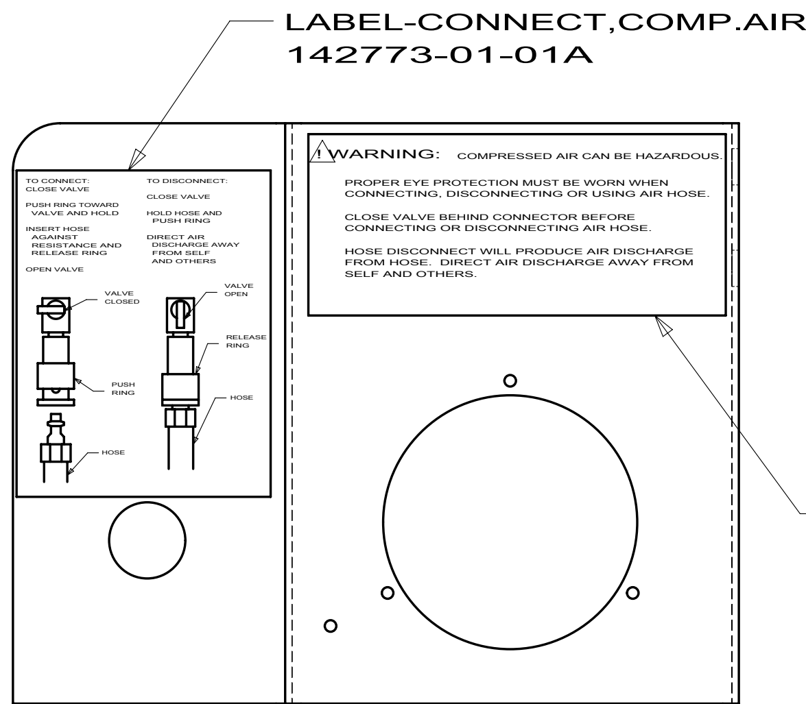
AIR ACCESS PANEL
