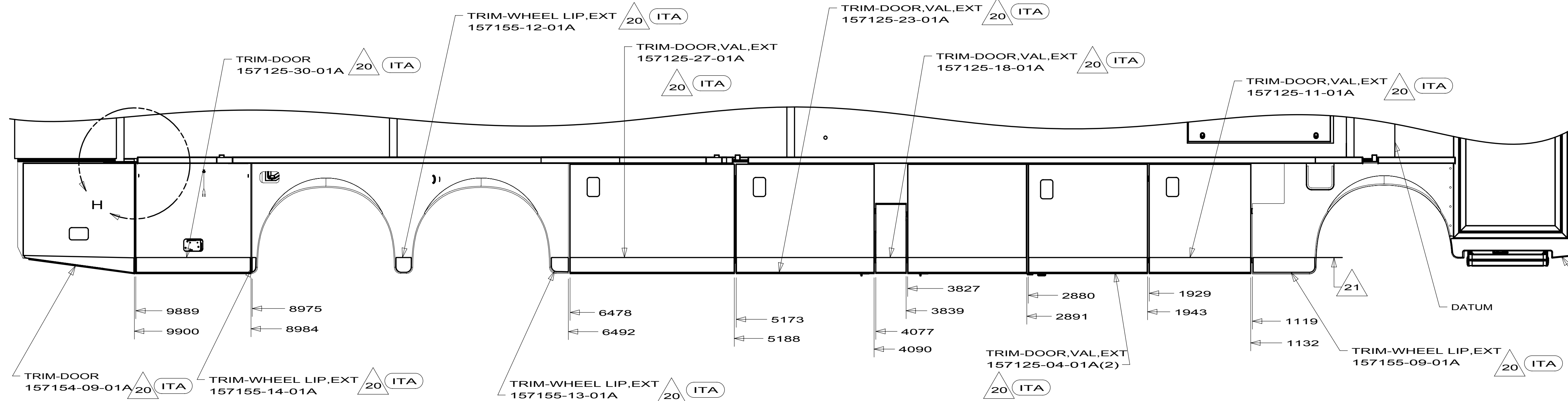
RIGHT SIDE COMPARTMENT DOORS
