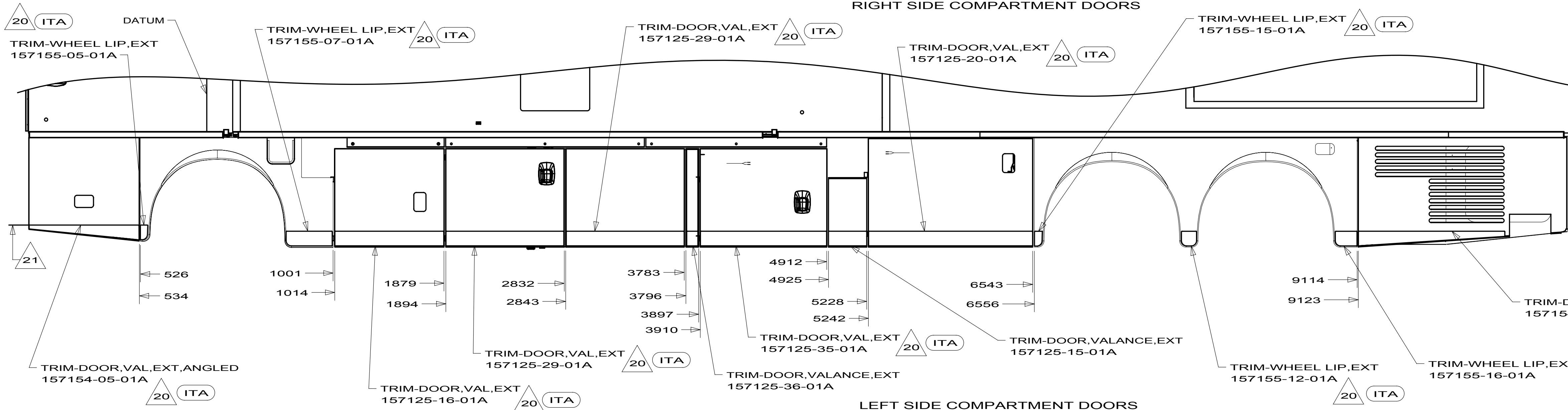
LEFT SIDE COMPARTMENT DOORS
