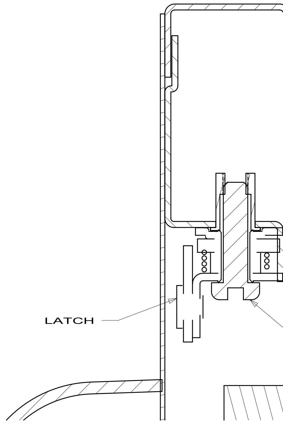
SECTION C-C
