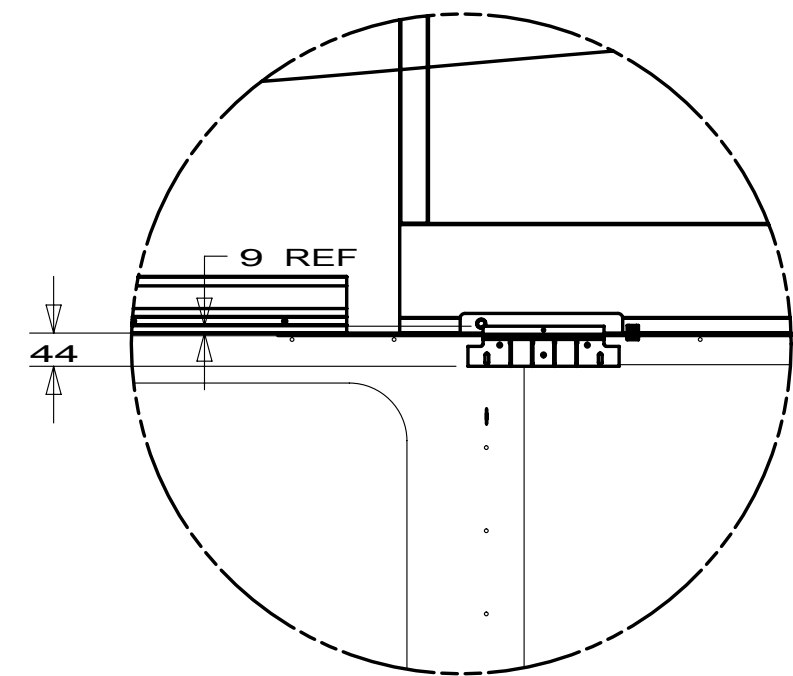
DETAIL H (SHOWN WITHOUT DOORS)
