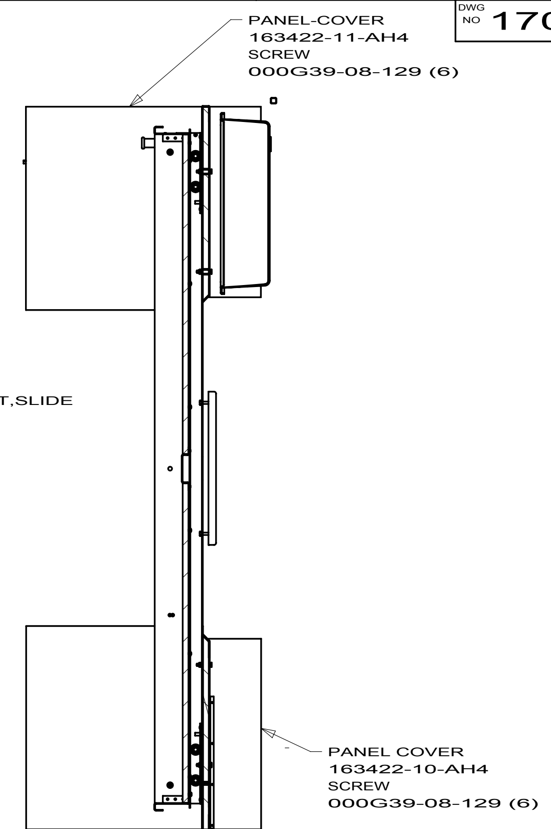
SECTION C-C
