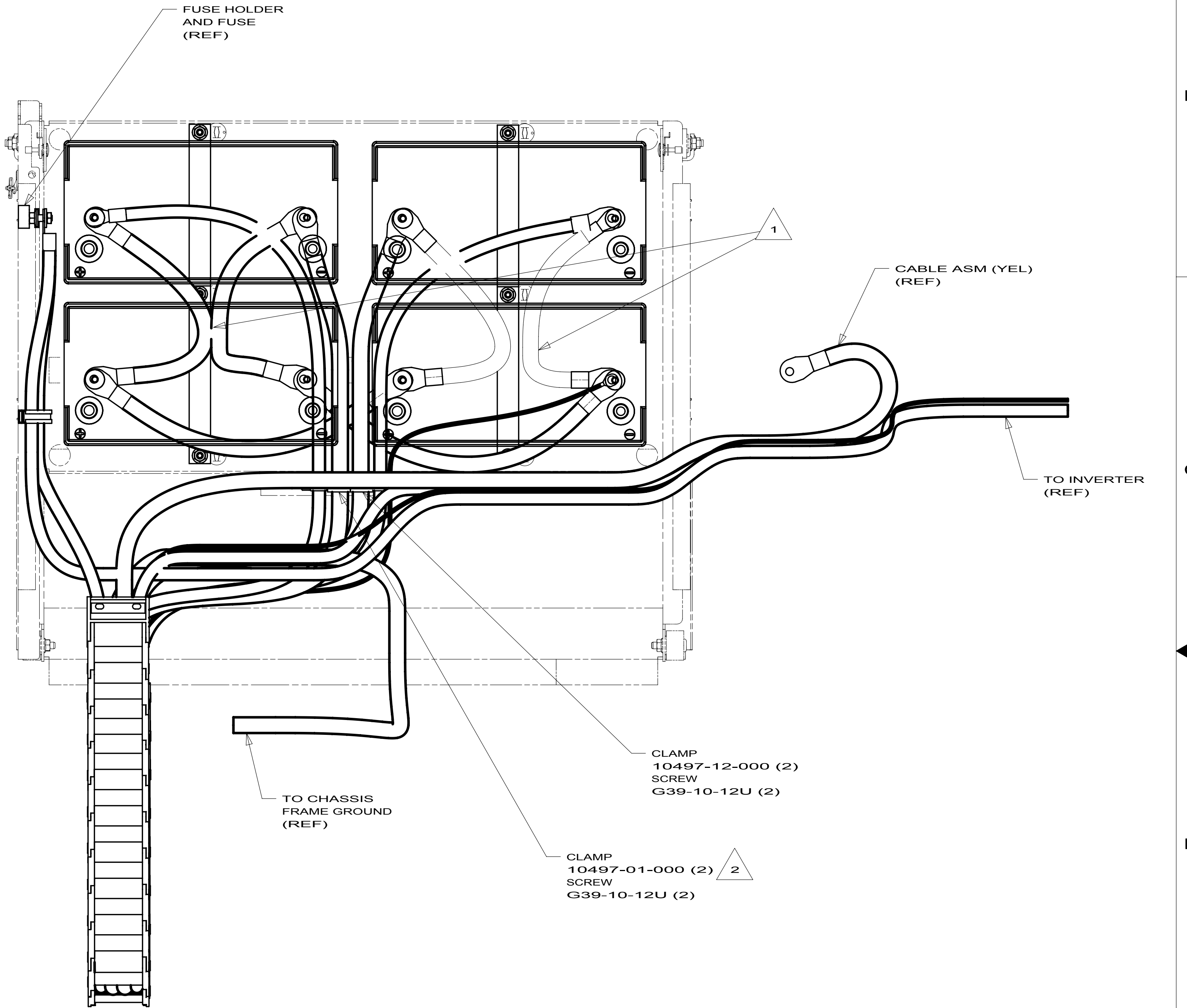
COACH BATTERIES (TOP VIEW) (RIGHTHAND BATTERIES SHOWN LEFTHAND OPPOSITE) (TAB -02)
