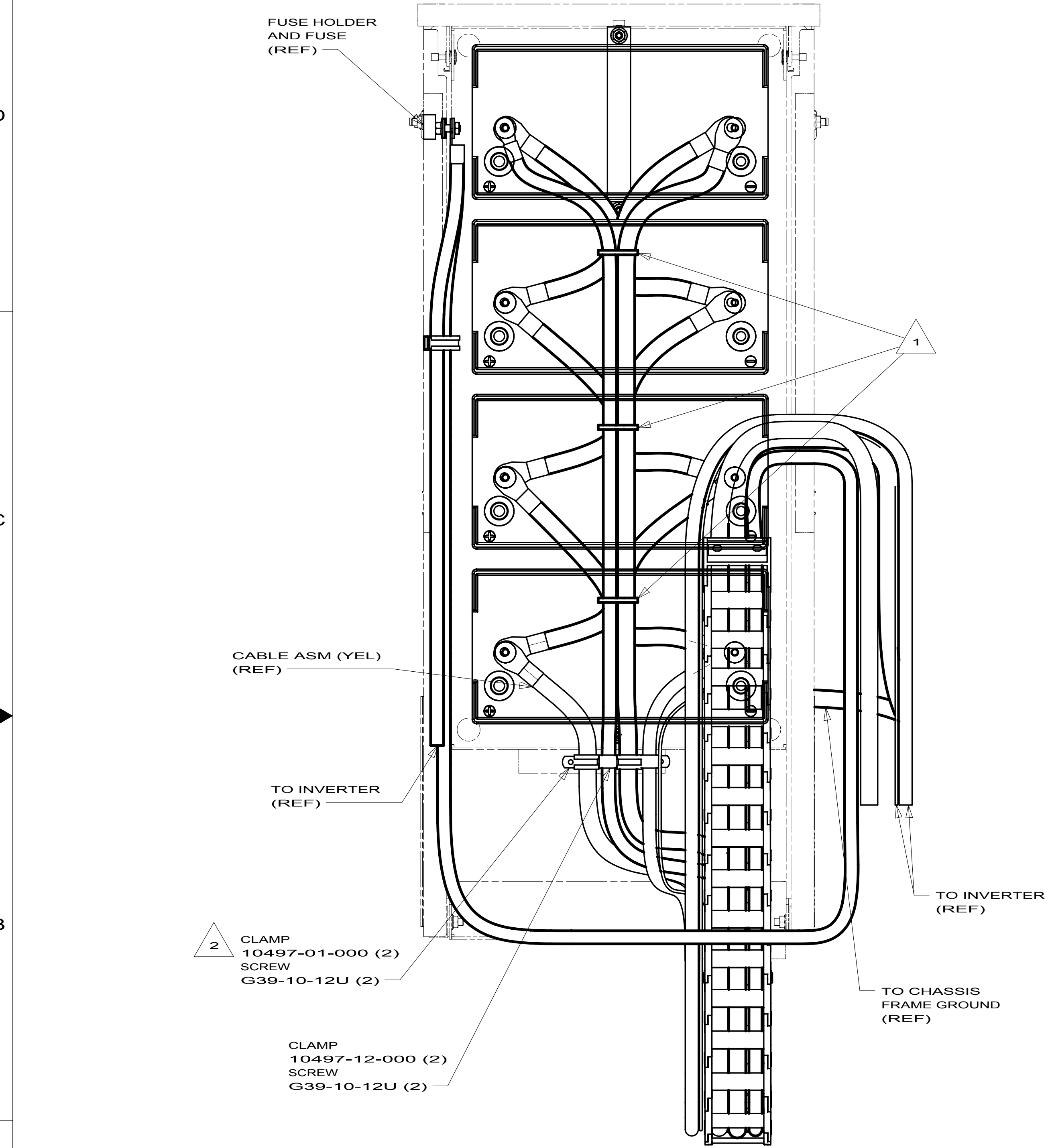
COACH BATTERIES (TOP VIEW) (RIGHTHAND BATTERIES SHOWN LEFTHAND OPPOSITE) (TAB -01)
