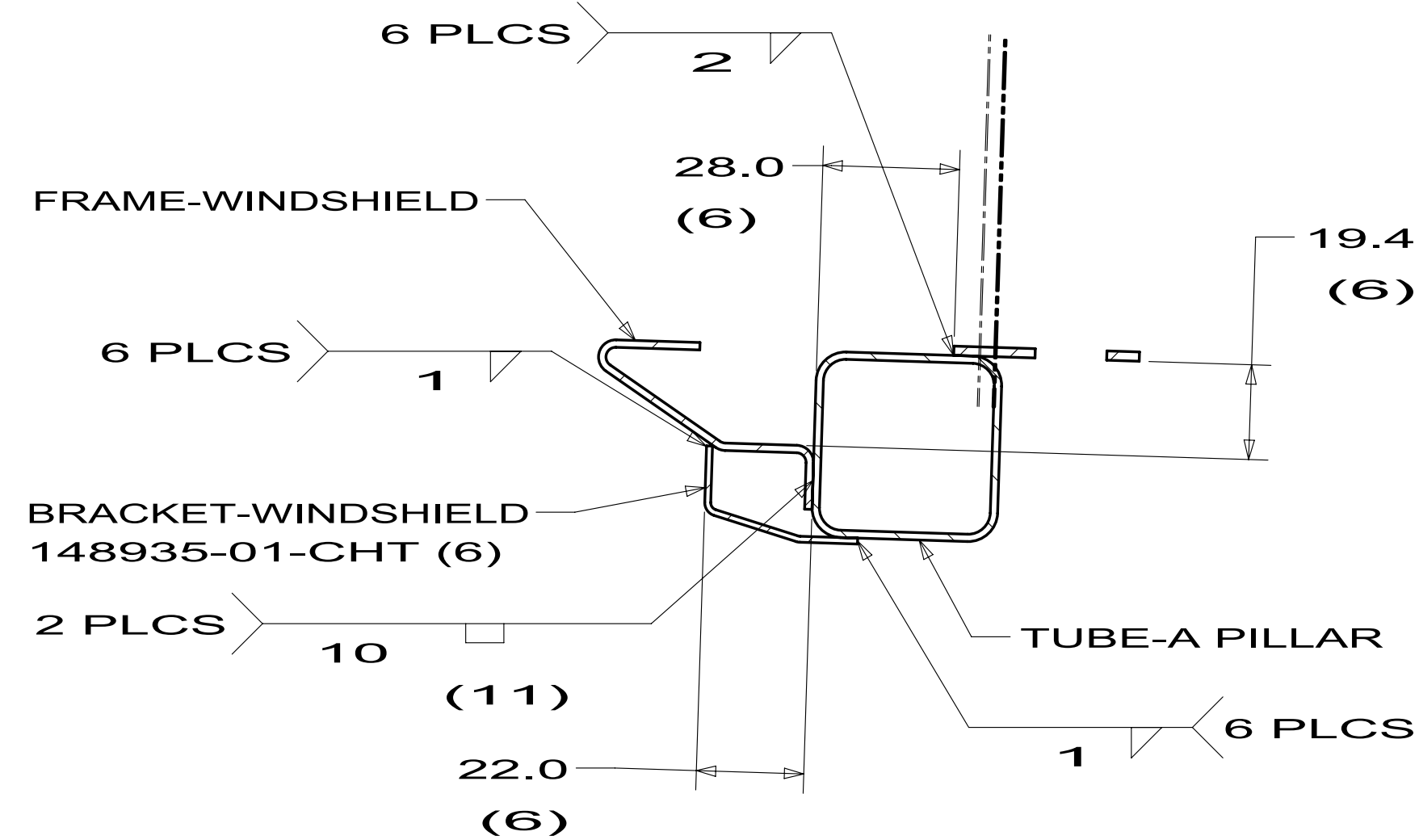
SECTION EC-EC
