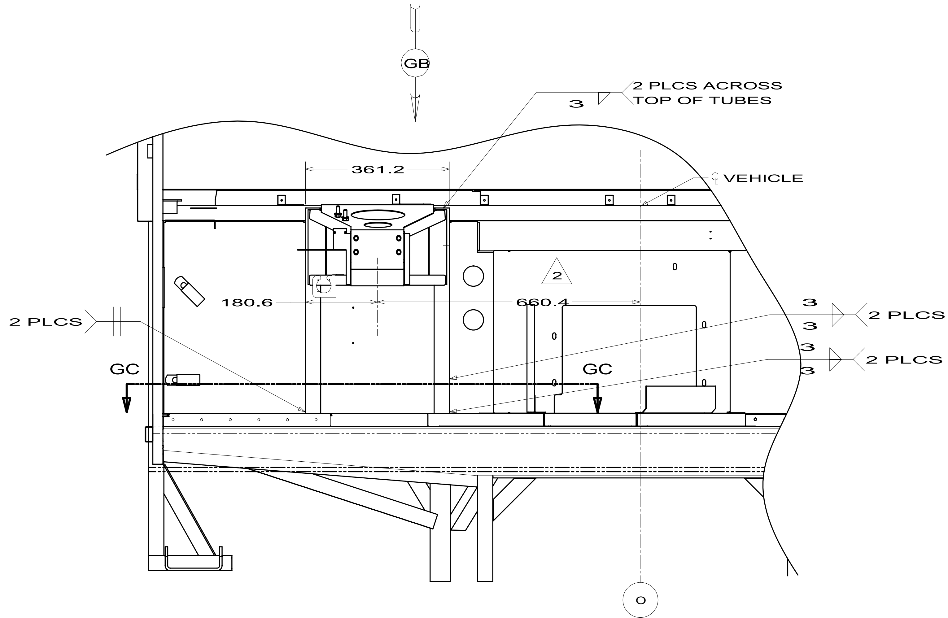
VIEW GA
