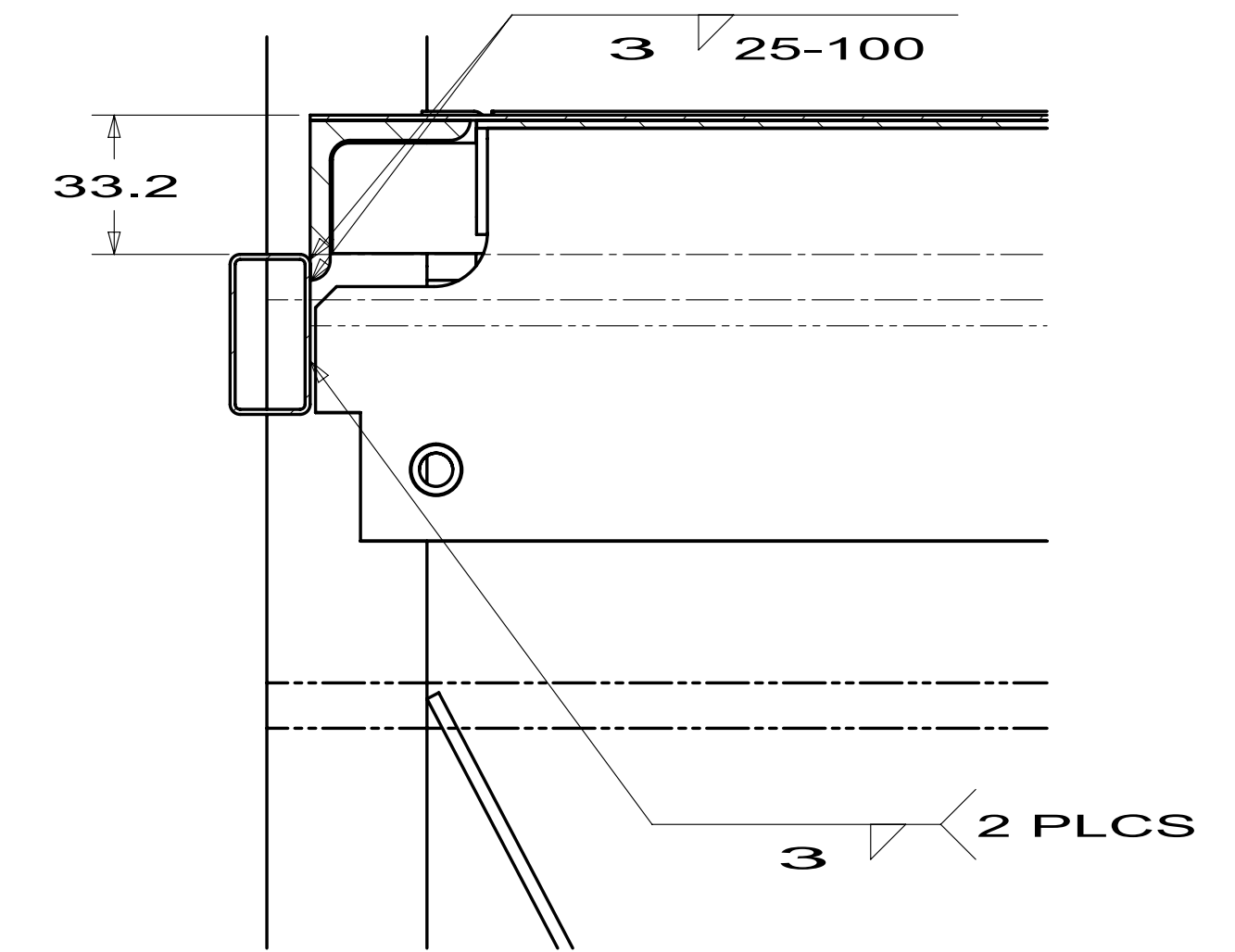
SECTION FC-FC
