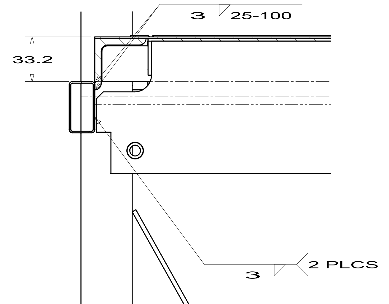
SECTION FC-FC
