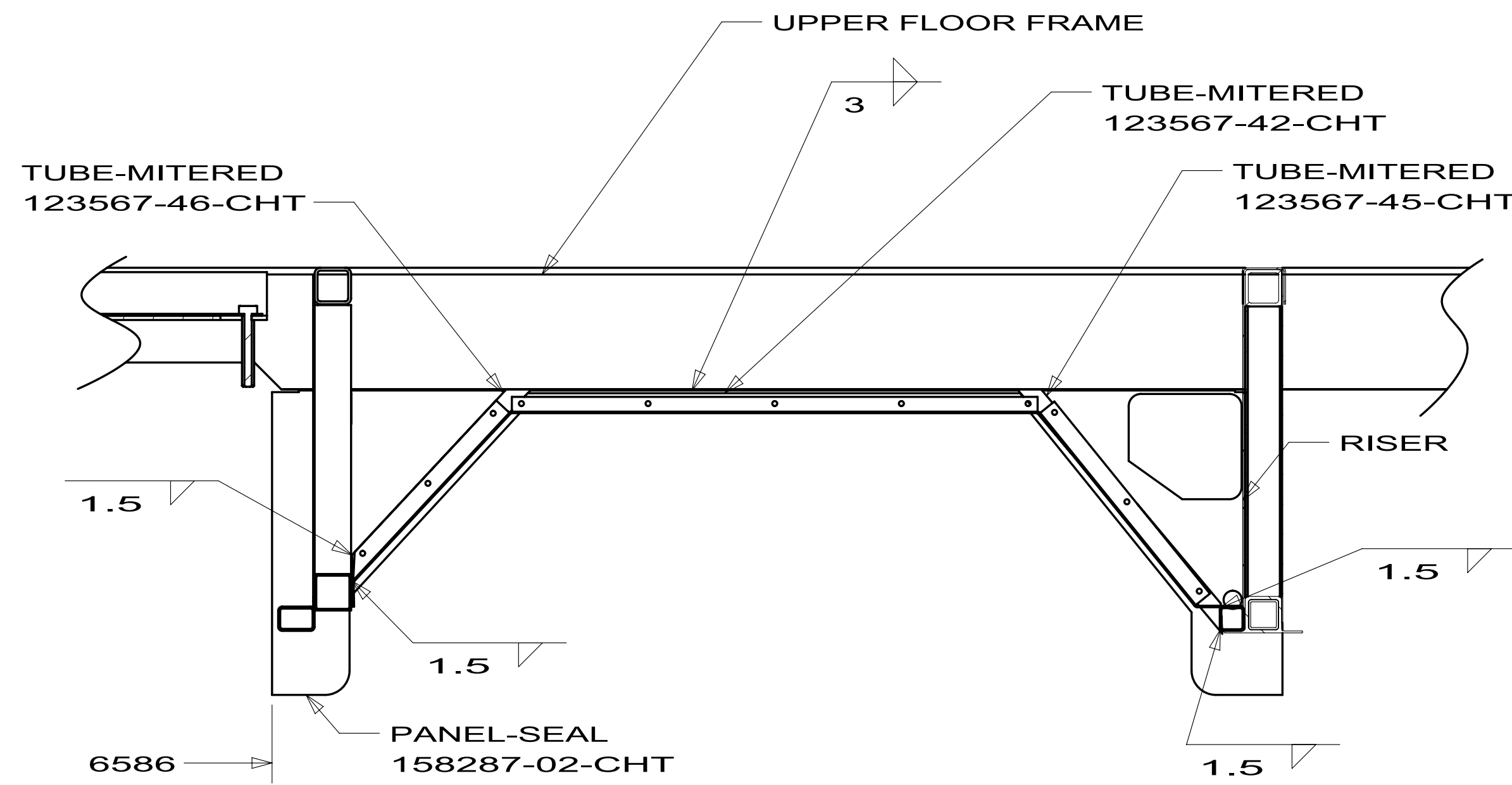
SECTION EA-EA
