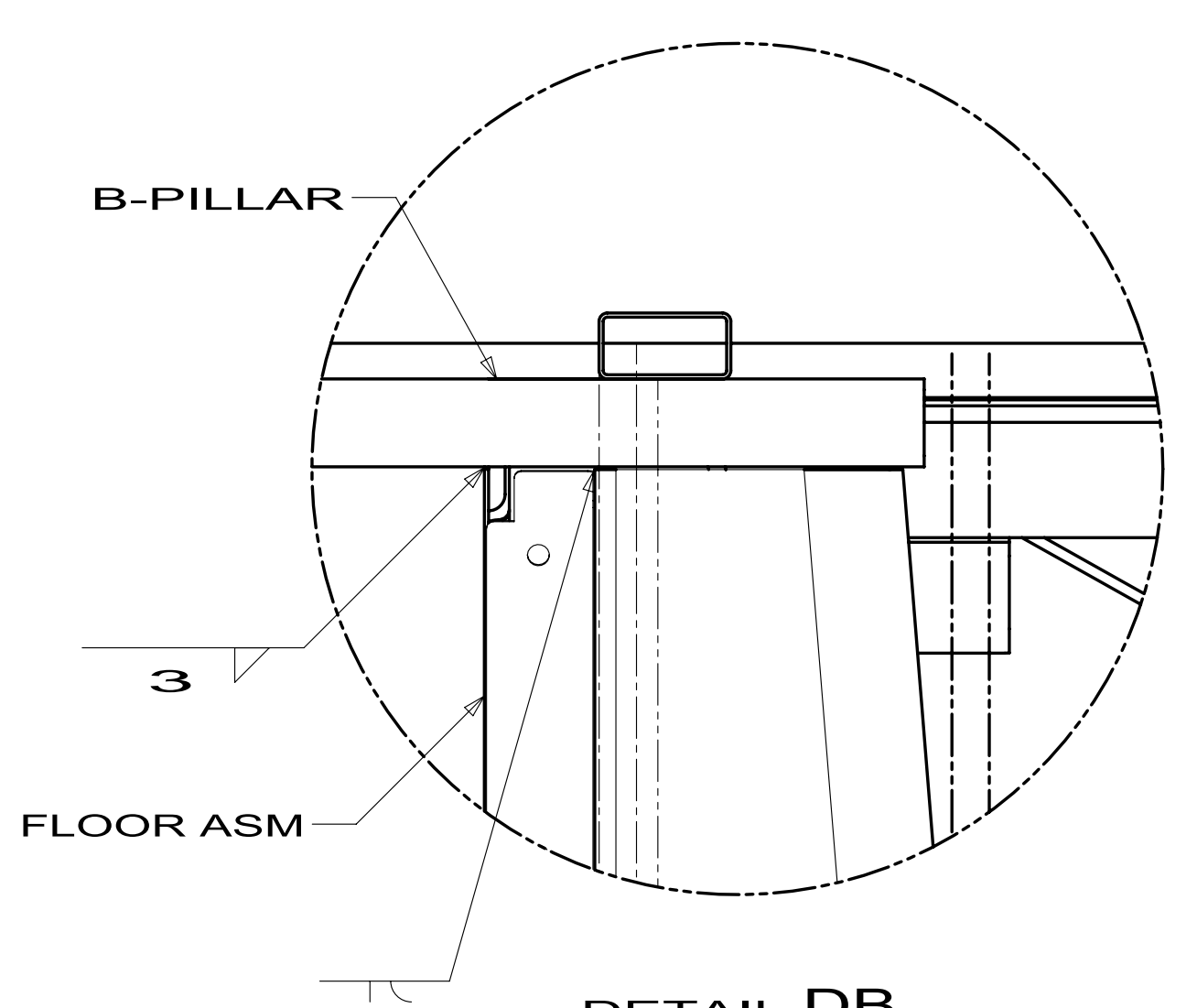
DETAIL DB
