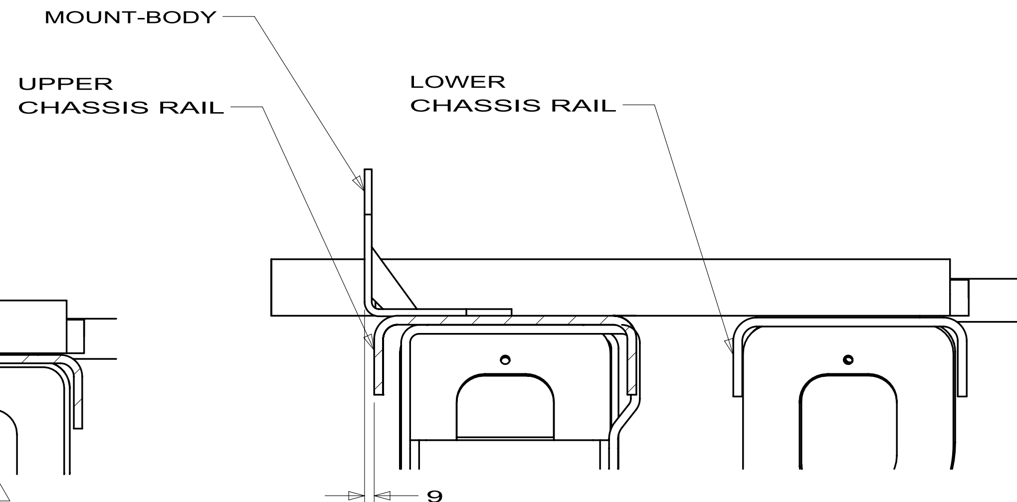
SECTION BG-BG (SHOWN) SECTION BH-BH (OPPOSITE)
