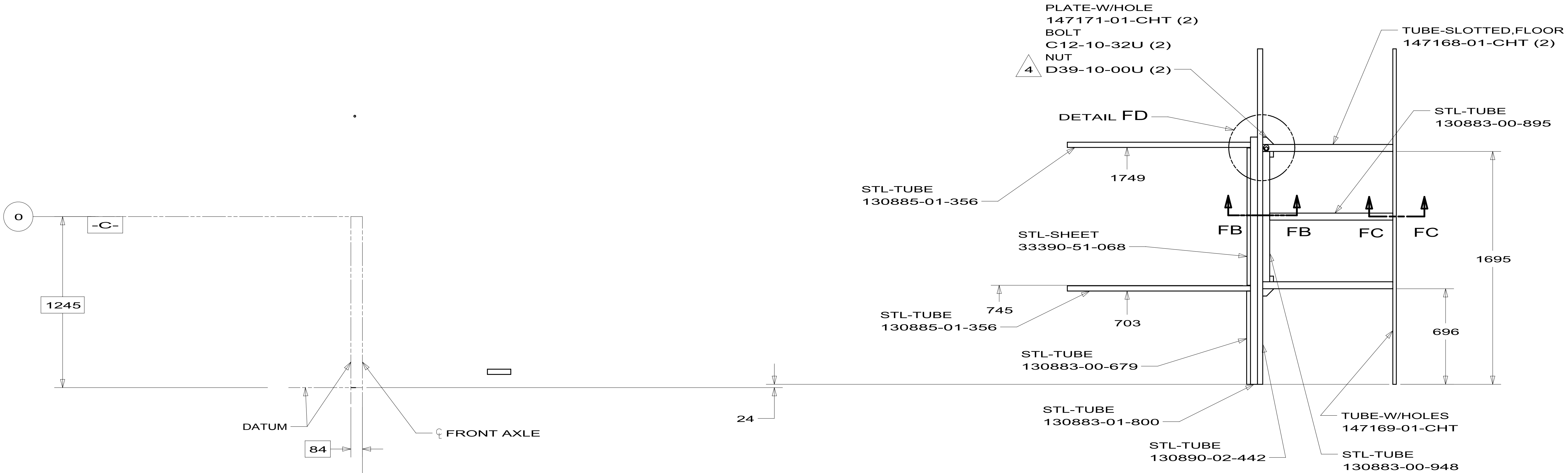
VIEW FA-FA FLOOR FRAME ASM-LOWER 169207-14
