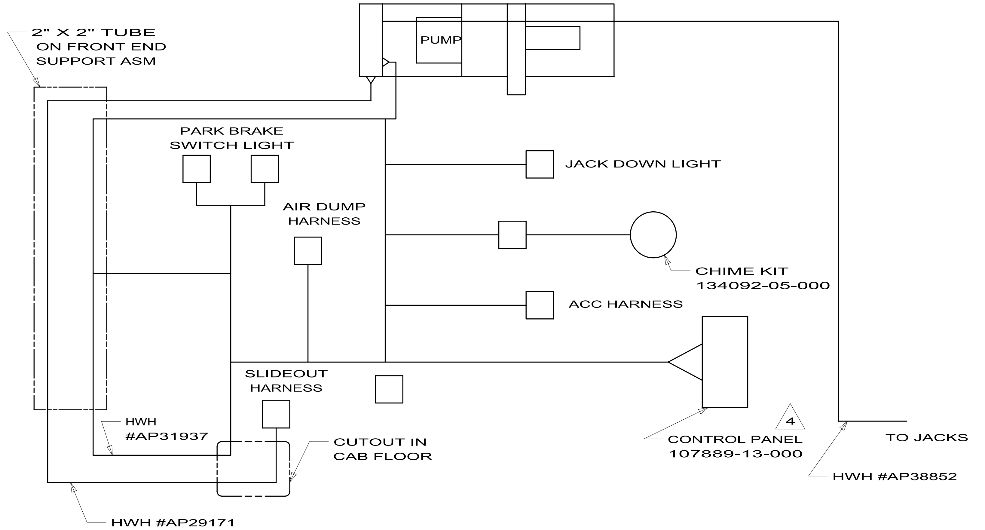
WIRING DIAGRAM
