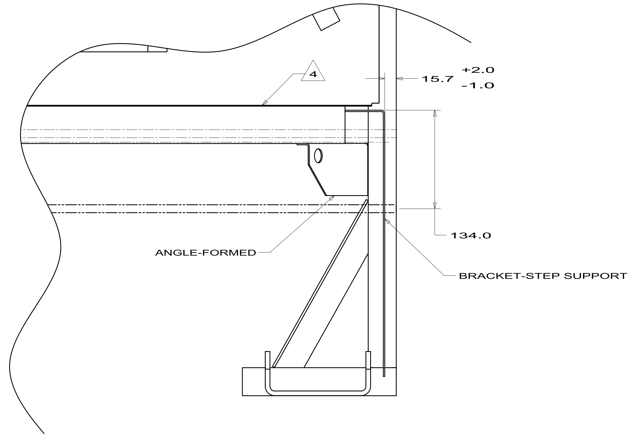
SECTION LD-LD
