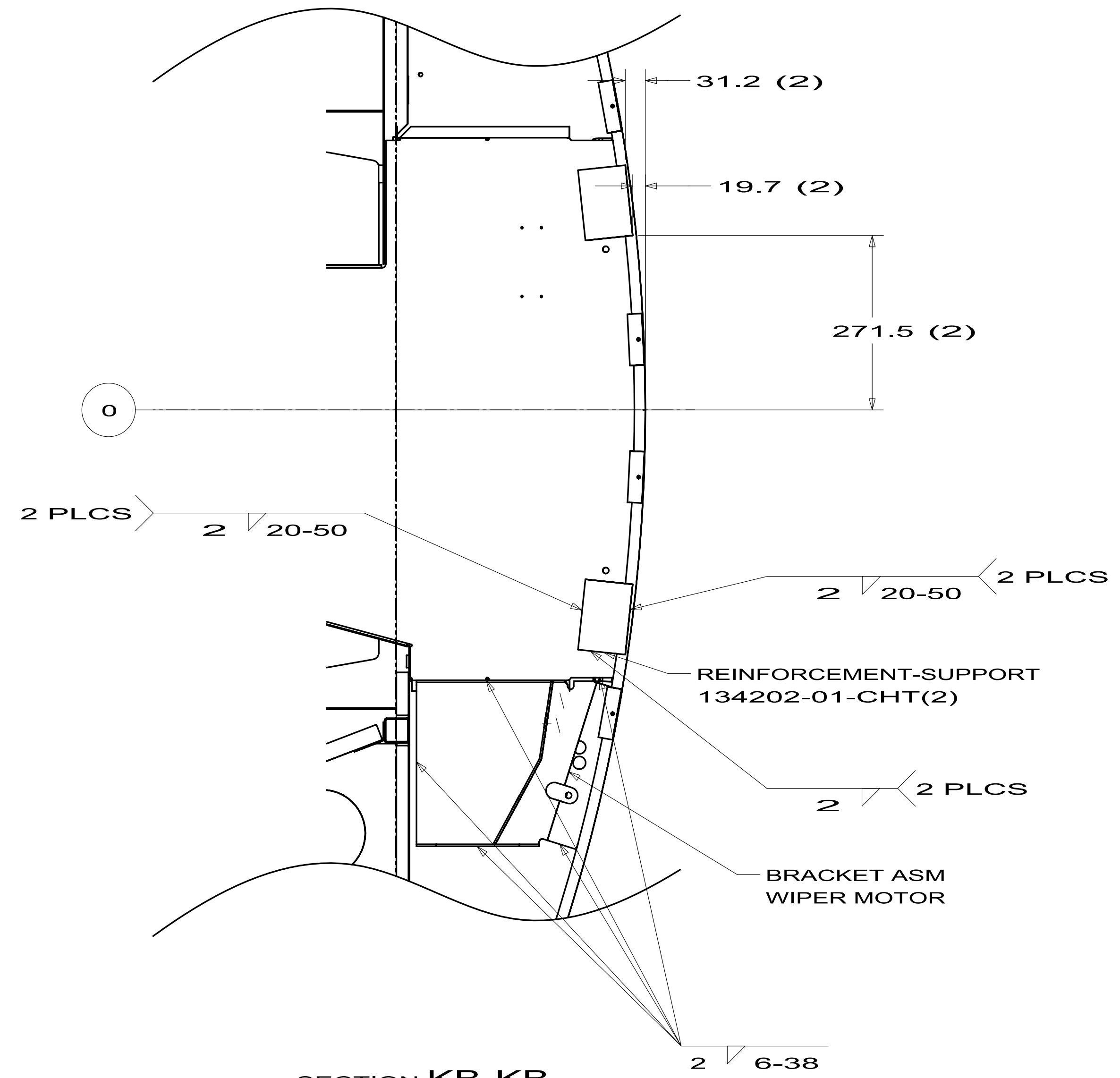
SECTION KB-KB
