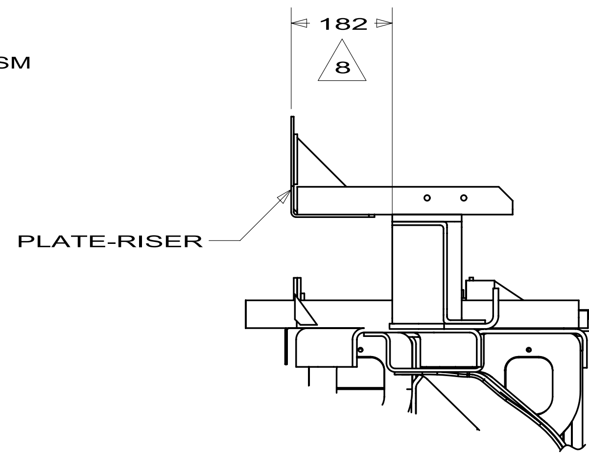
VIEW BB-BB
