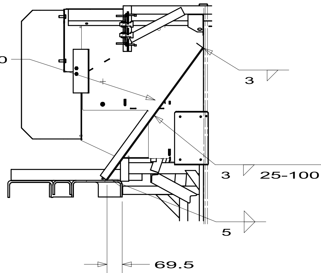
SECTION BB-BB
