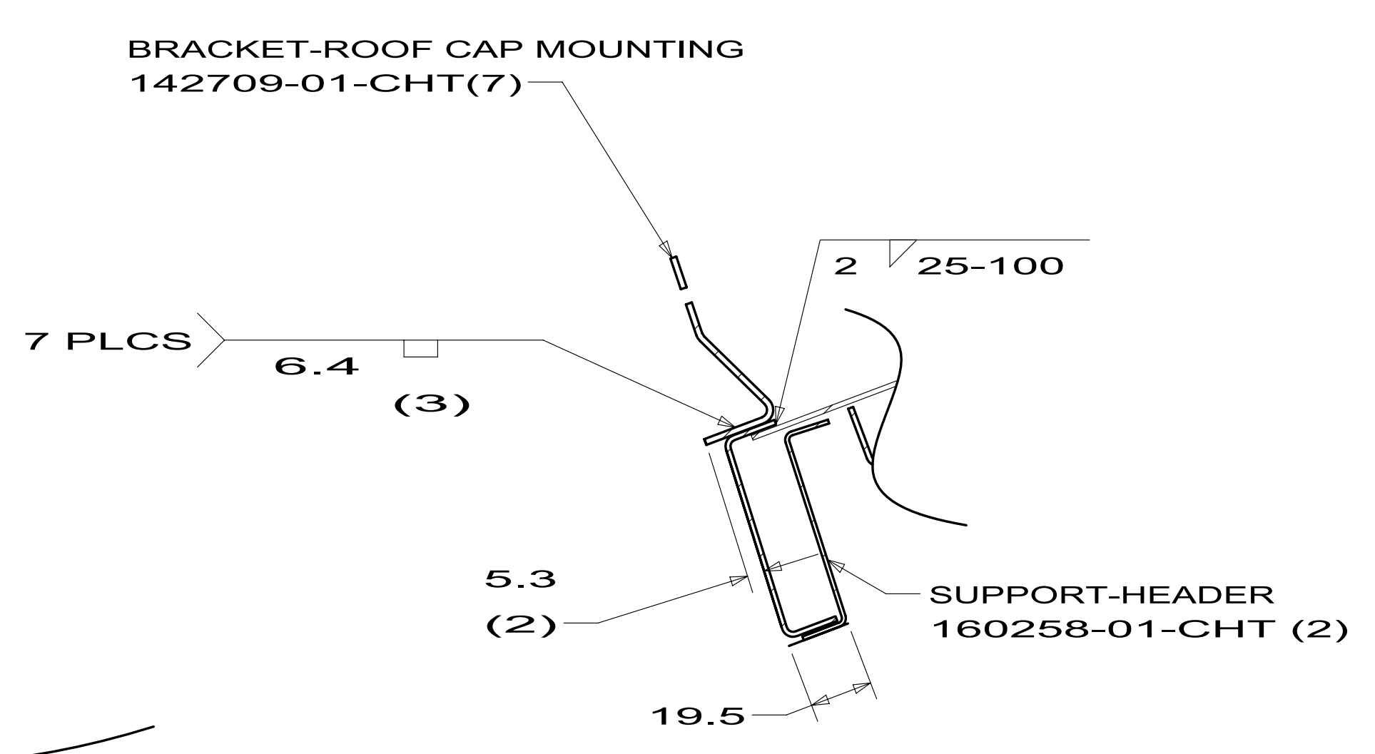
SECTION DD-DD
