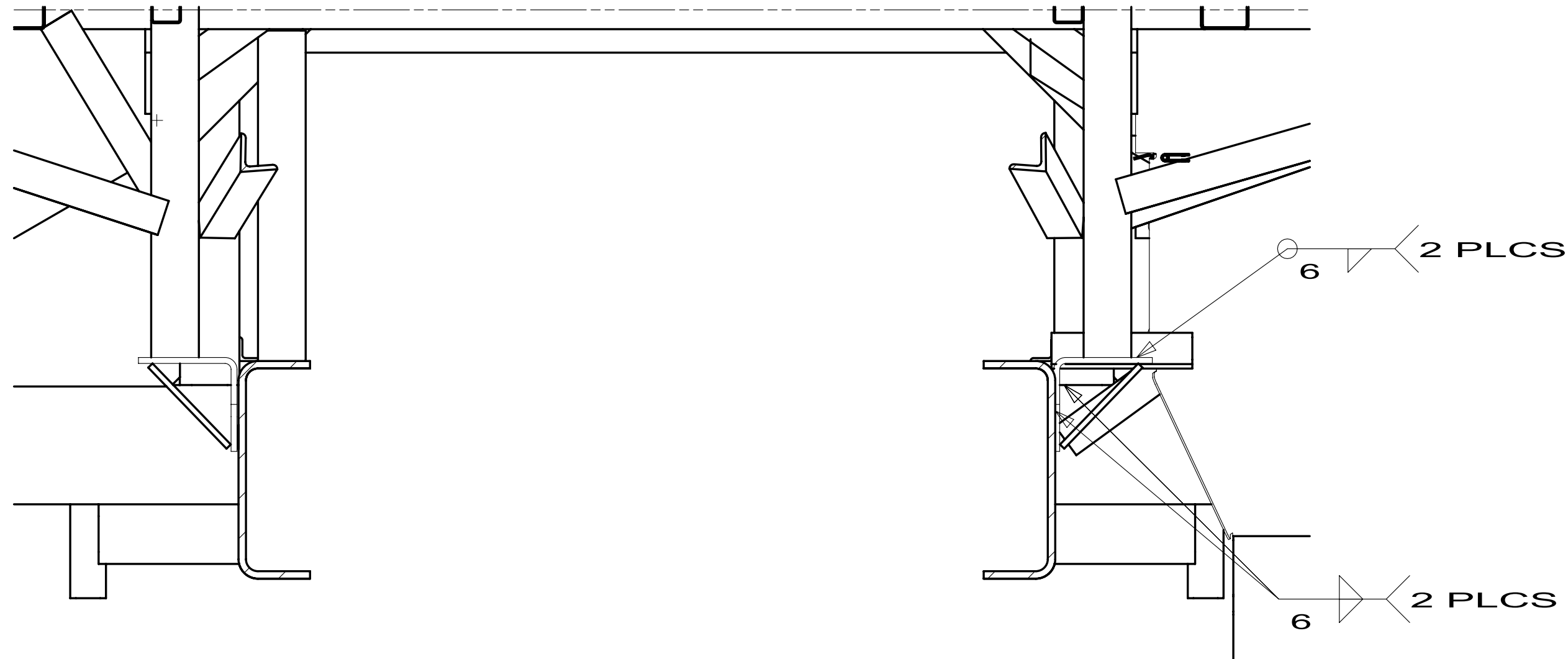
SECTION CB-CB
