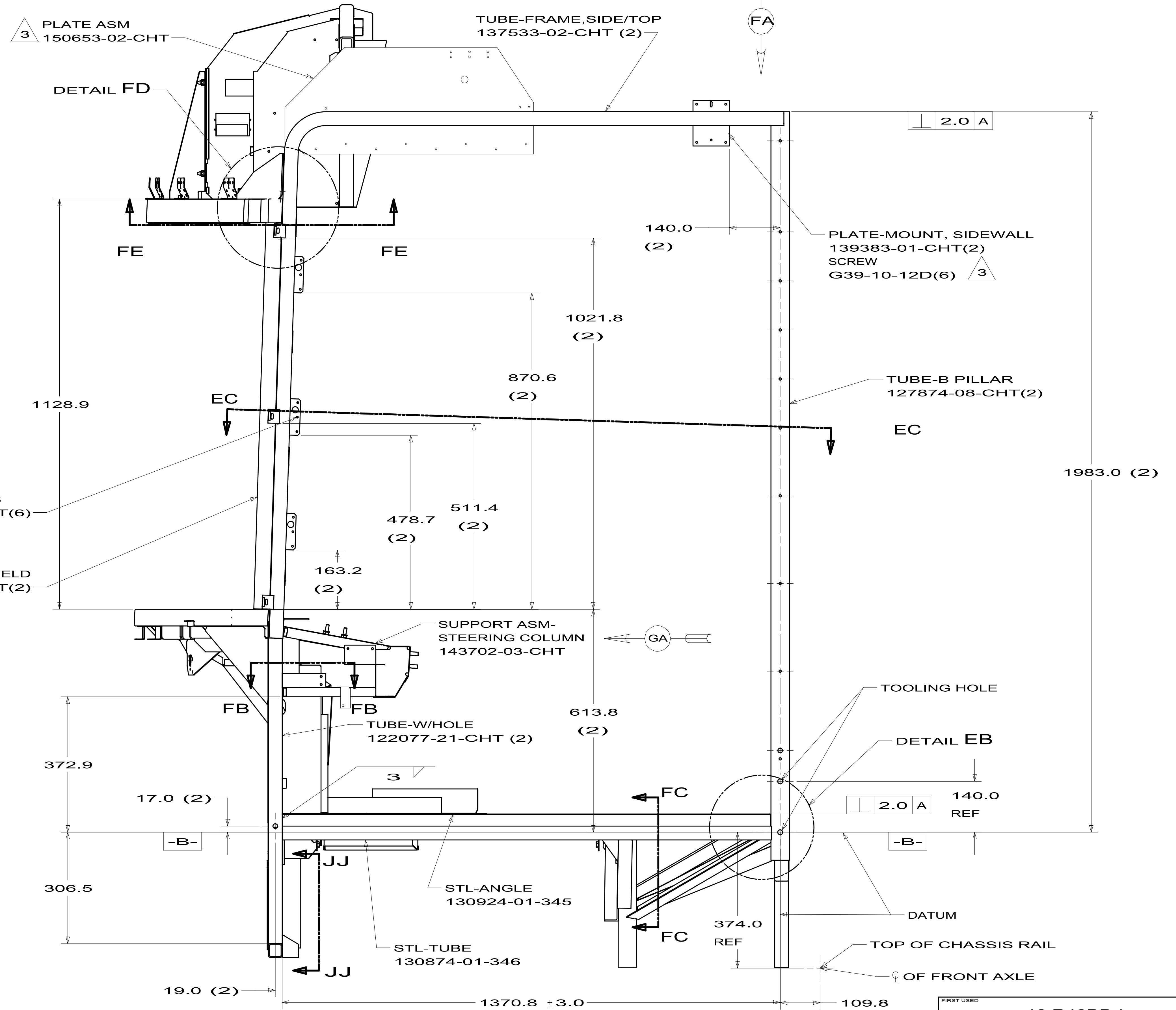
VIEW EA
