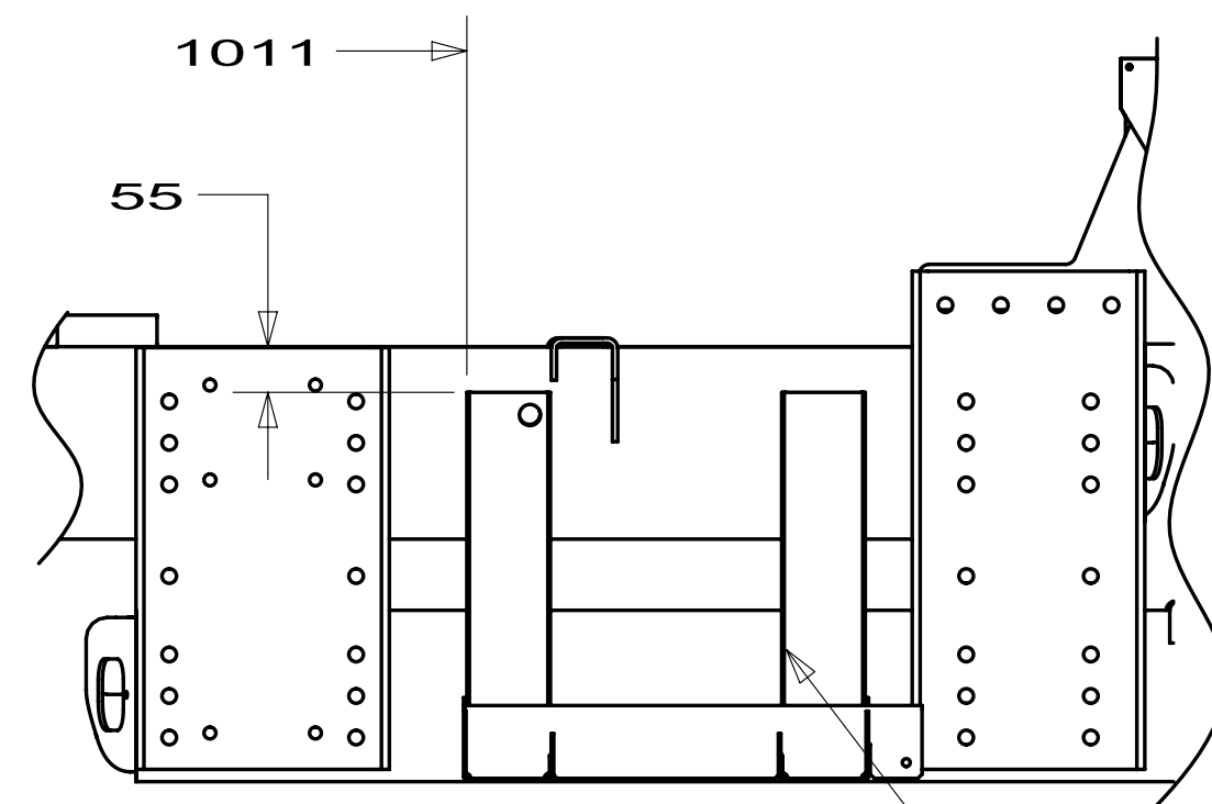
HANGER ASM-LP TANK
