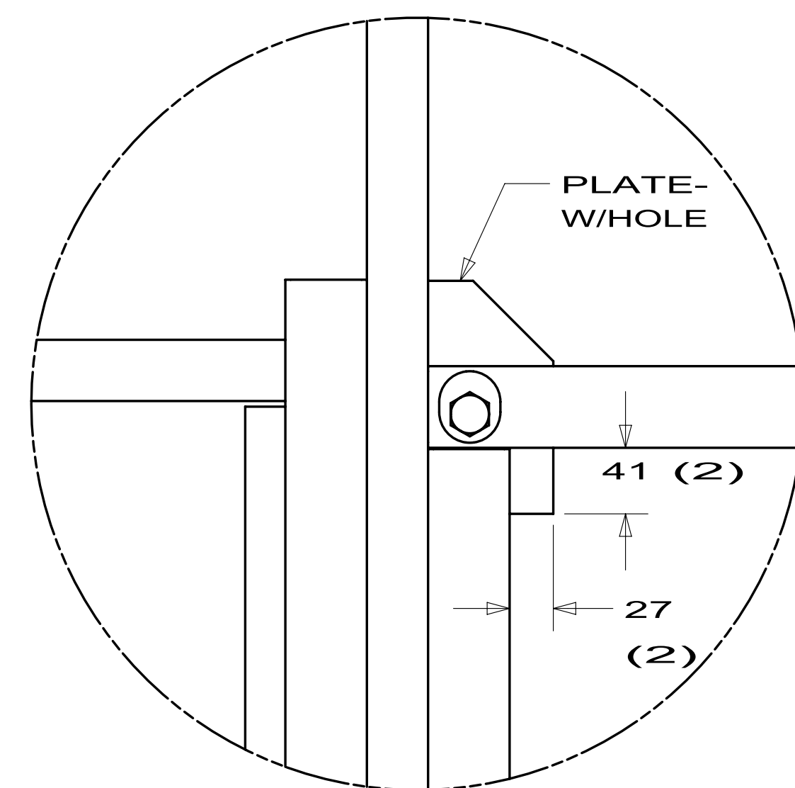
DETAIL FD
