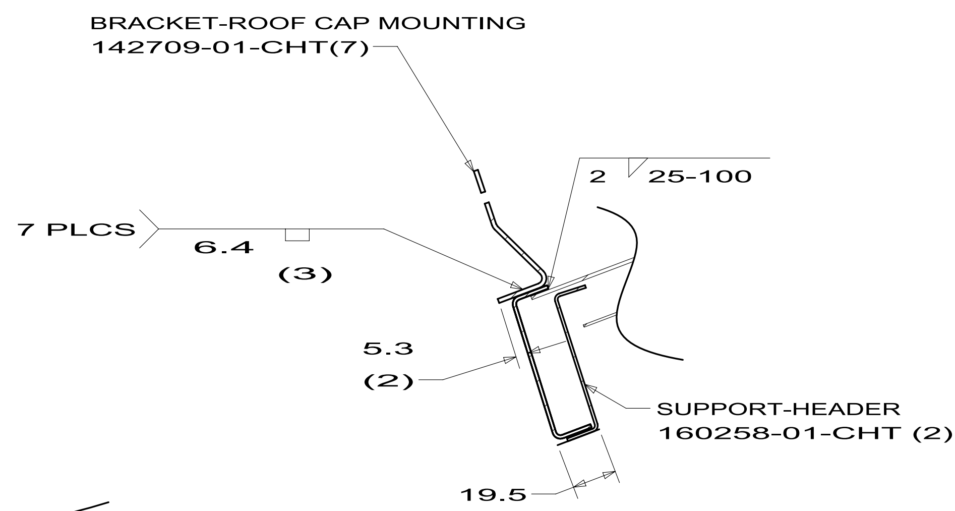
SECTION DD-DD
