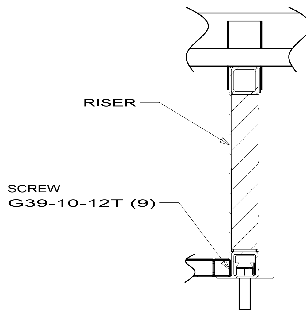
SECTION FC-FC
