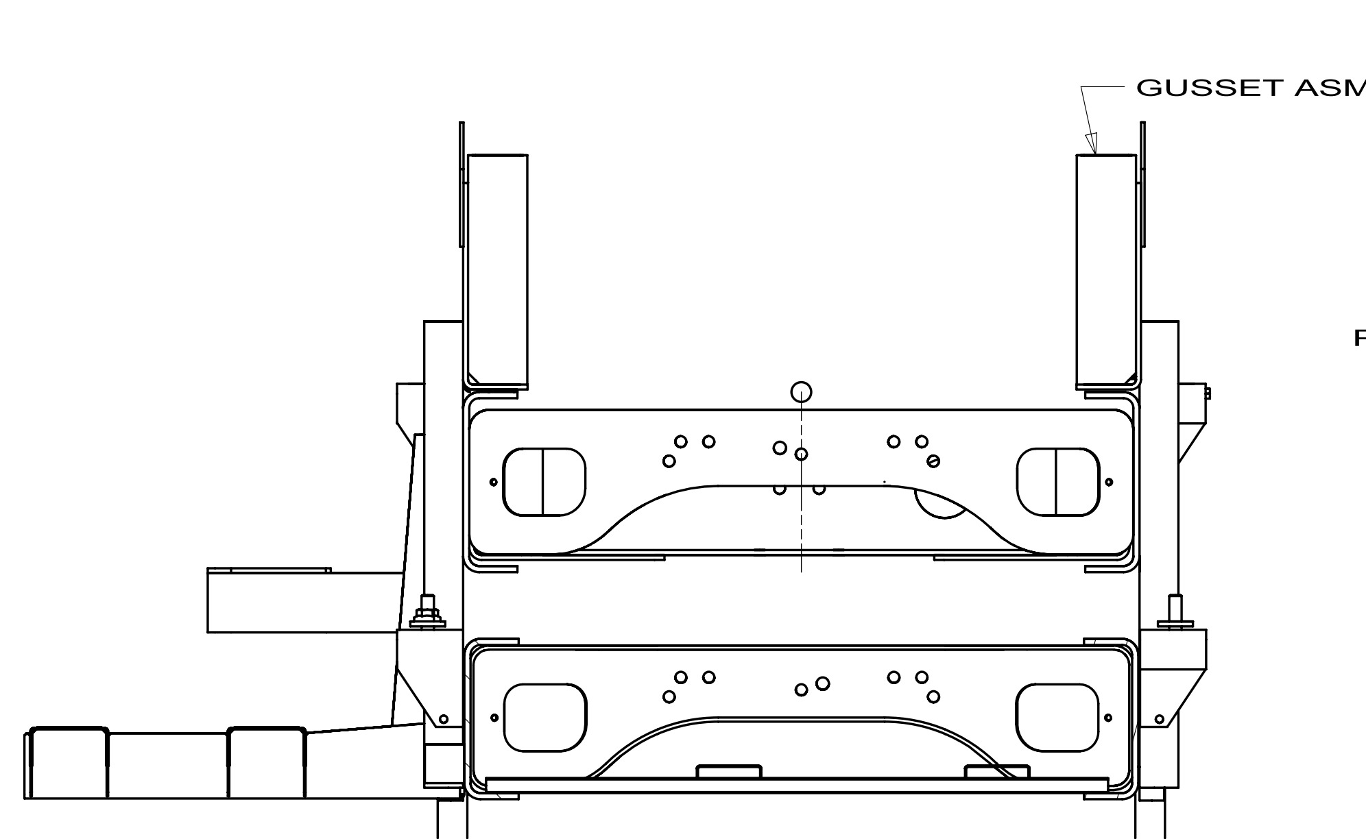
SECTION BA-BA
