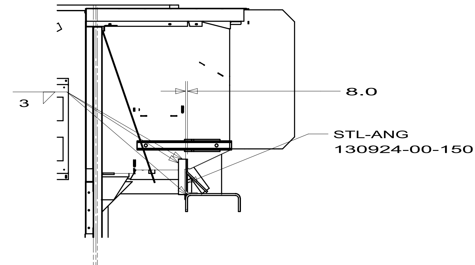
SECTION BC-BC
