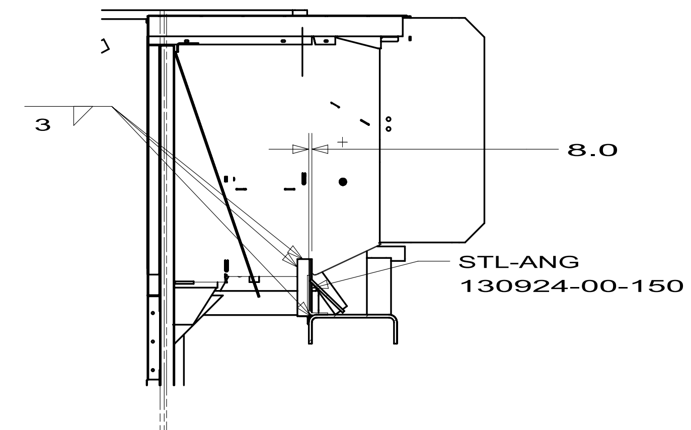
SECTION BC-BC
