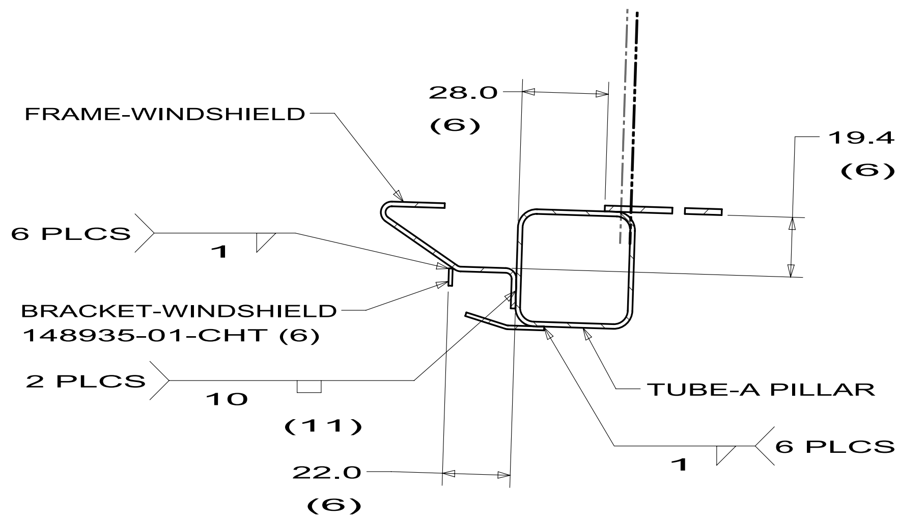
SECTION EC-EC
