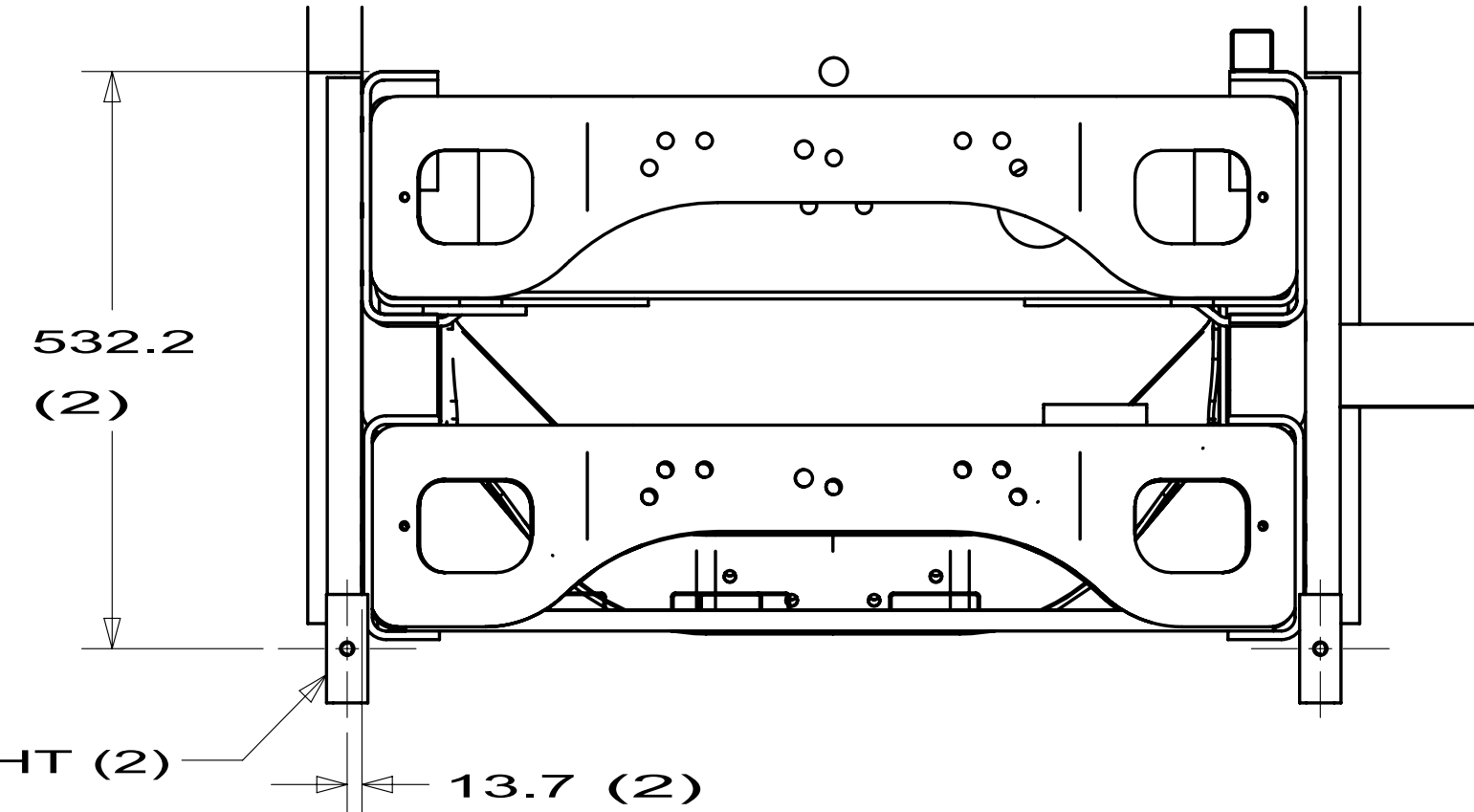
SECTION BM-BM
