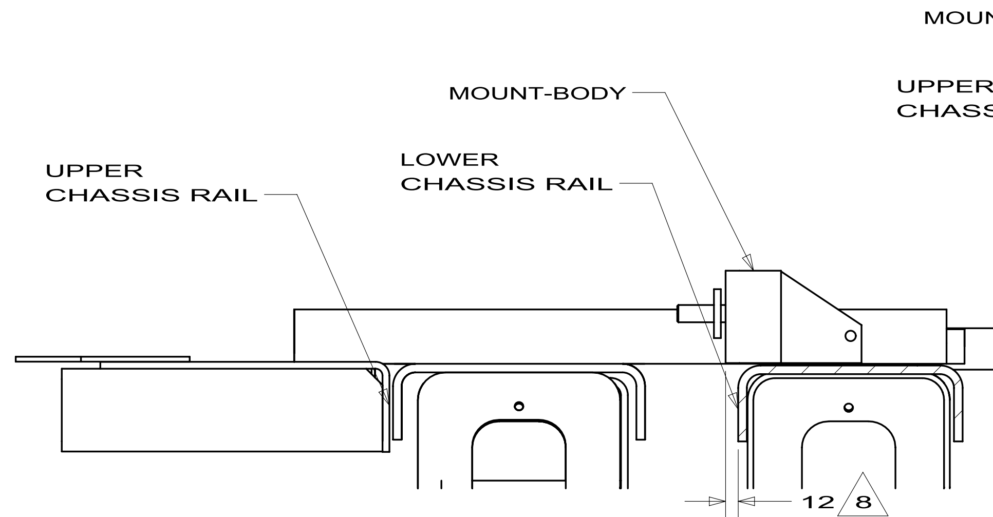
SECTION BA-BA
