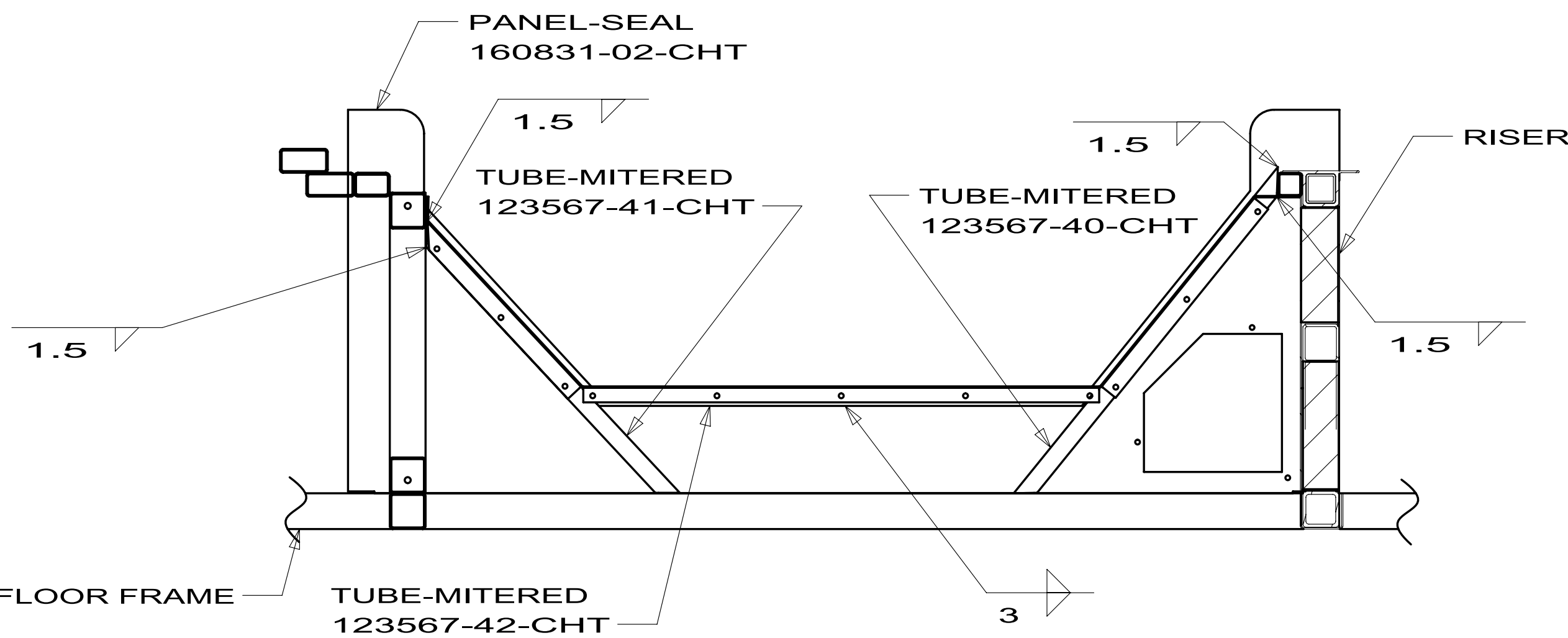
SECTION EB-EB
