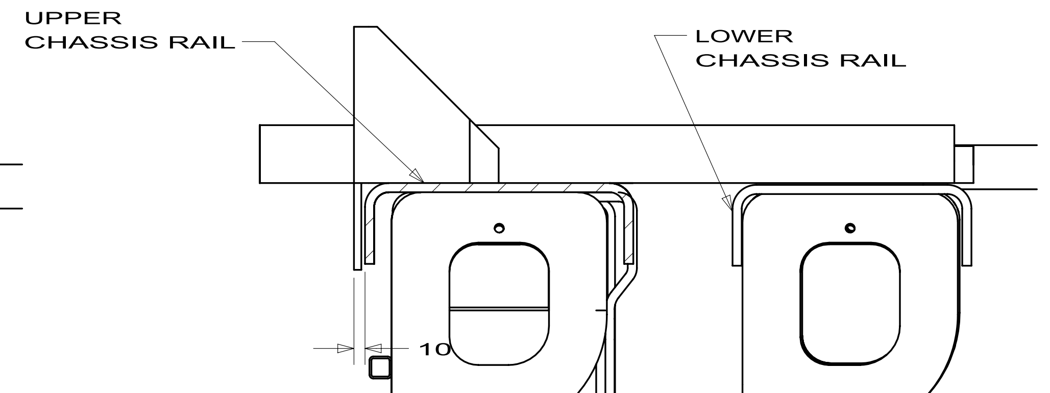
SECTION BJ-BJ (SHOWN) SECTION BK-BK (OPPOSITE)
