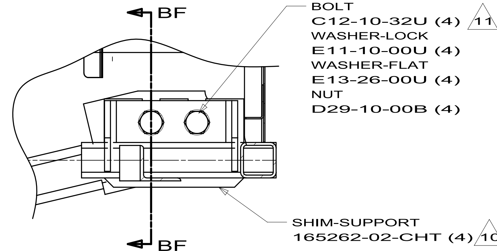
SECTION BE-BE
