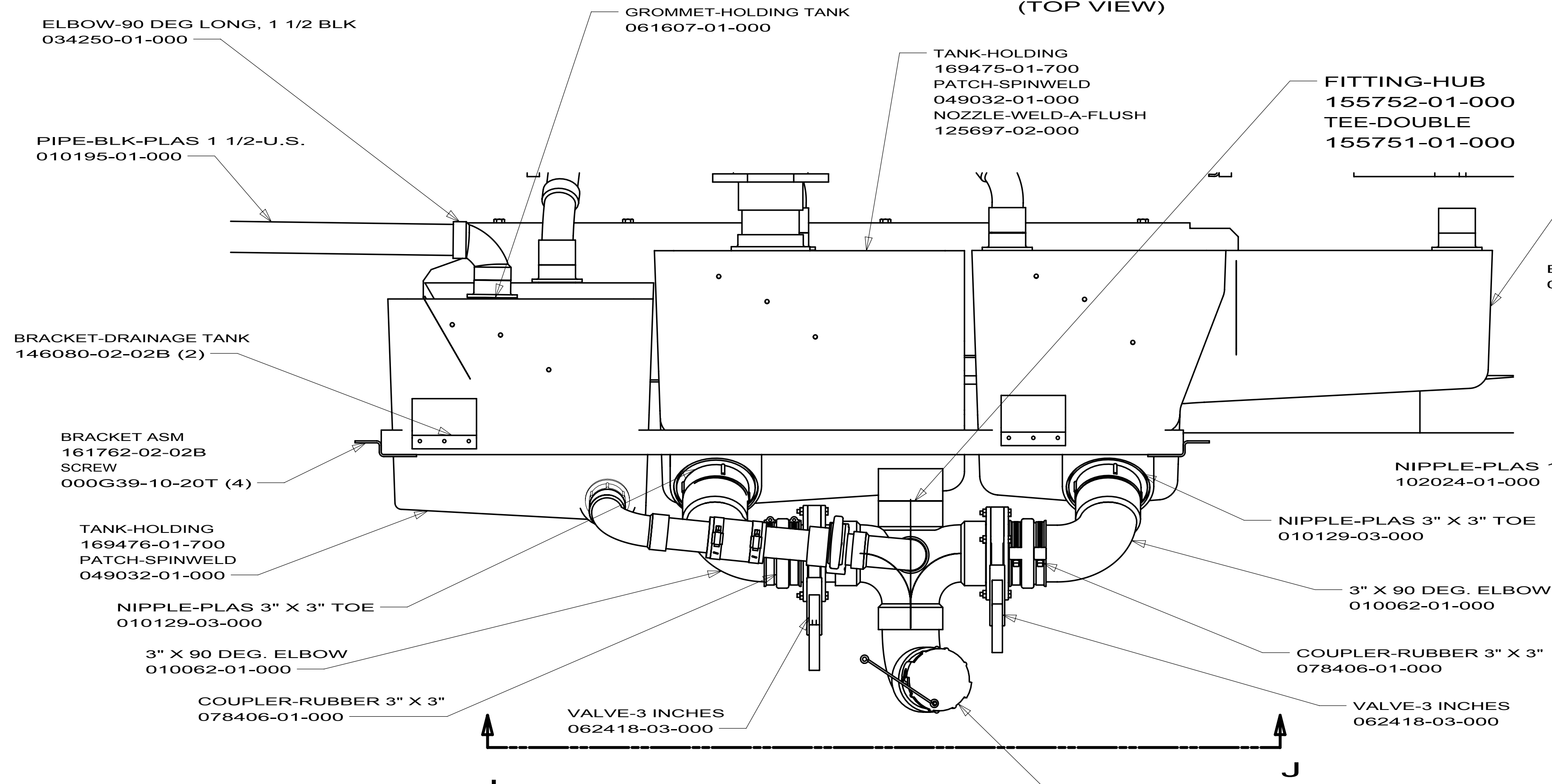
VIEW E (TOP VIEW)
