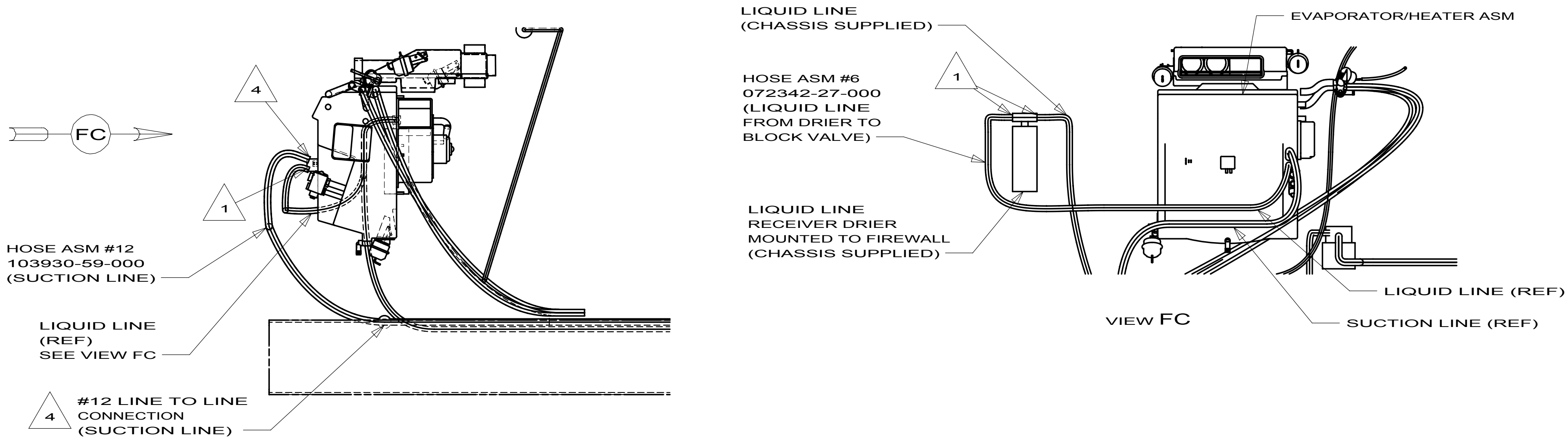
VIEW FA-FA
