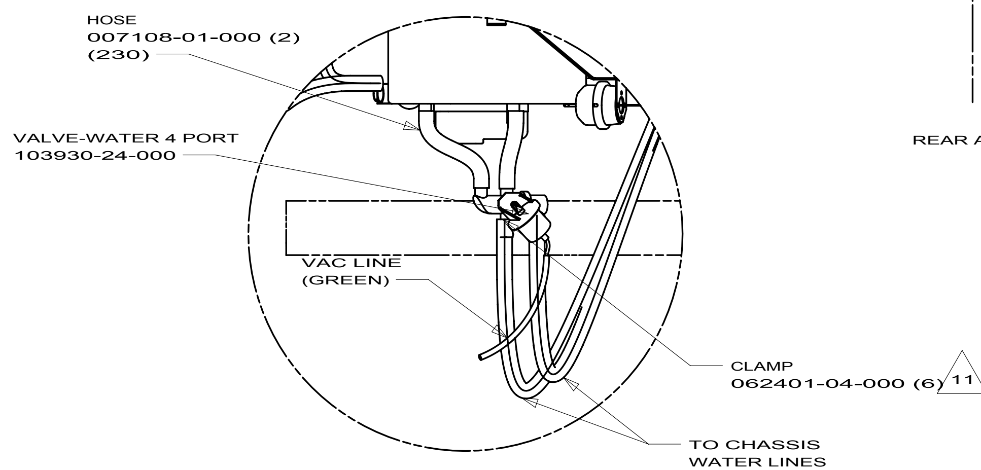
DETAIL FB
