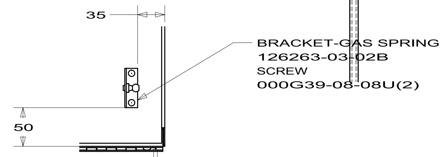
SECTION BE-BE (DOOR JAMB REMOVED FOR CLARITY)
