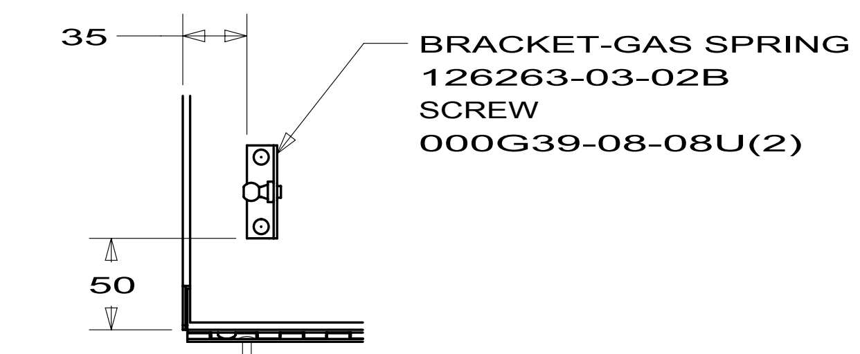
SECTION BF-BF (DOOR JAMB REMOVED FOR CLARITY)
