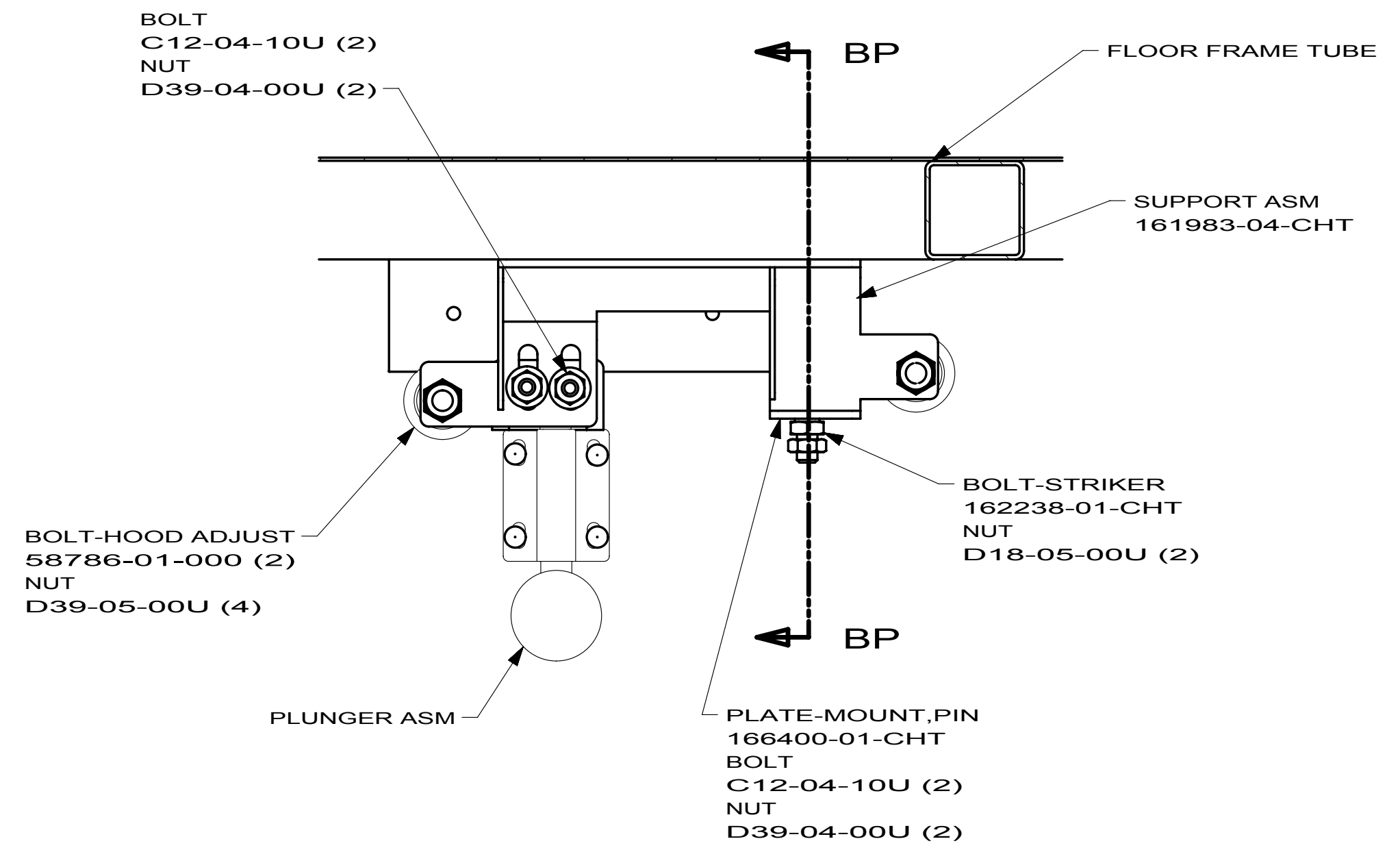
SECTION BS-BS (ROTATED)
