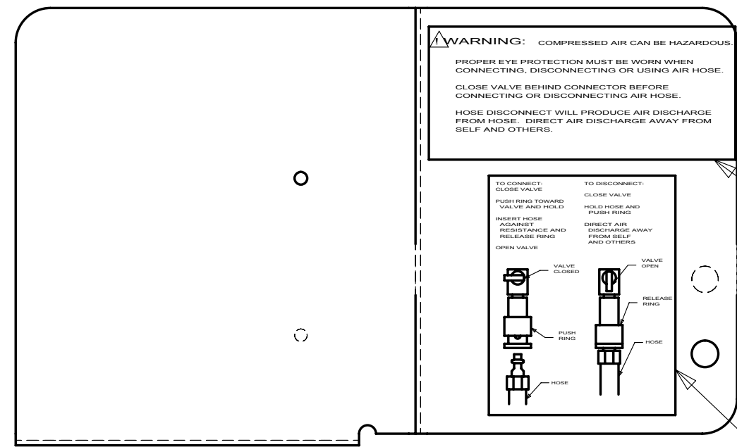
AIR ACCESS PANEL
