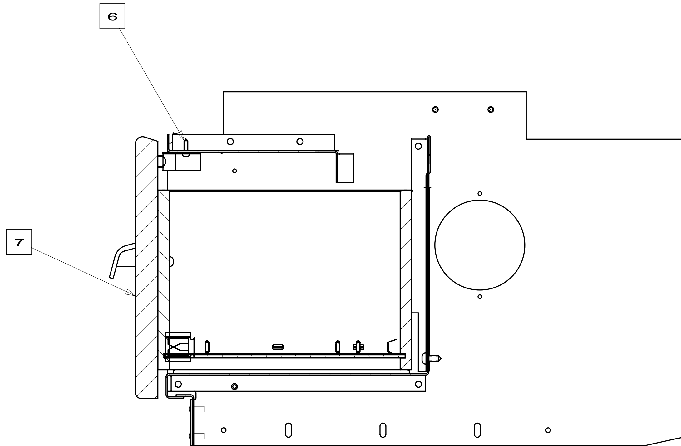
SECTION F-F
