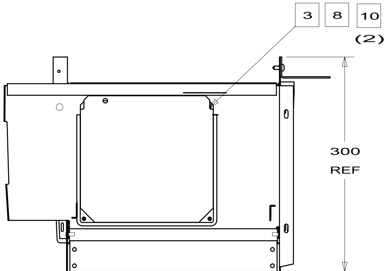
VIEW E (BACK OF FACE PANELS)
