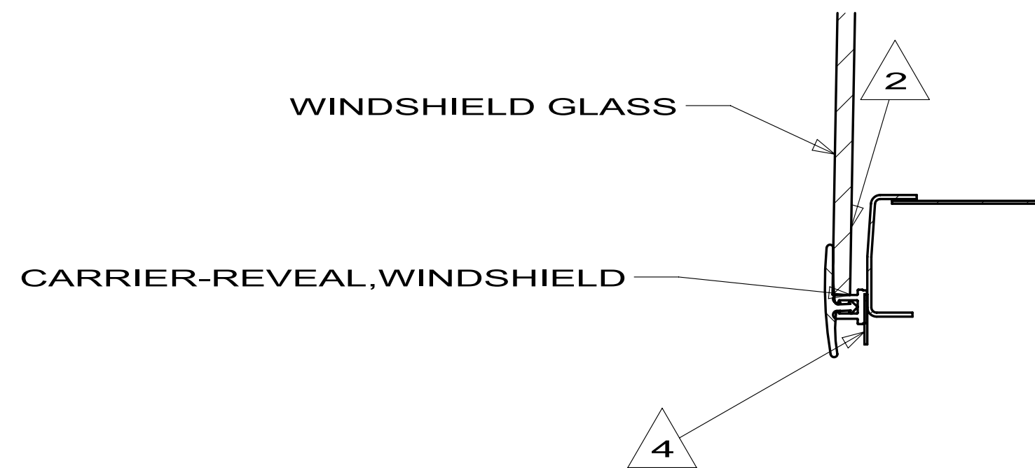
SECTION DD-DD
