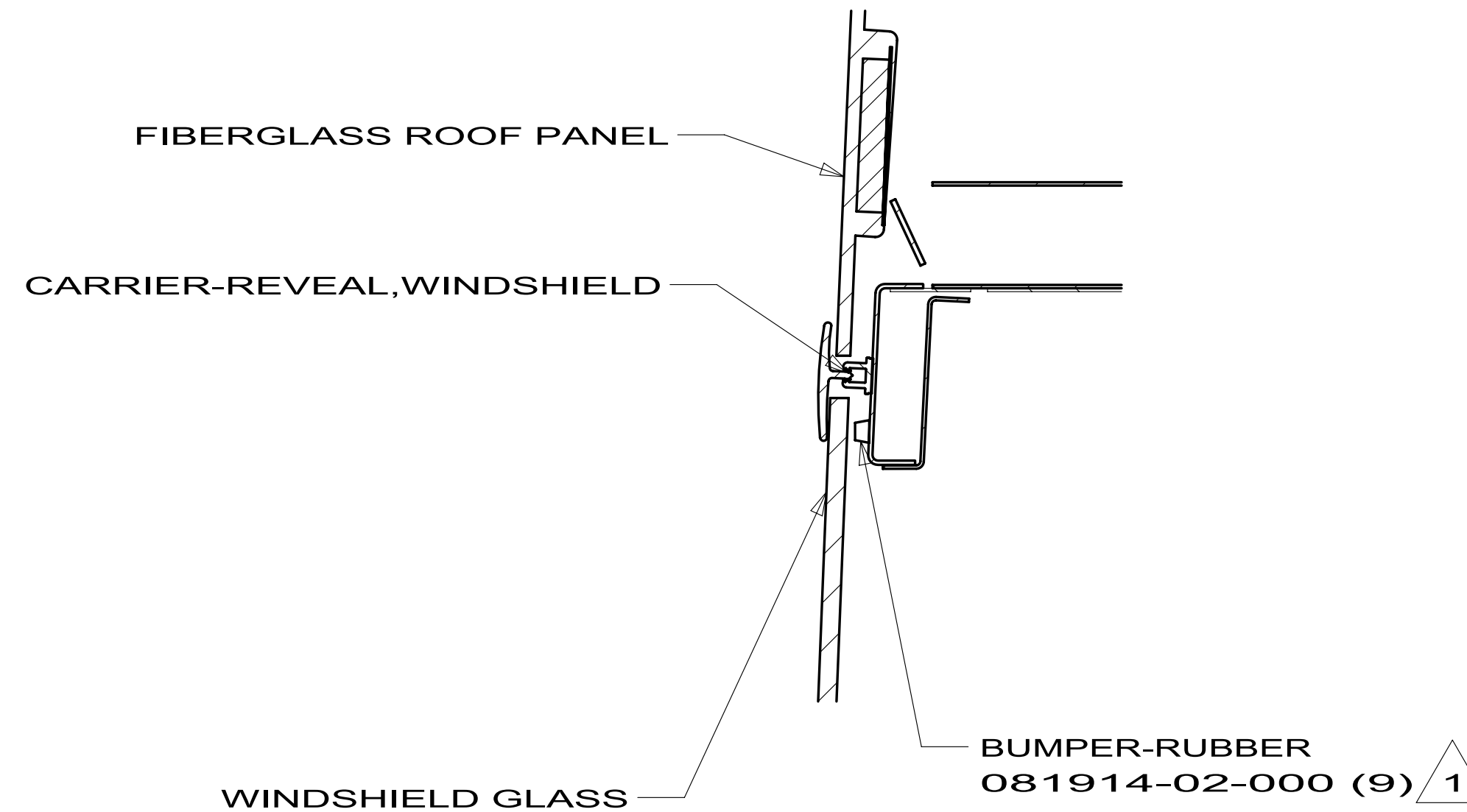
SECTION DE-DE
