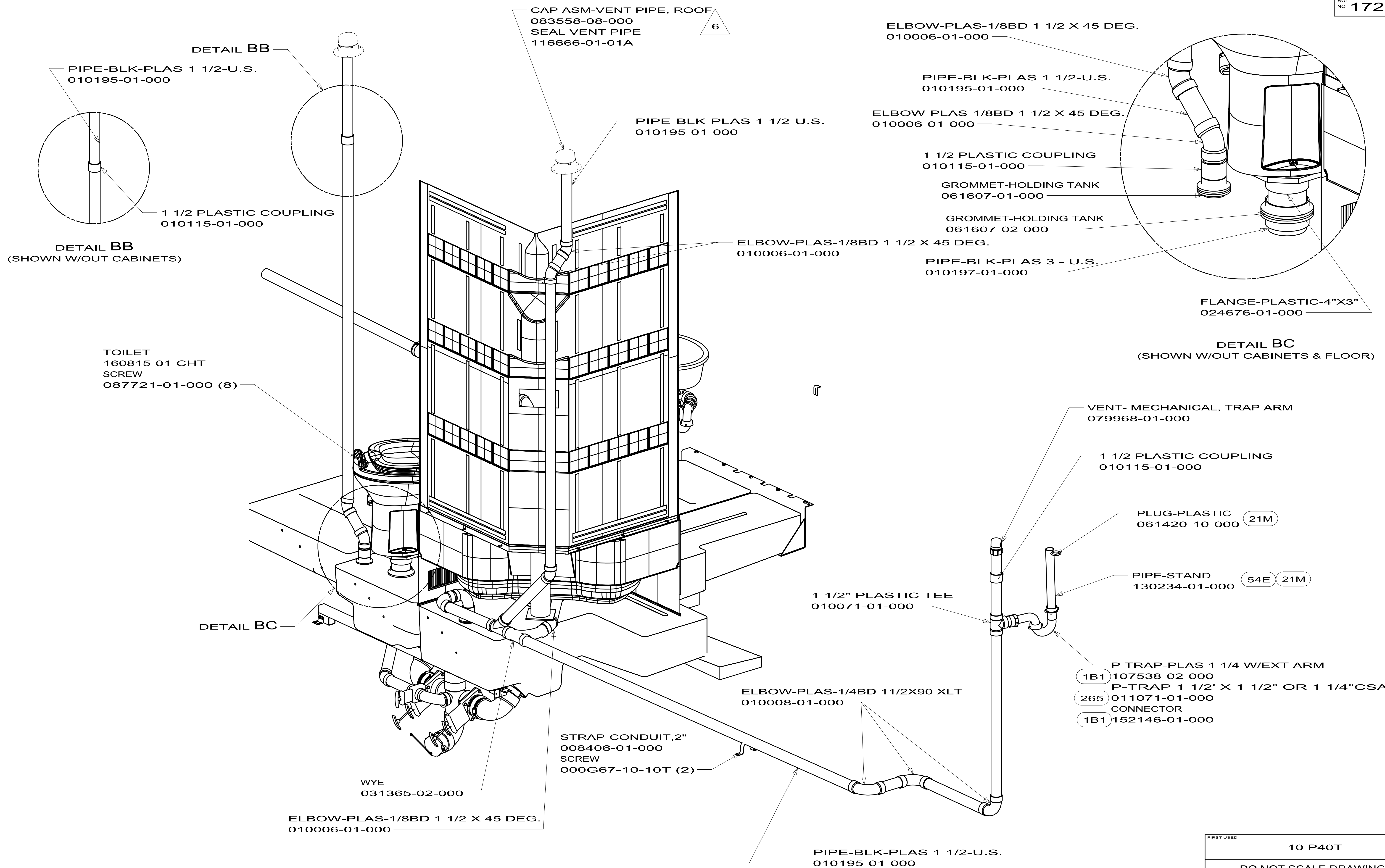
VIEW BA
