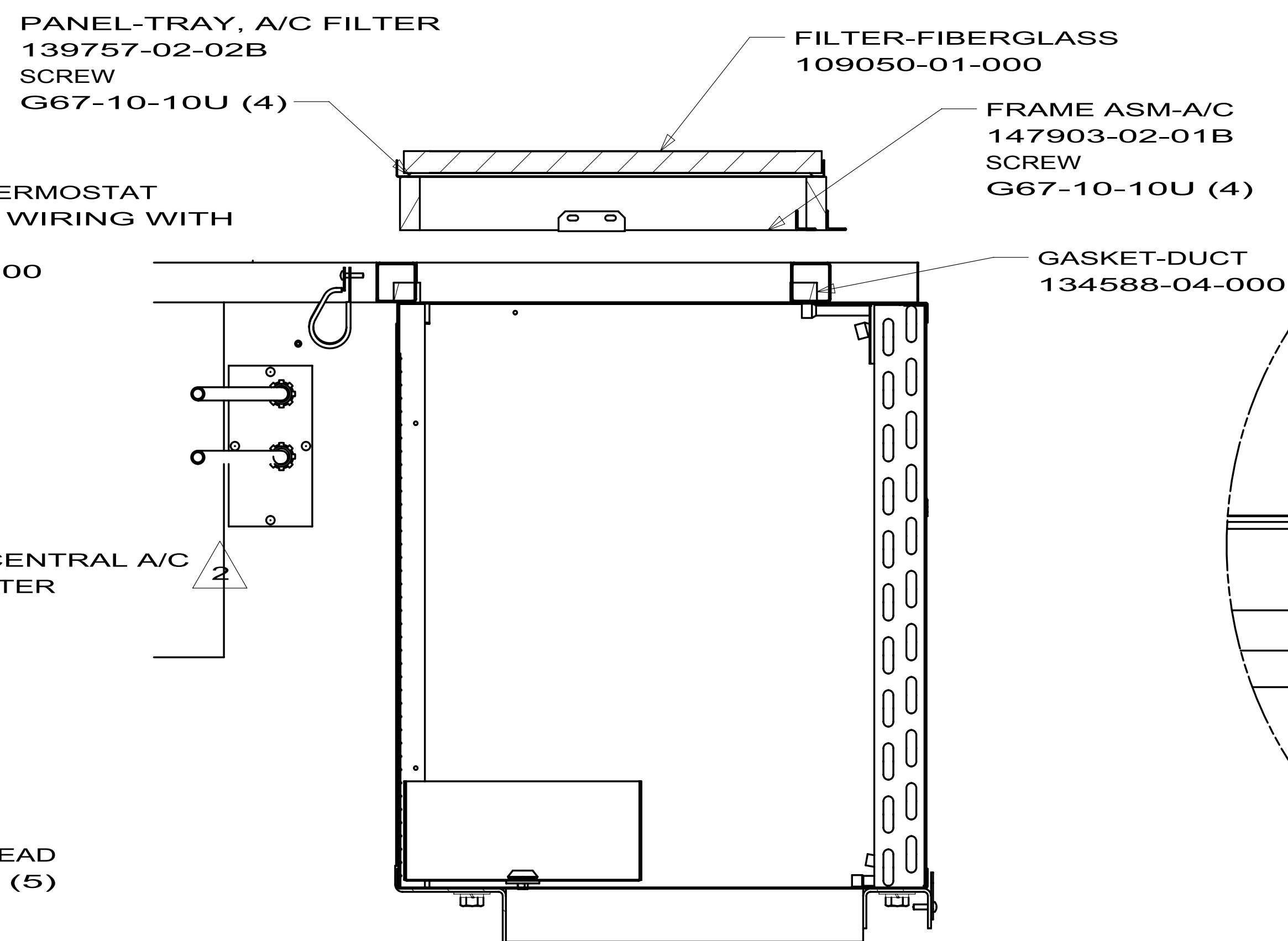
SECTION B-B
