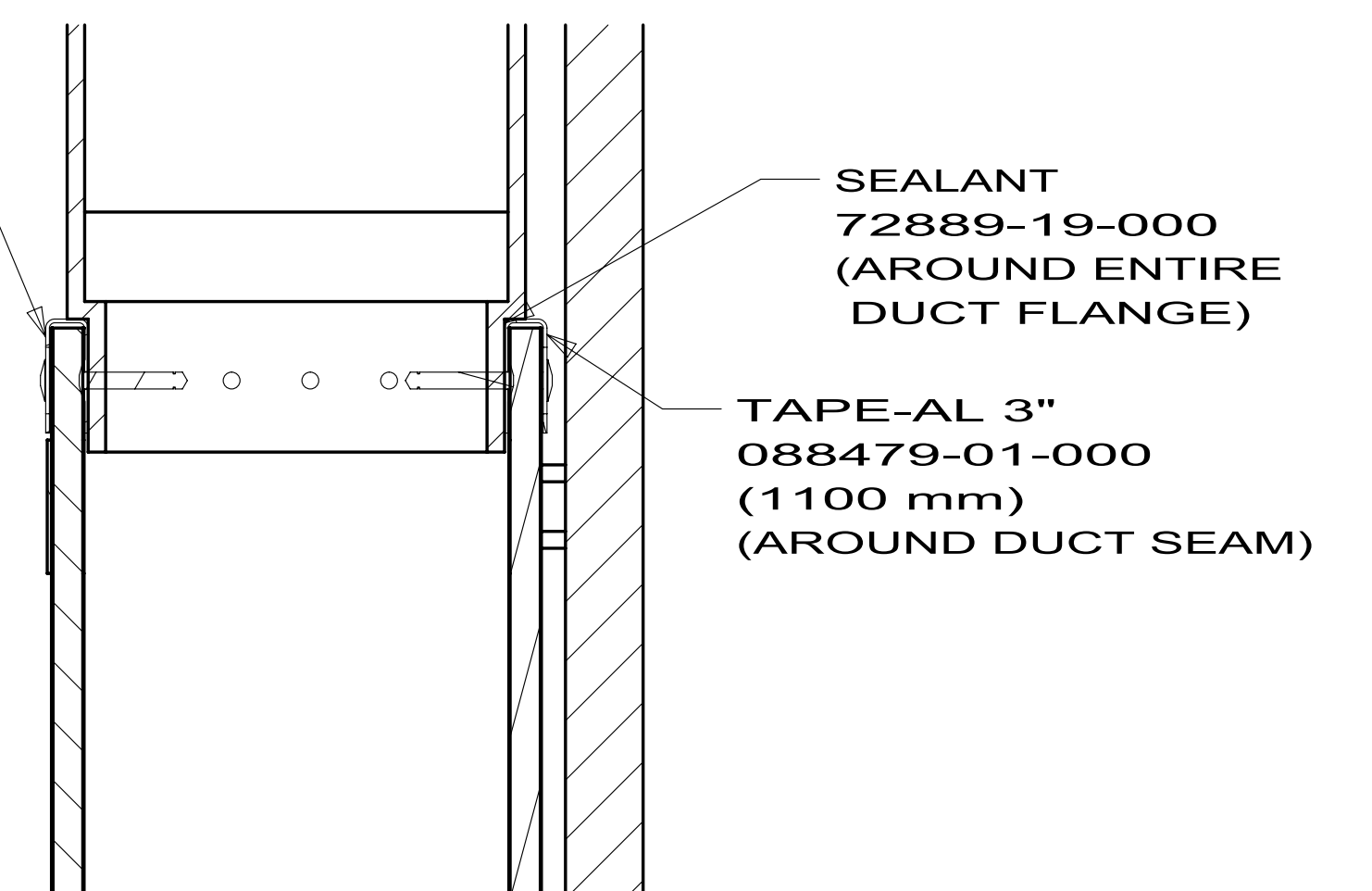
SECTION F-F
