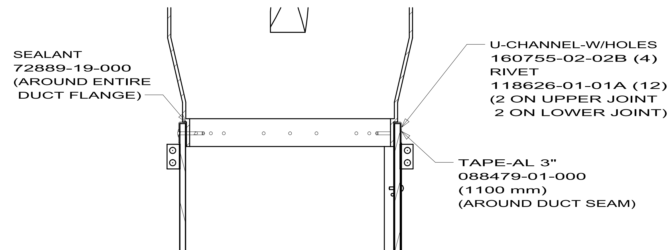
SECTION E-E
