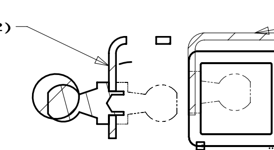
SECTION BN-BN
