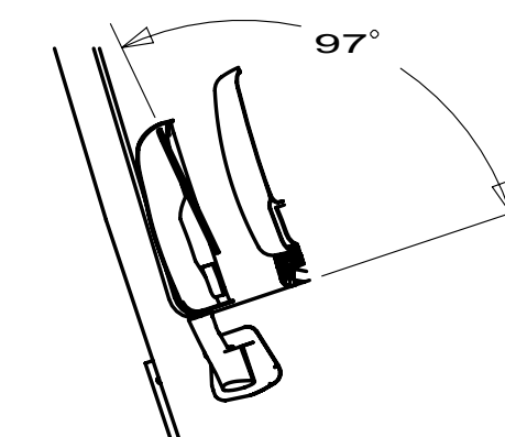
SECTION DB-DB
