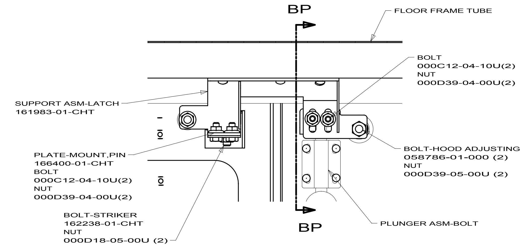
SECTION BM-BM
