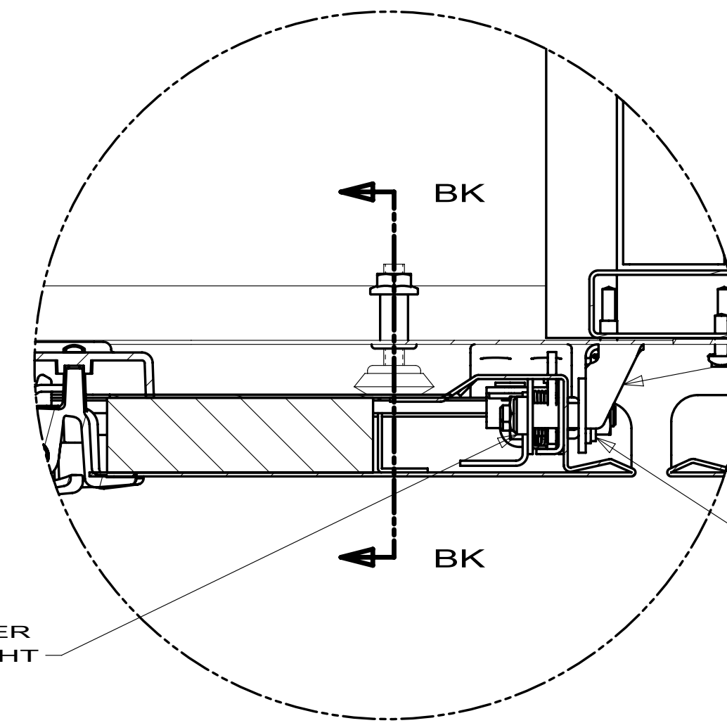
DETAIL BJ
