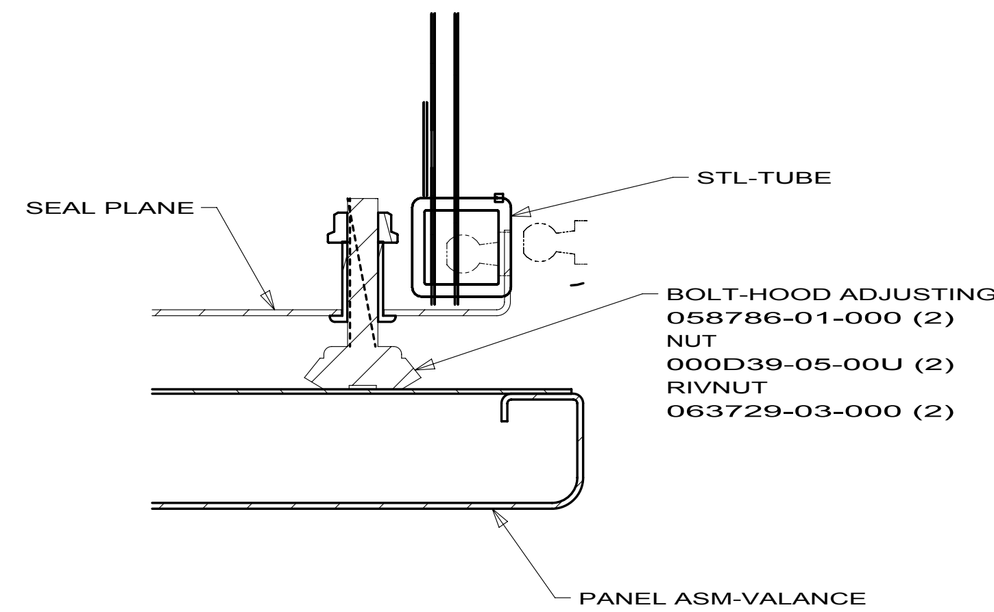
SECTION BK-BK
