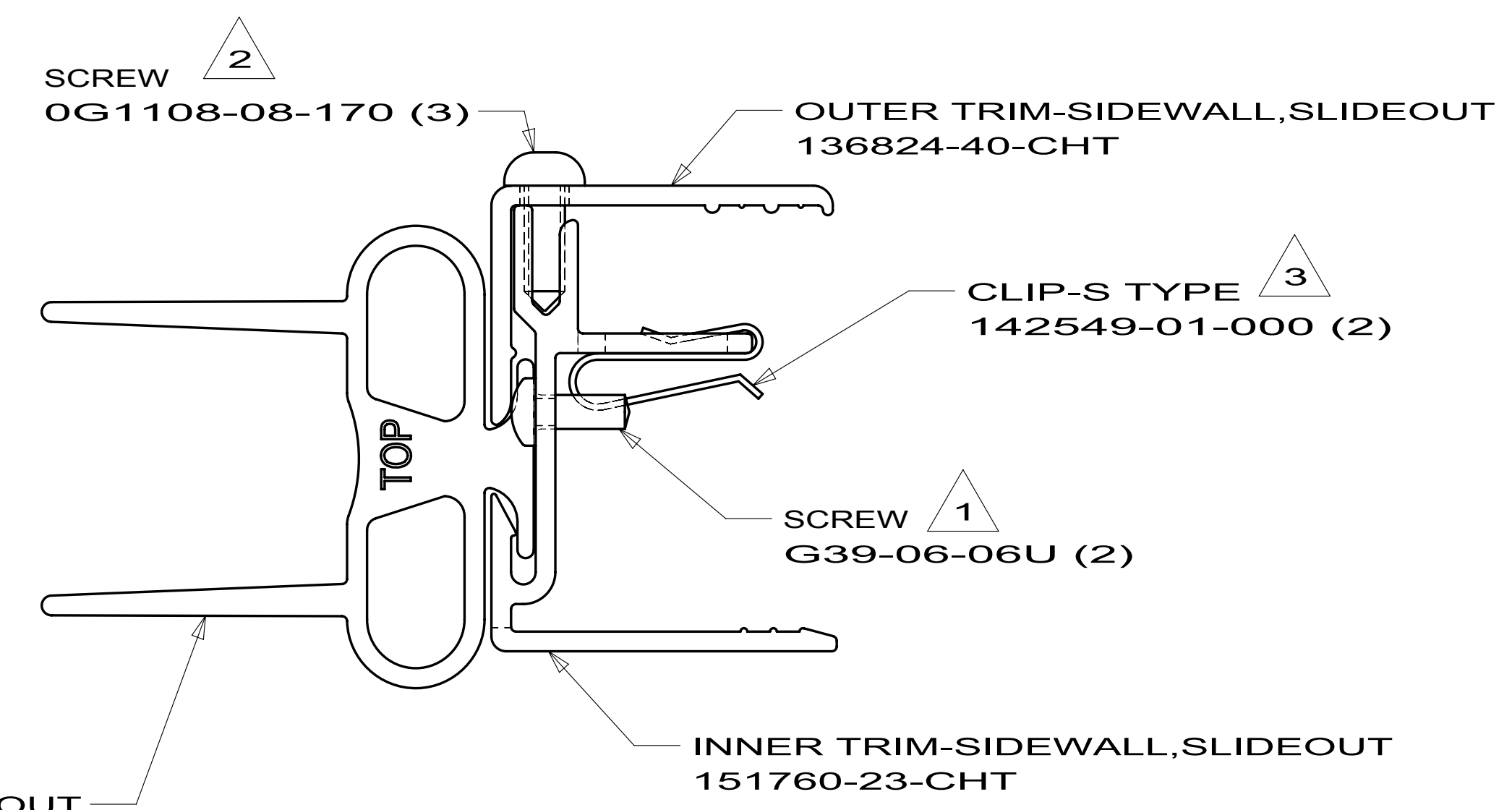
VIEW B
