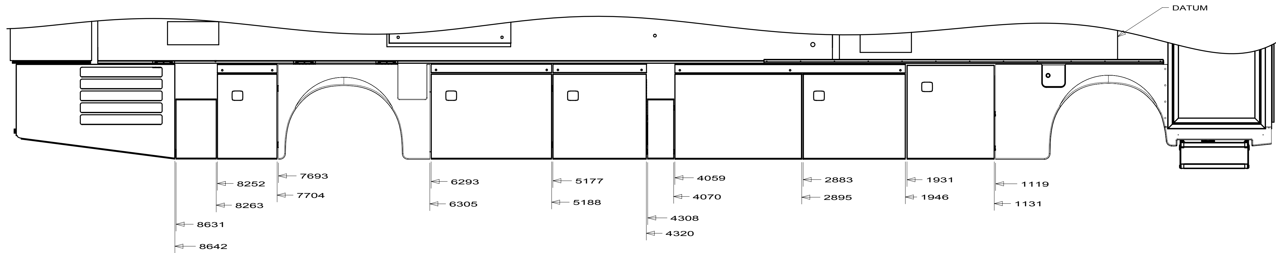
RIGHT SIDE COMPARTMENT DOORS
