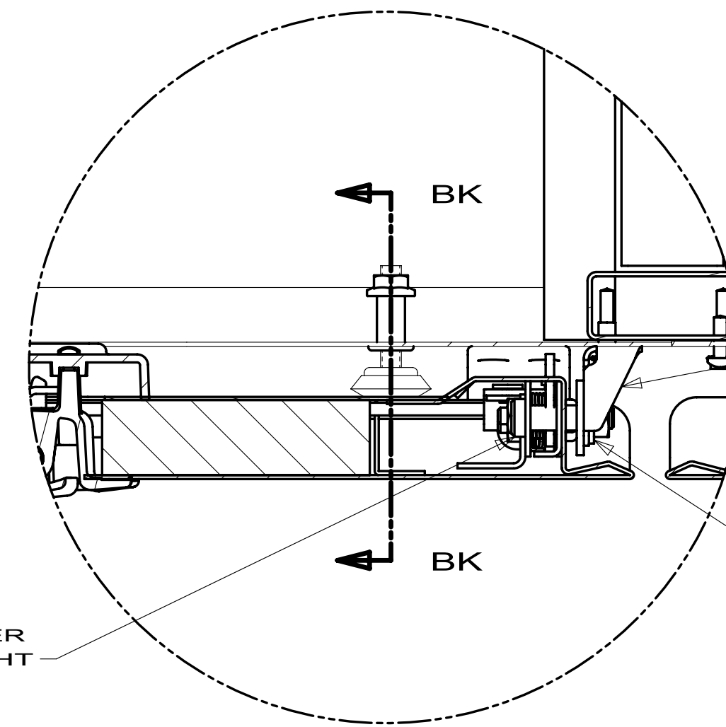
DETAIL BJ 6
