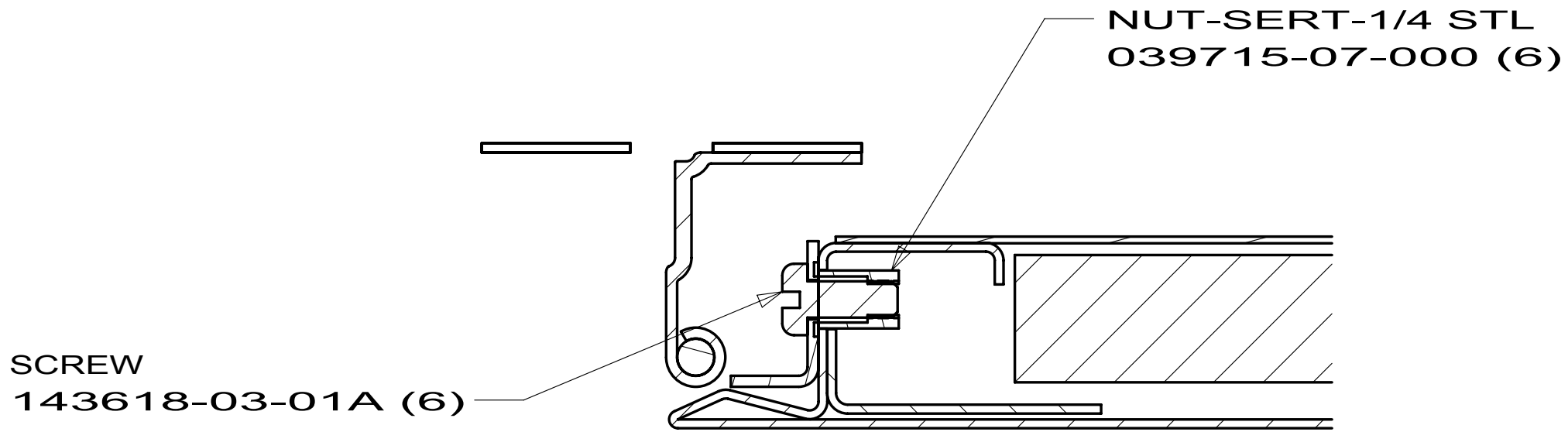
SECTION FC-FC
