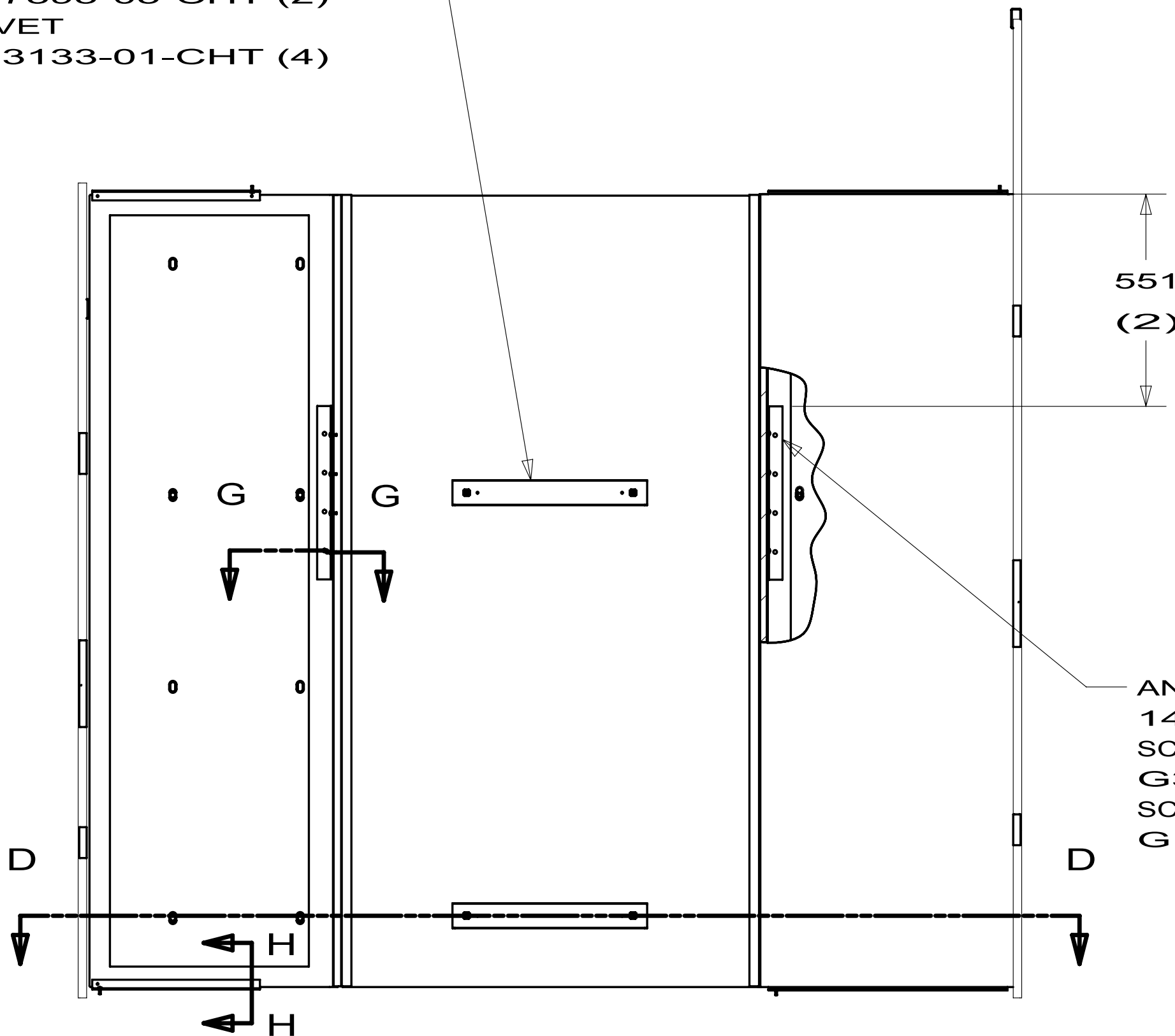
VIEW B
