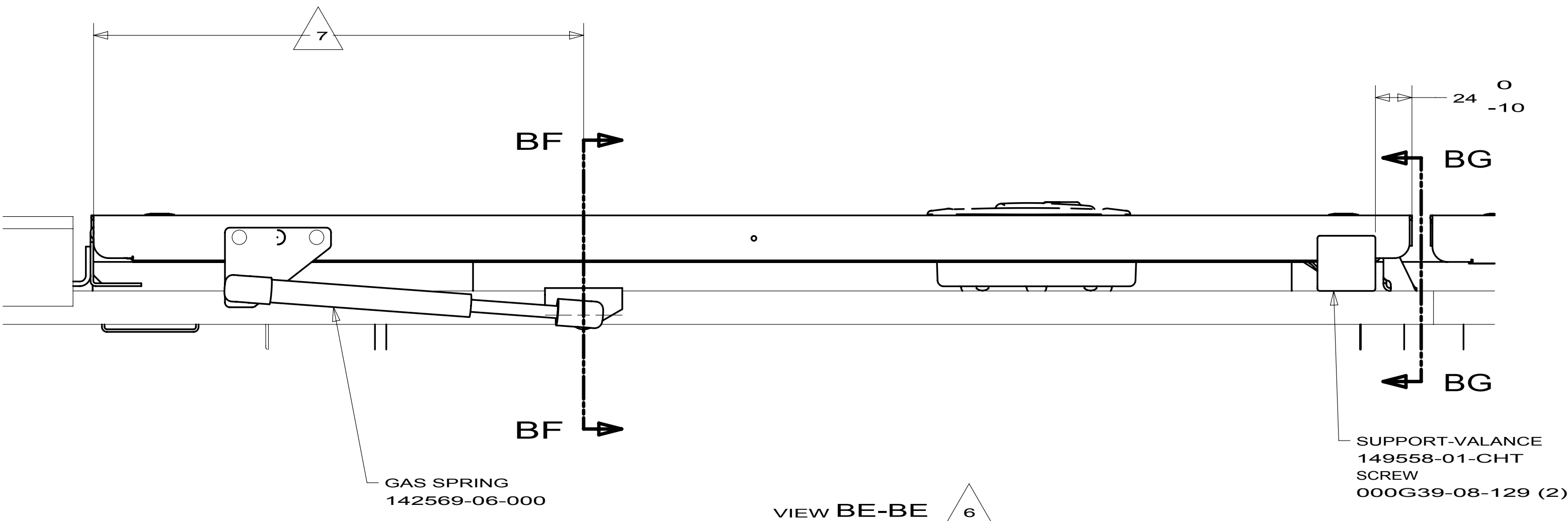
VIEW BE-BE 6
