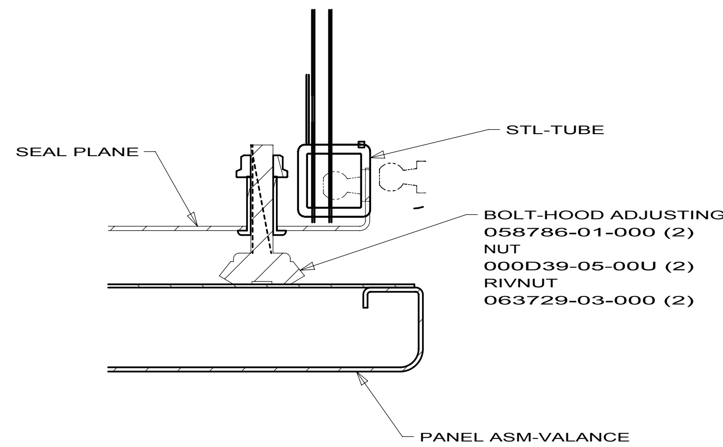
SECTION BK-BK 6
