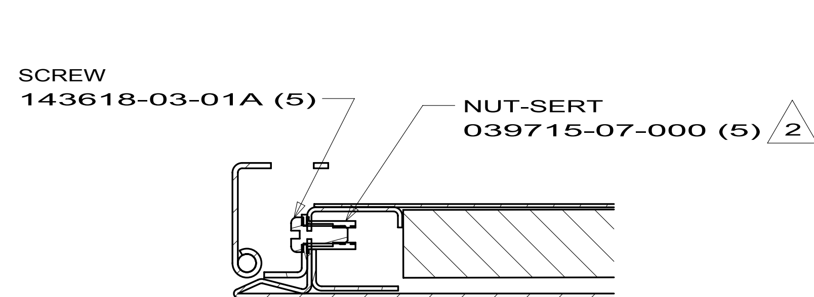
SECTION BA-BA
