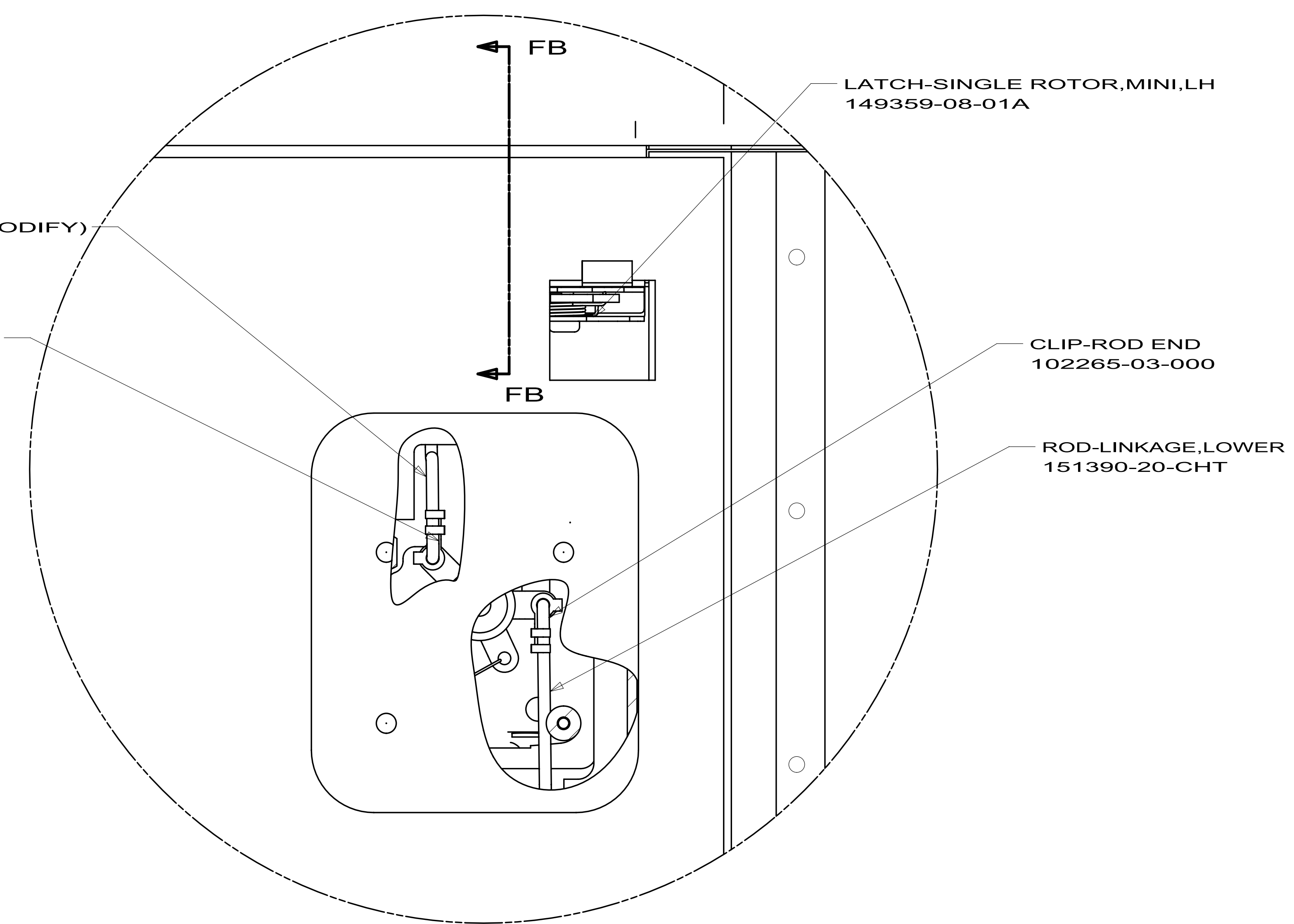
DETAIL FA
