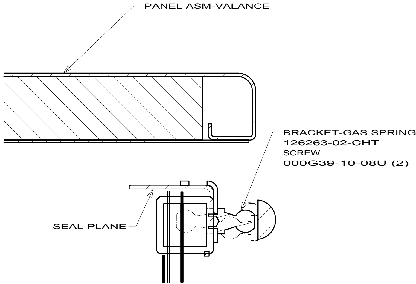
SECTION BF-BF 6
