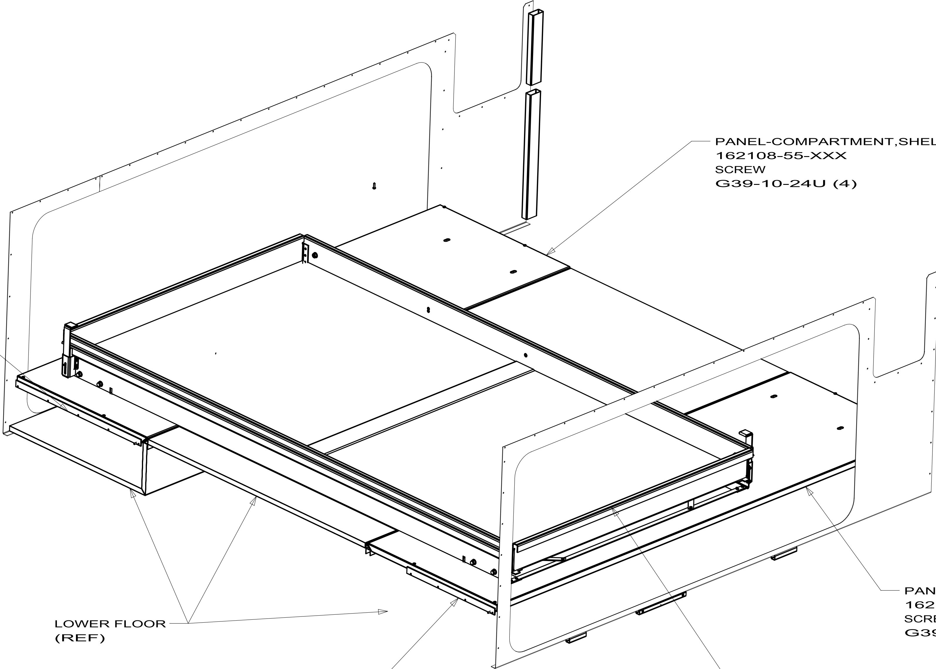
VIEW A
