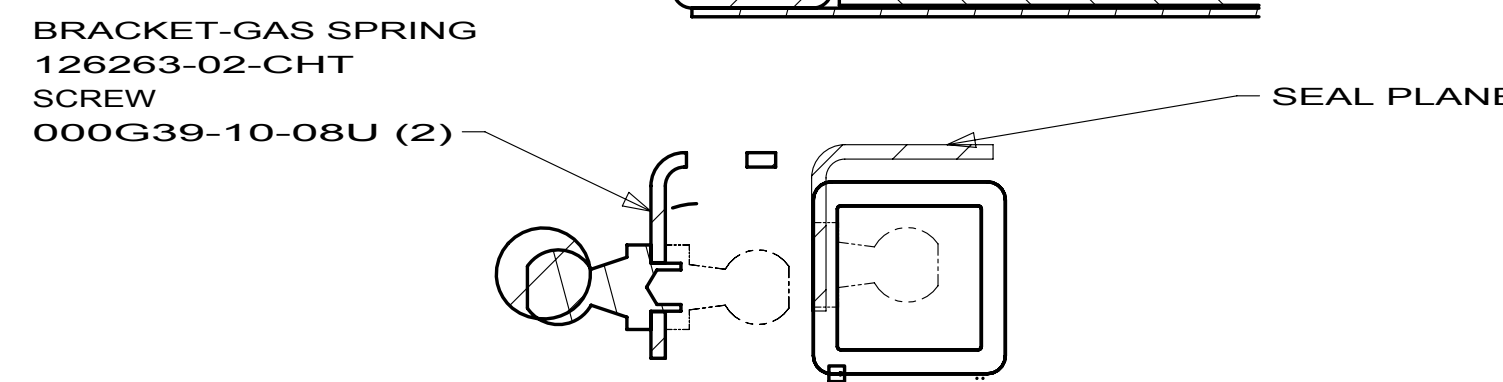
SECTION BN-BN 9
