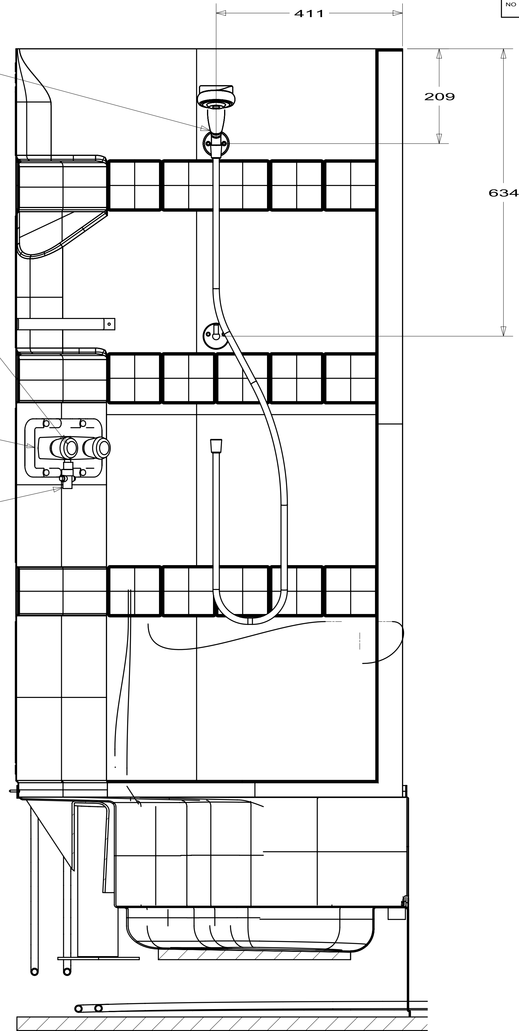
SECTION E-E (ROTATED)
