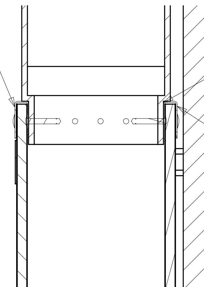
SECTION F-F
