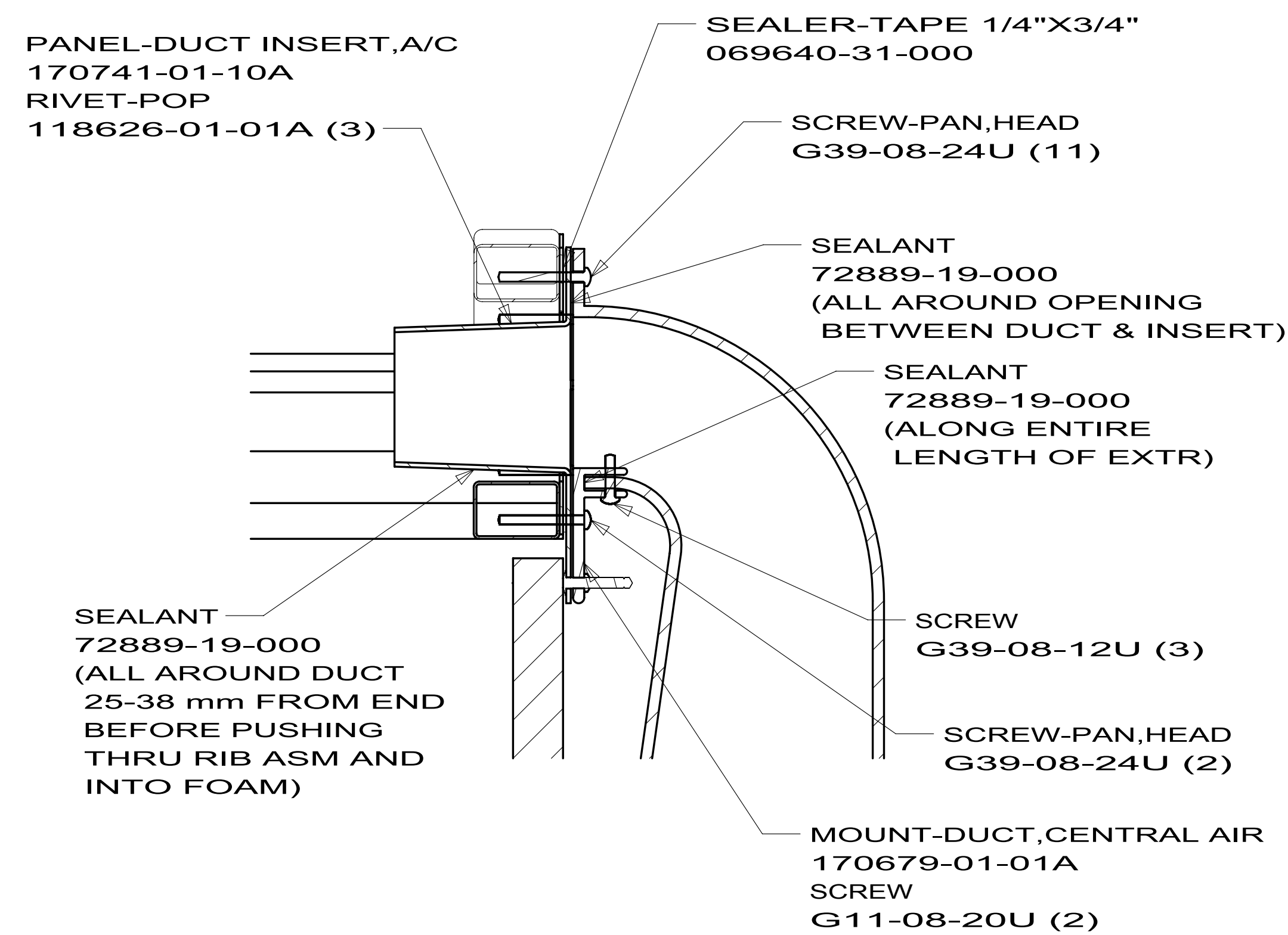
SECTION D-D (2 PLACES)
