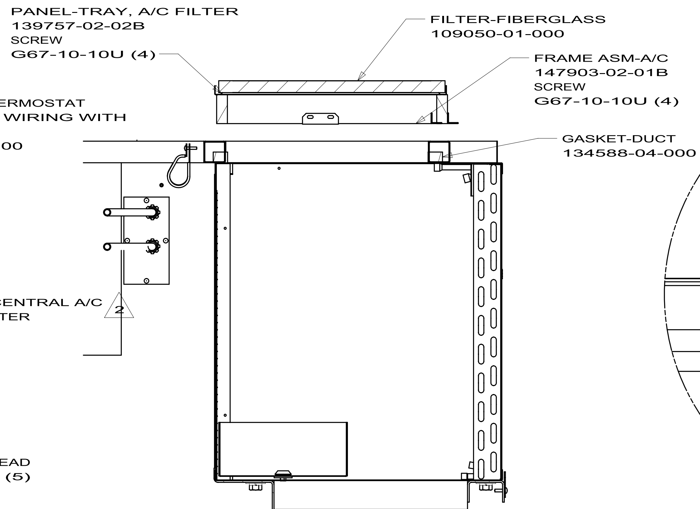
SECTION B-B
