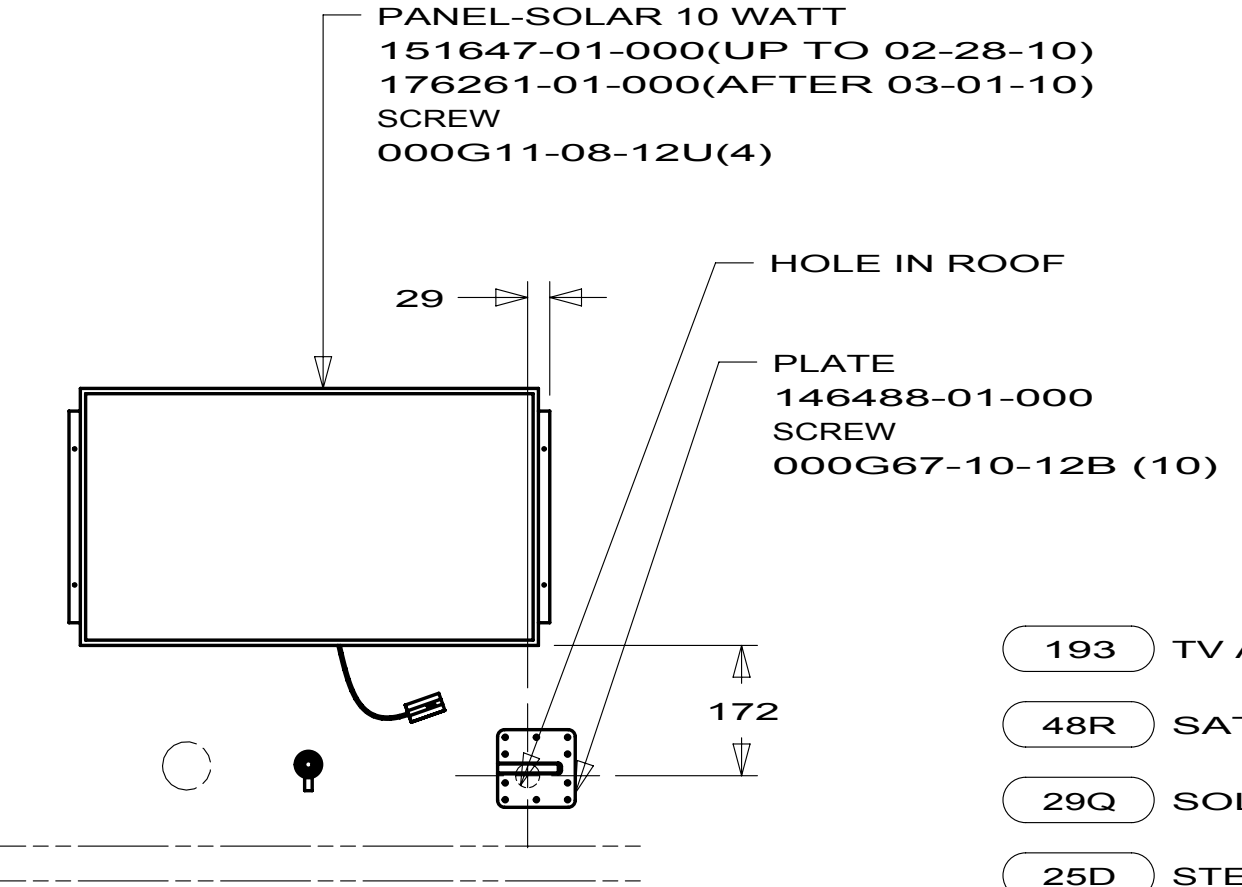
VIEW GC 29Q
