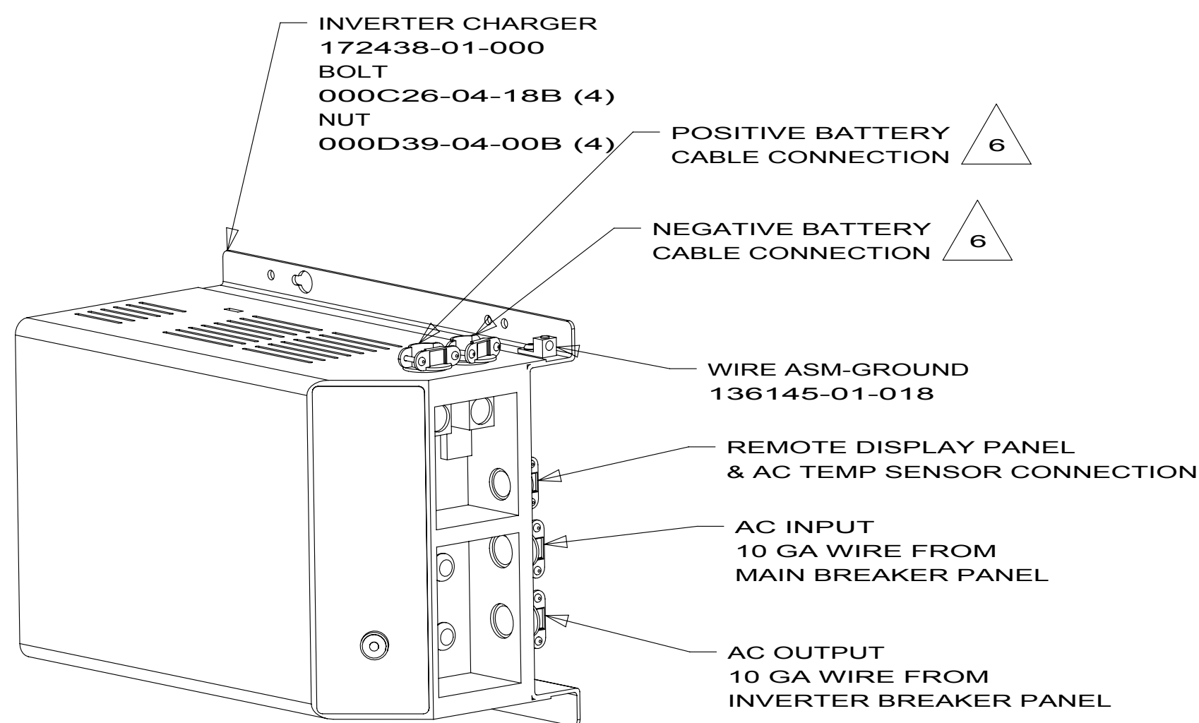
DETAIL DB
