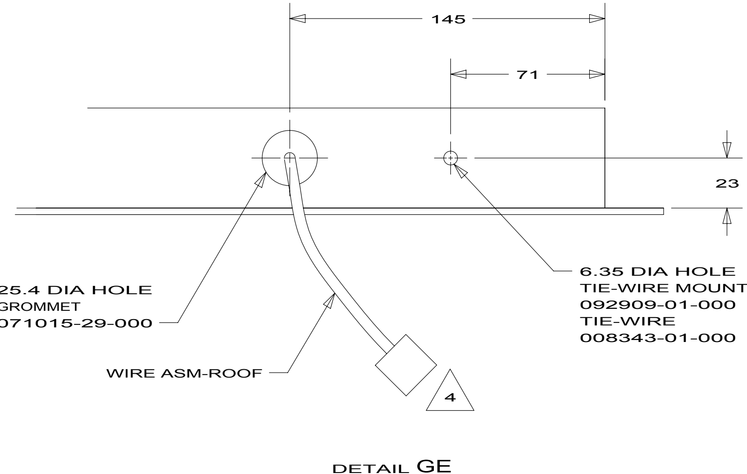
DETAIL GE
