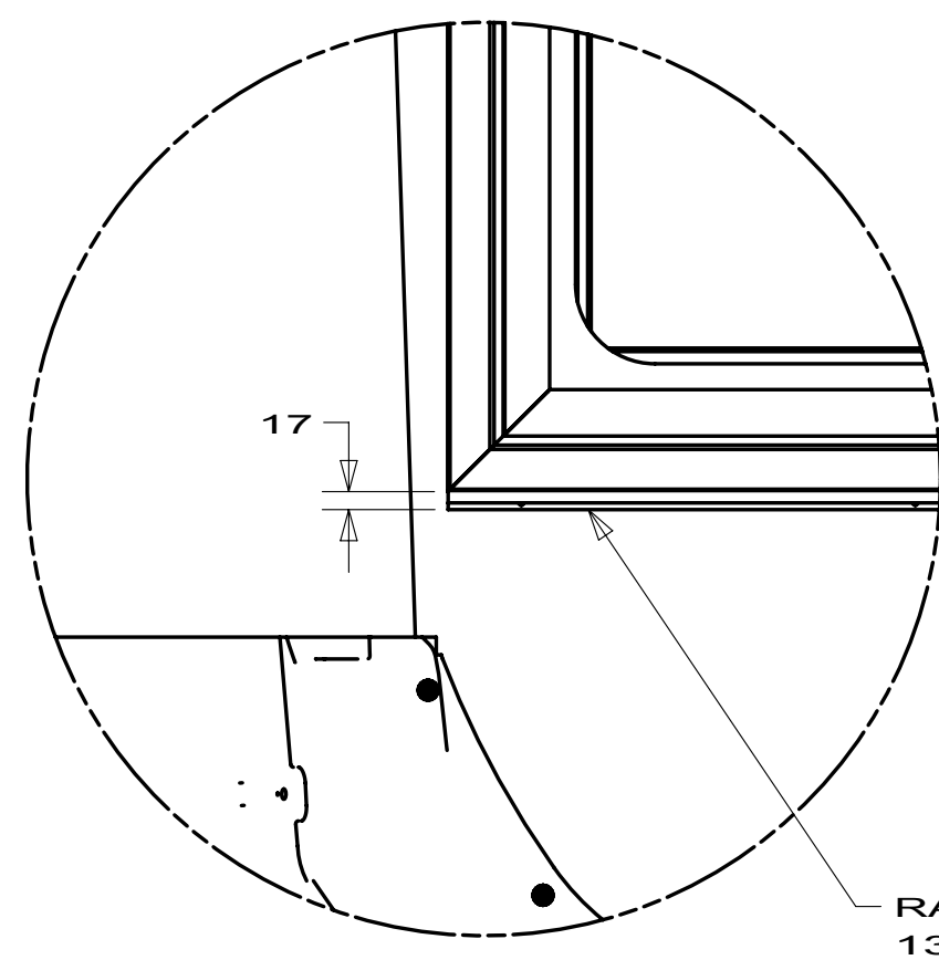
DETAIL B
