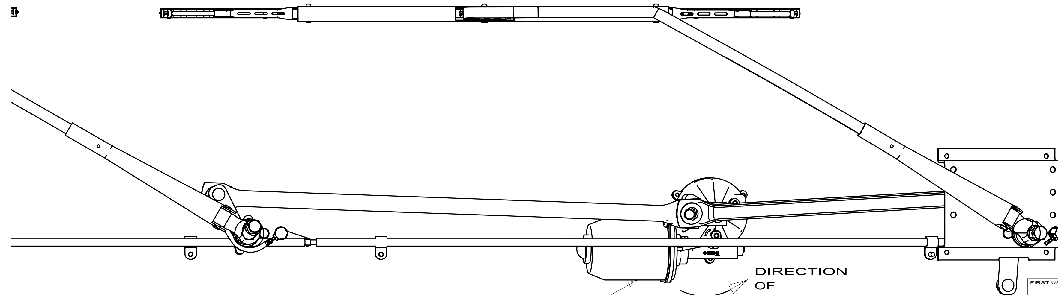
VIEW E MOTOR ASM-WIPER (REF--SHOWS IN PARK POSITION)
