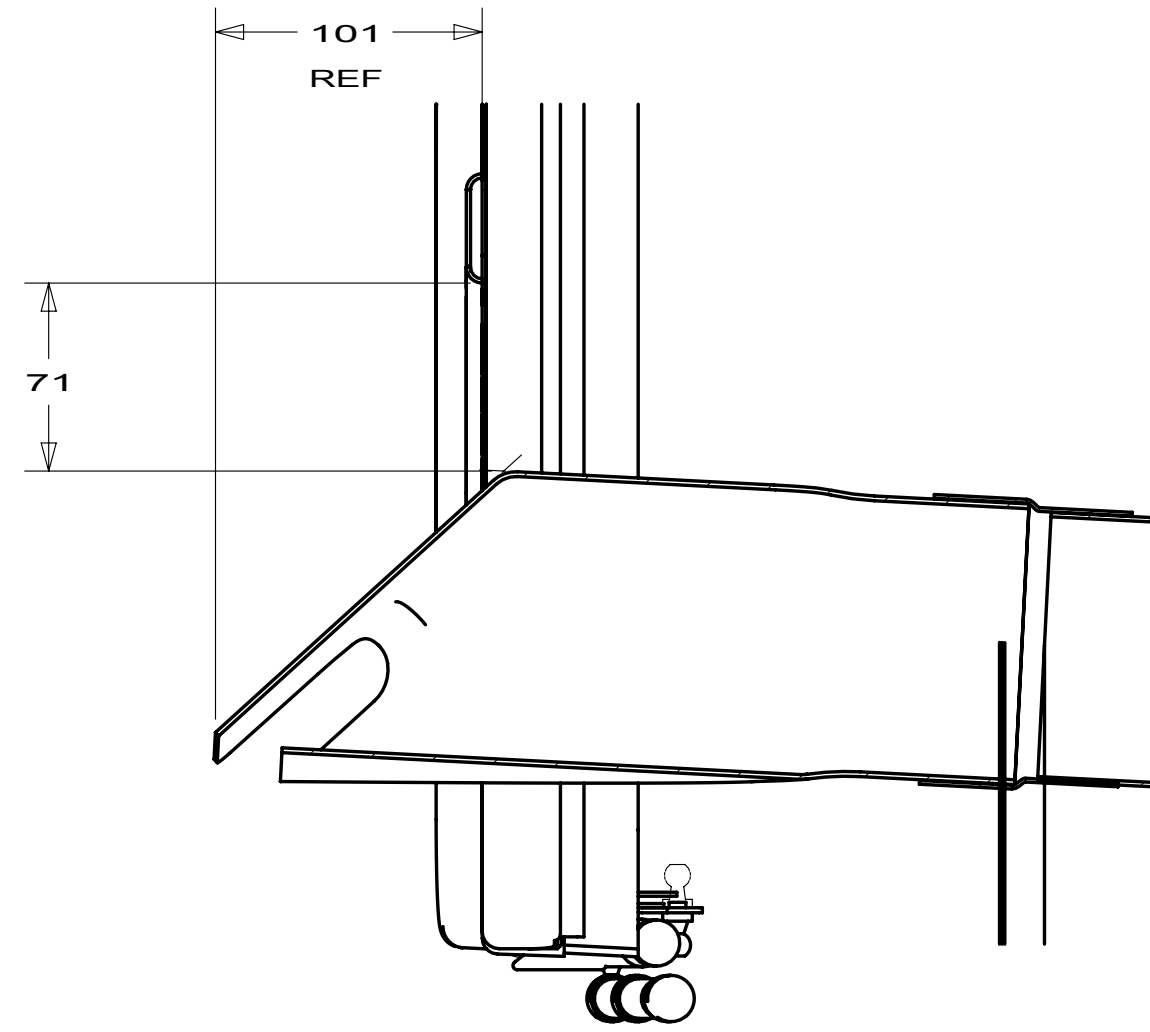
SECTION BM-BM
