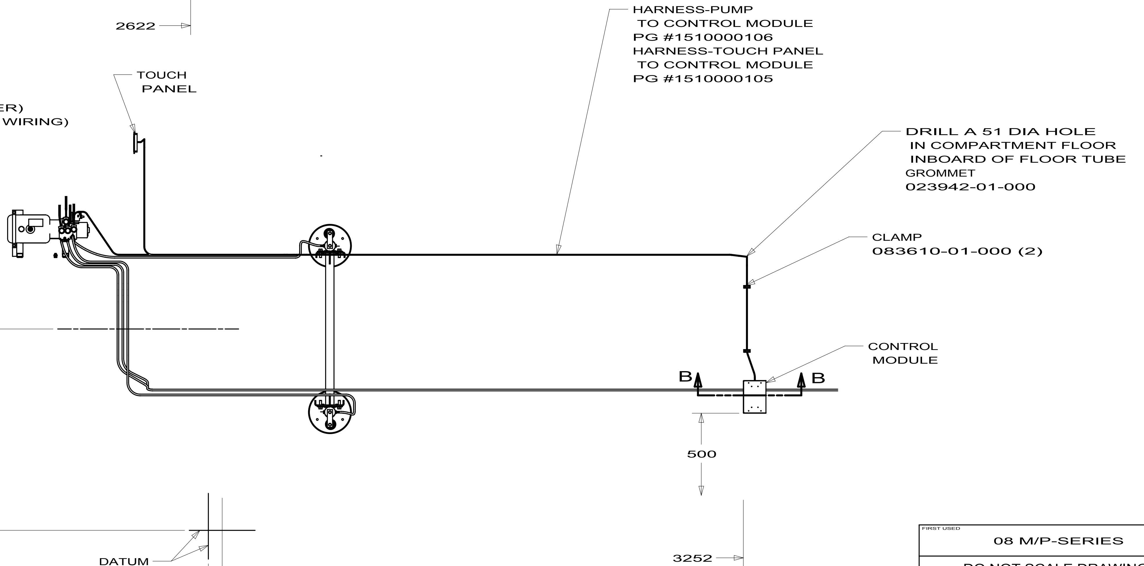
P39N (FREIGHTLINER) (CONTROL MODULE WIRING)
