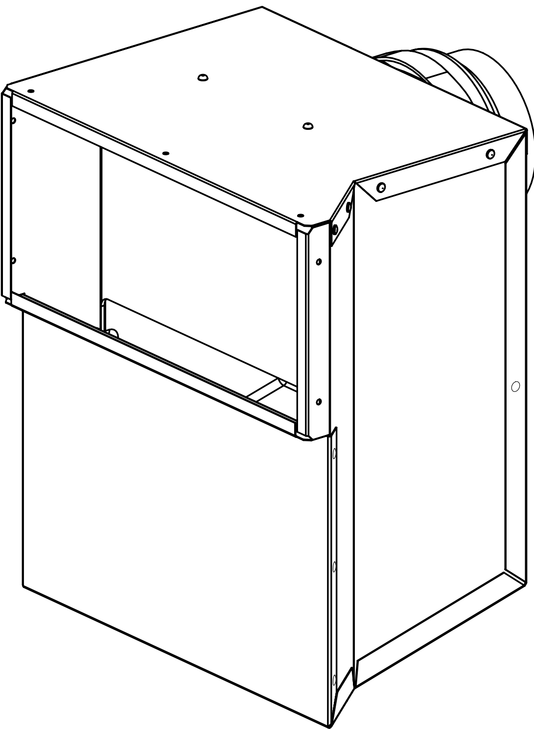
BOX ASM-INTAKE, ENGINE AIR 166777-01-02B
