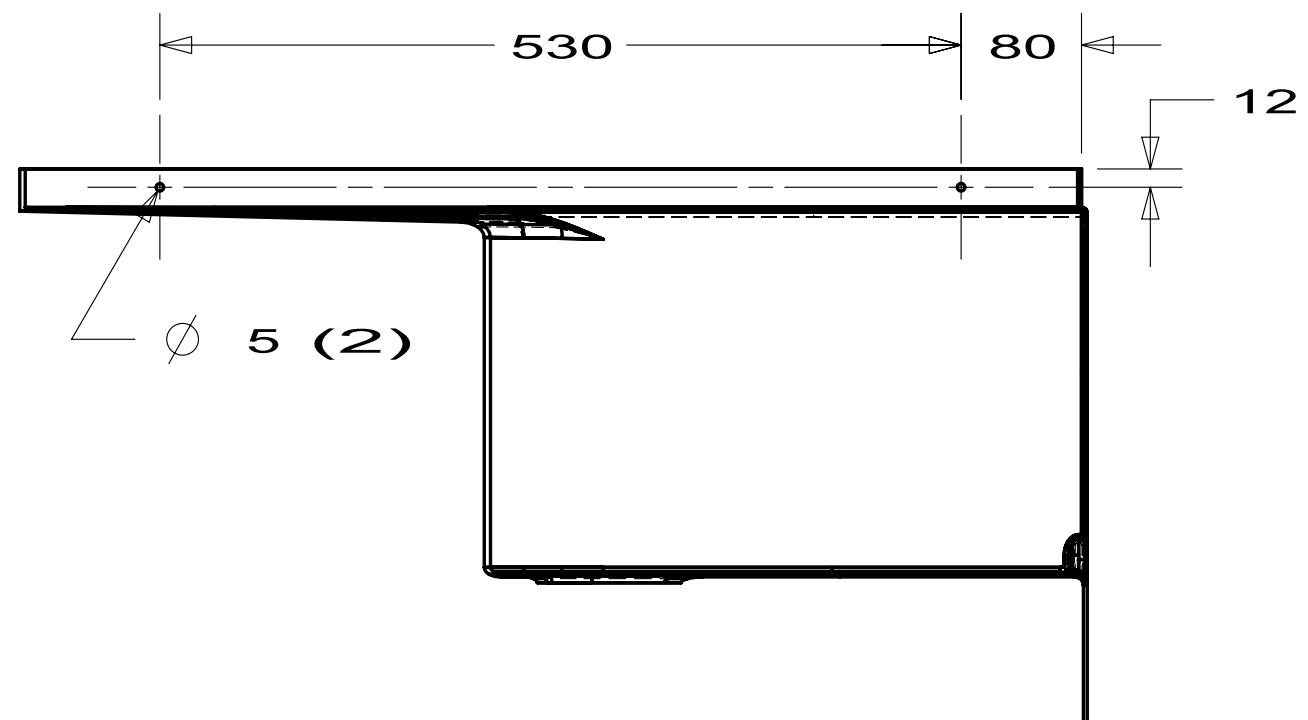
SECTION S-S
