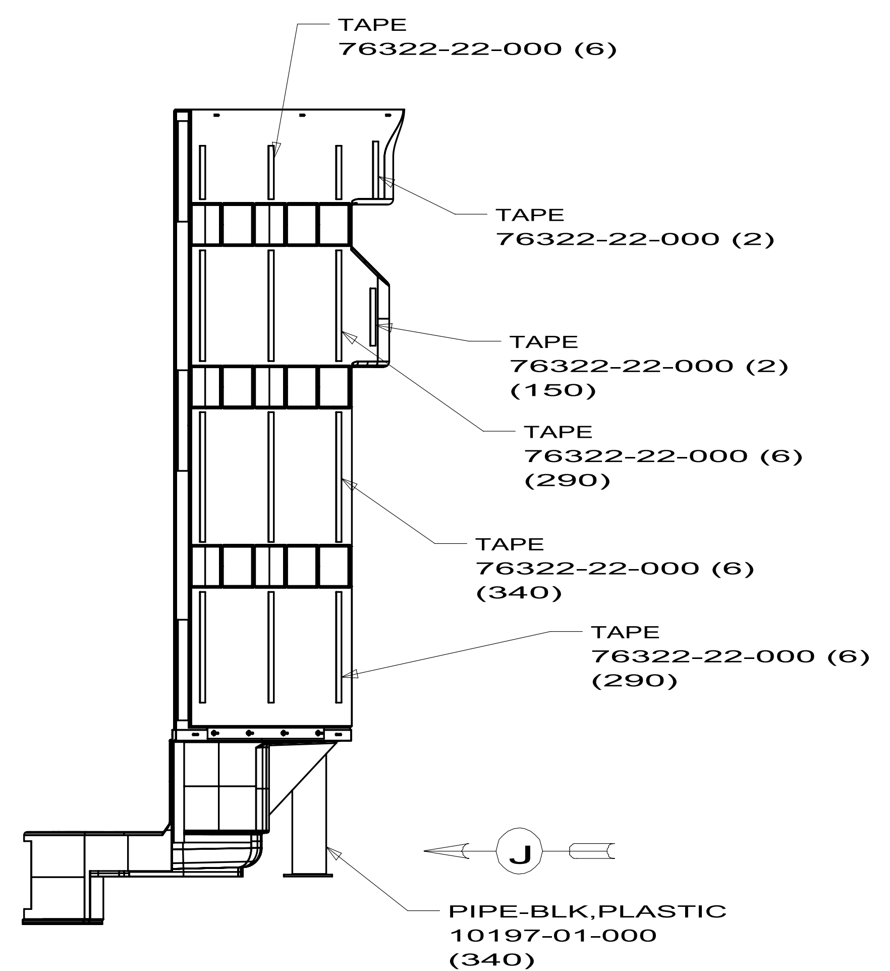
VIEW F
