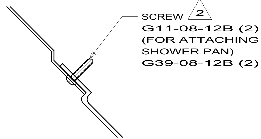
SECTION E-E
