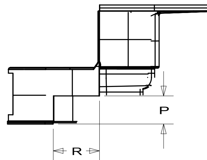
VIEW N
