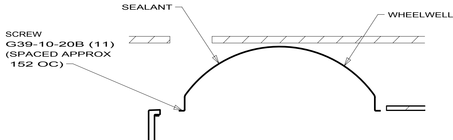
SECTION AF-AF
