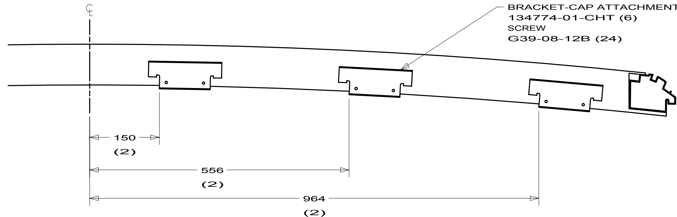
SECTION AH-AH
