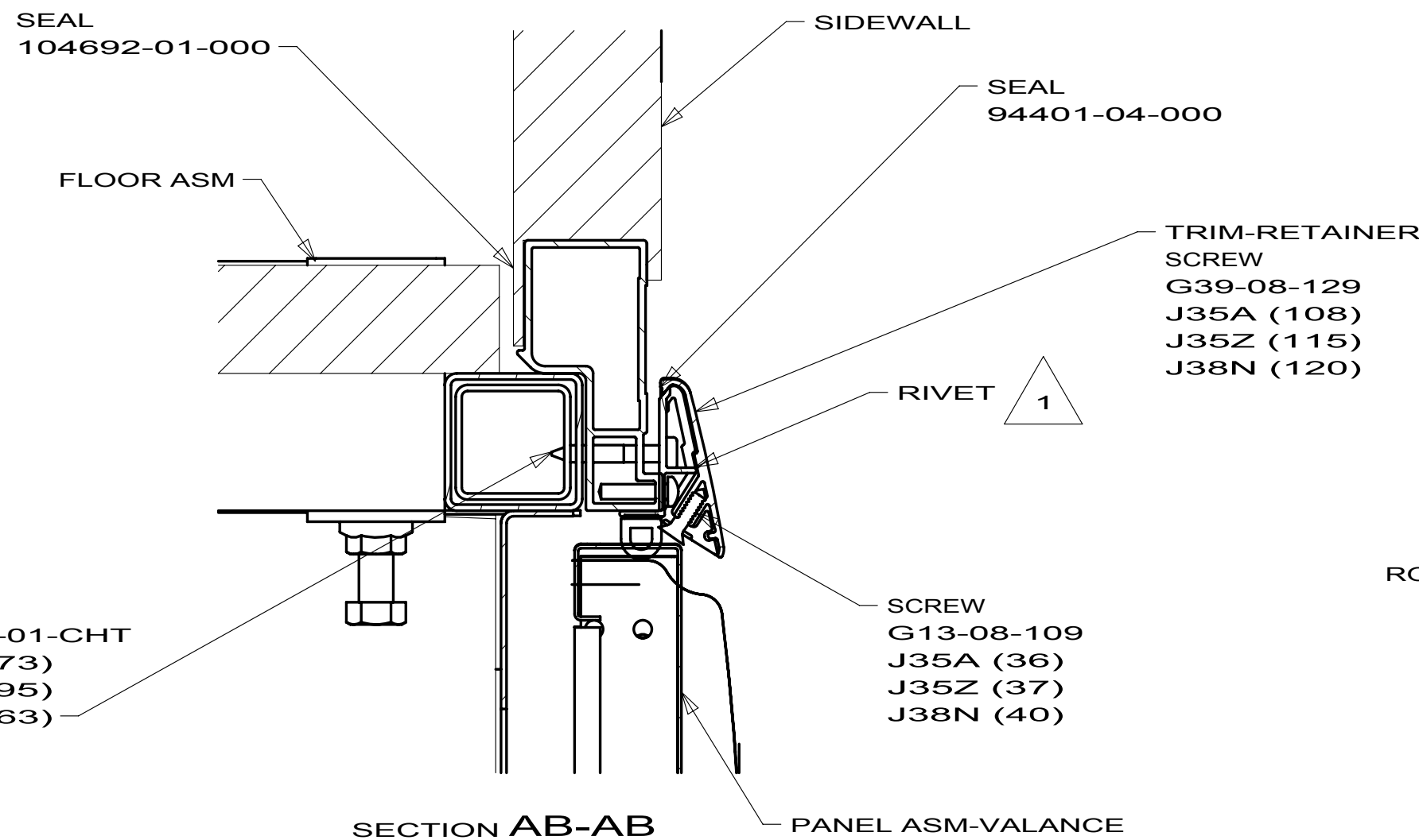
SECTION AB-AB
