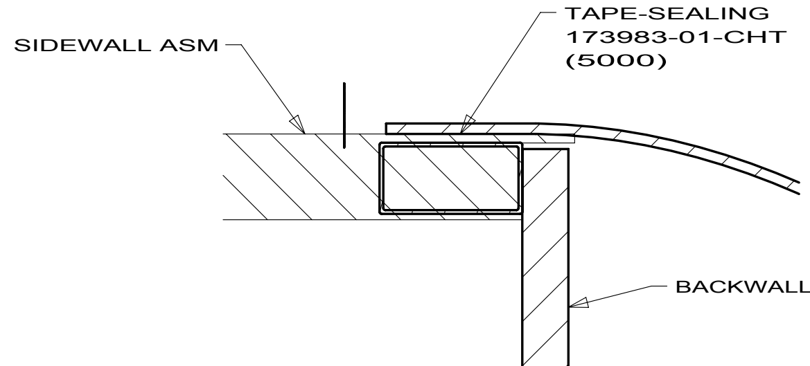
SECTION AD-AD
