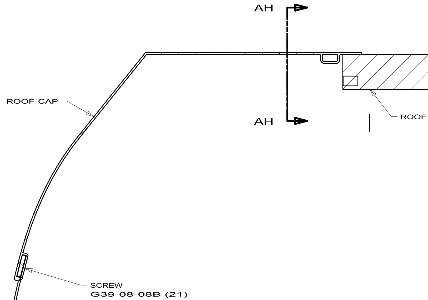
SECTION AC-AC
