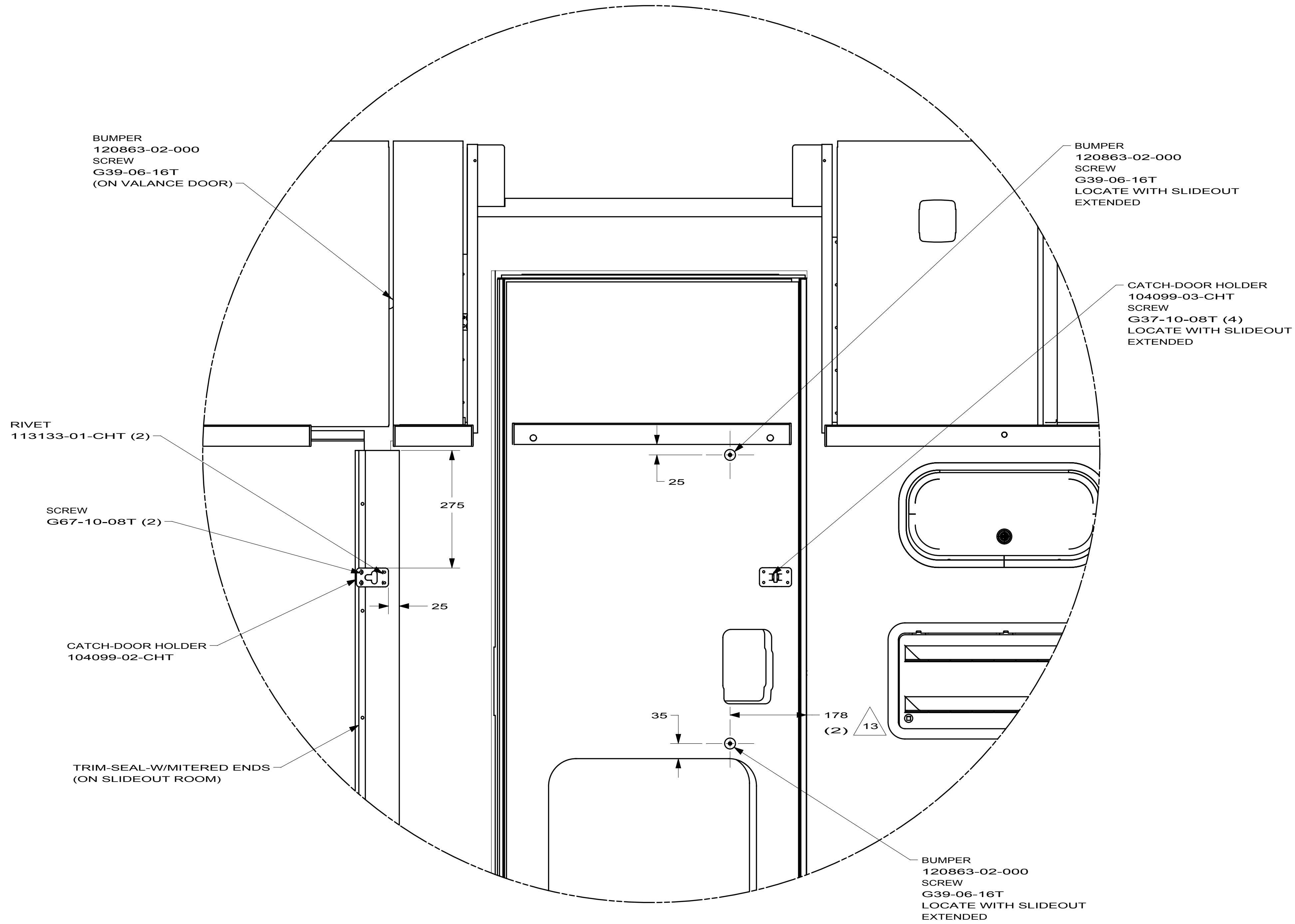
DETAIL A
