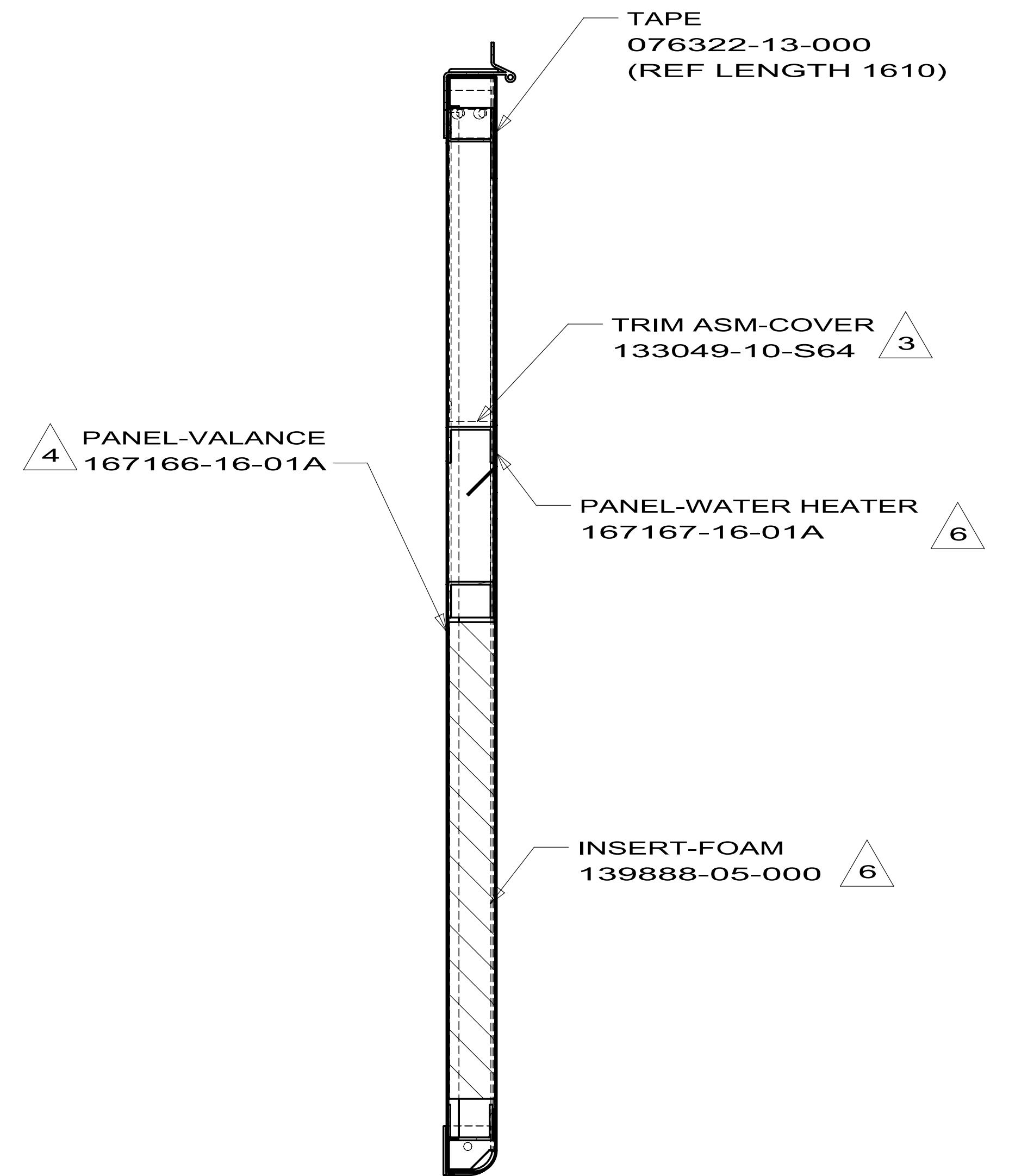
SECTION TA-TA
