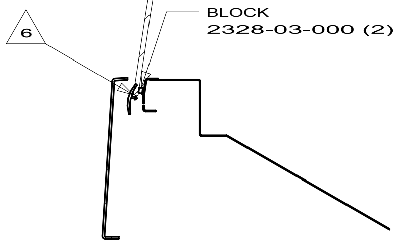
SECTION AC-AC
