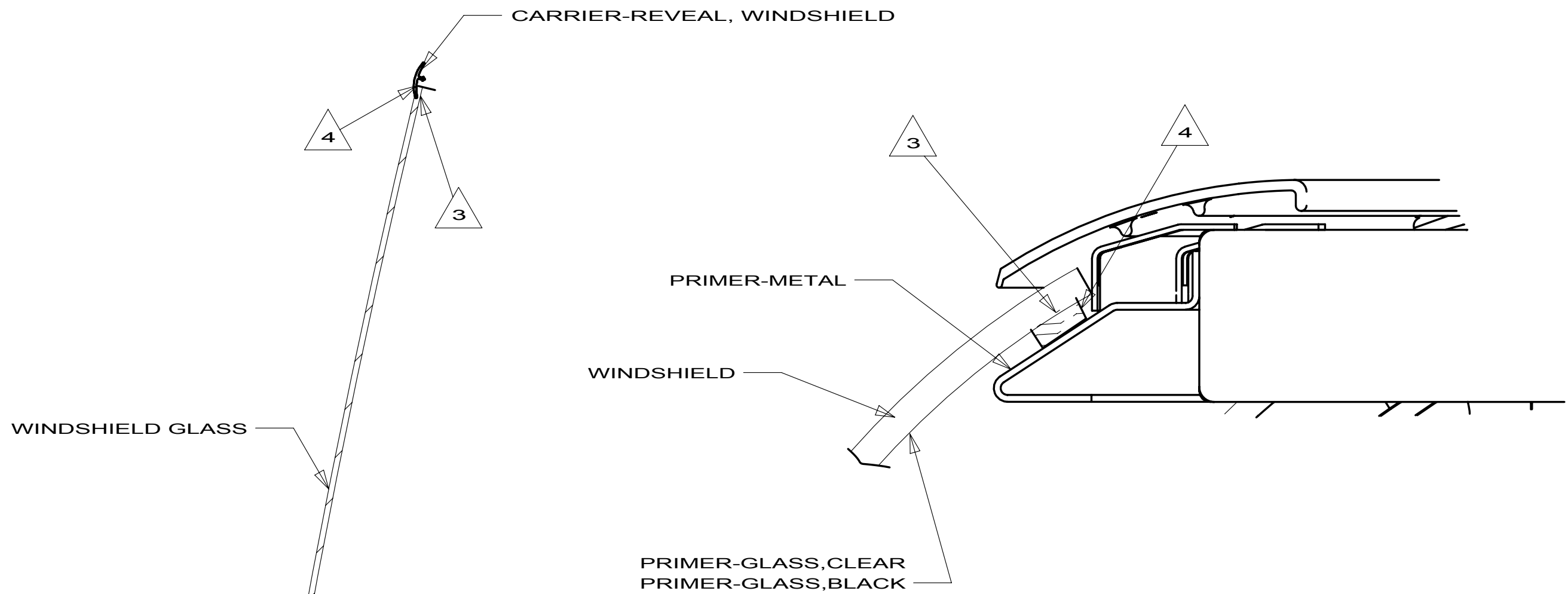
SECTION AB-AB
