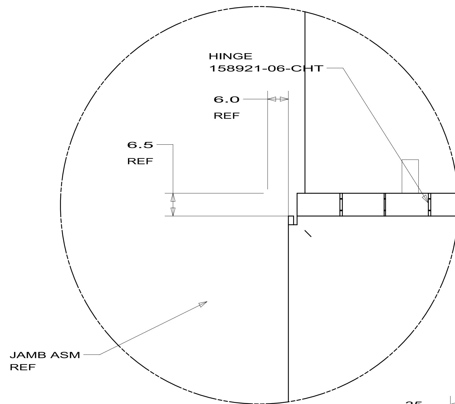
DETAIL BH
