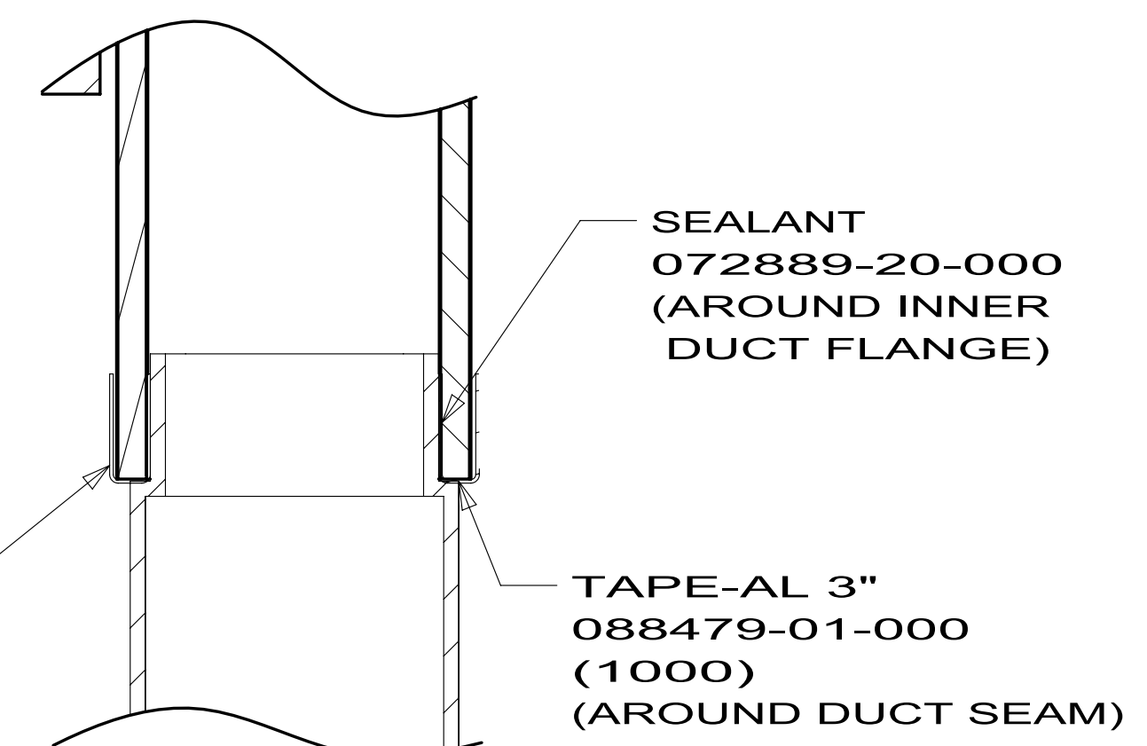
SECTION BE-BE PART OF P38842-01-000
