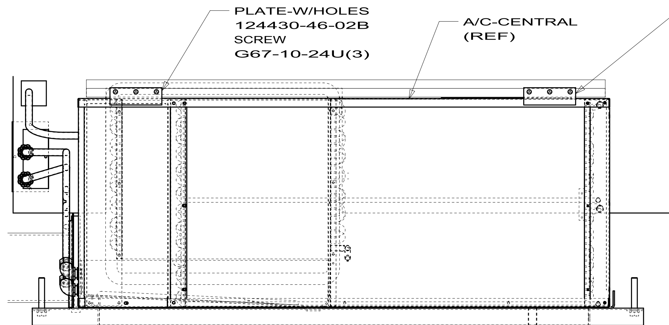
SECTION CA-CA
