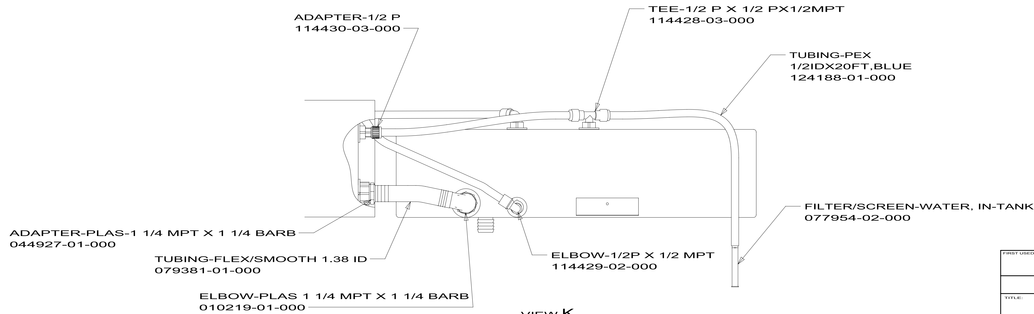
VIEW K
