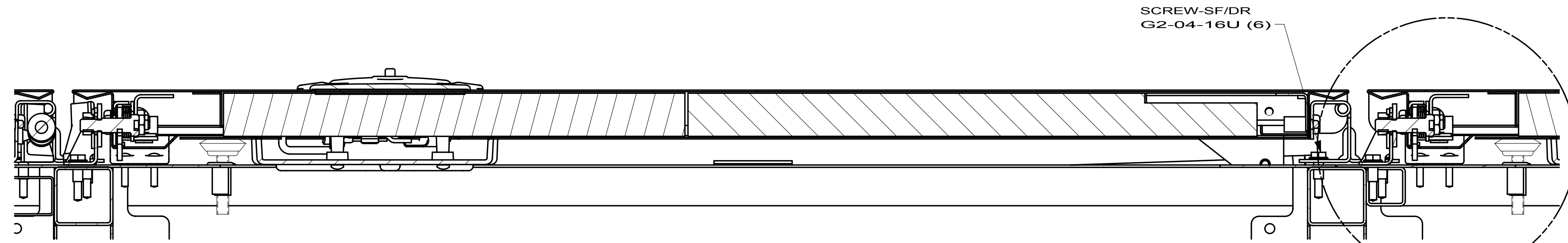
SECTION BG-BG
