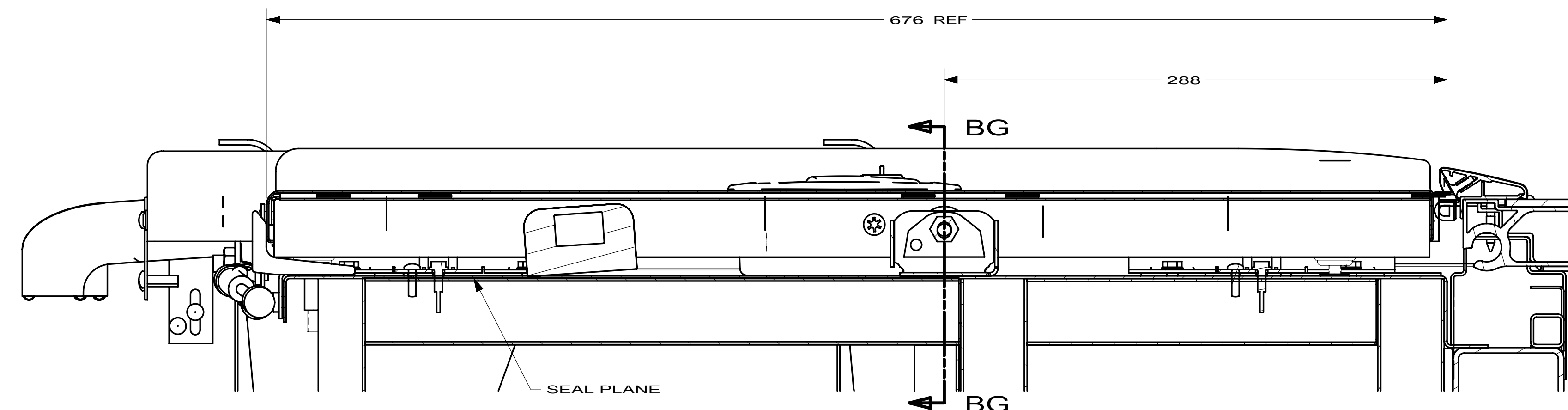
SECTION BF-BF
