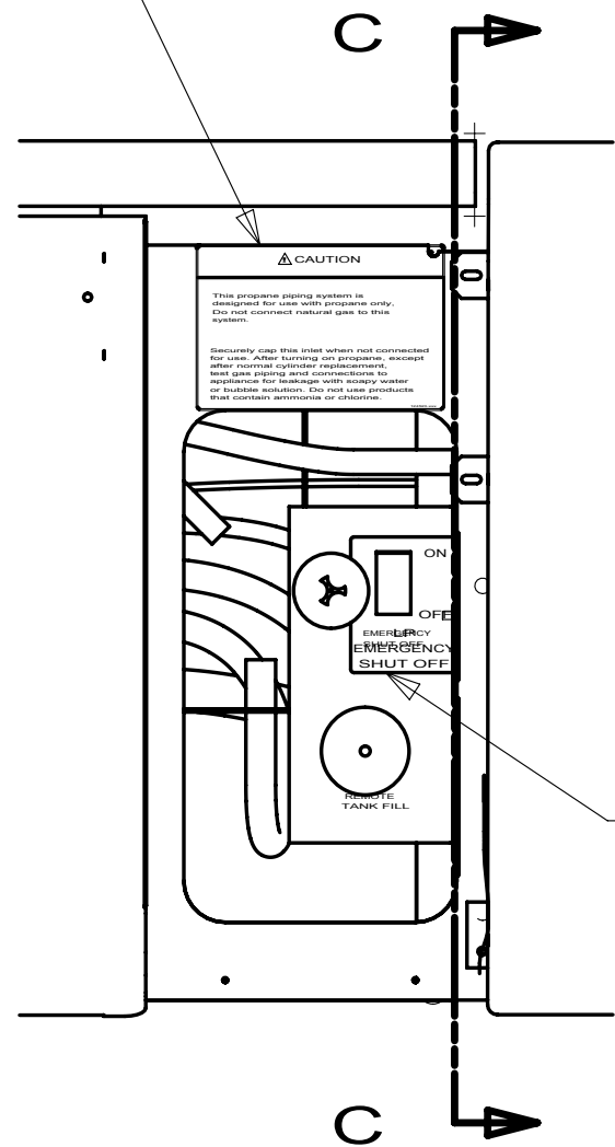
LABEL-PANEL SWITCH 130170-08-000
