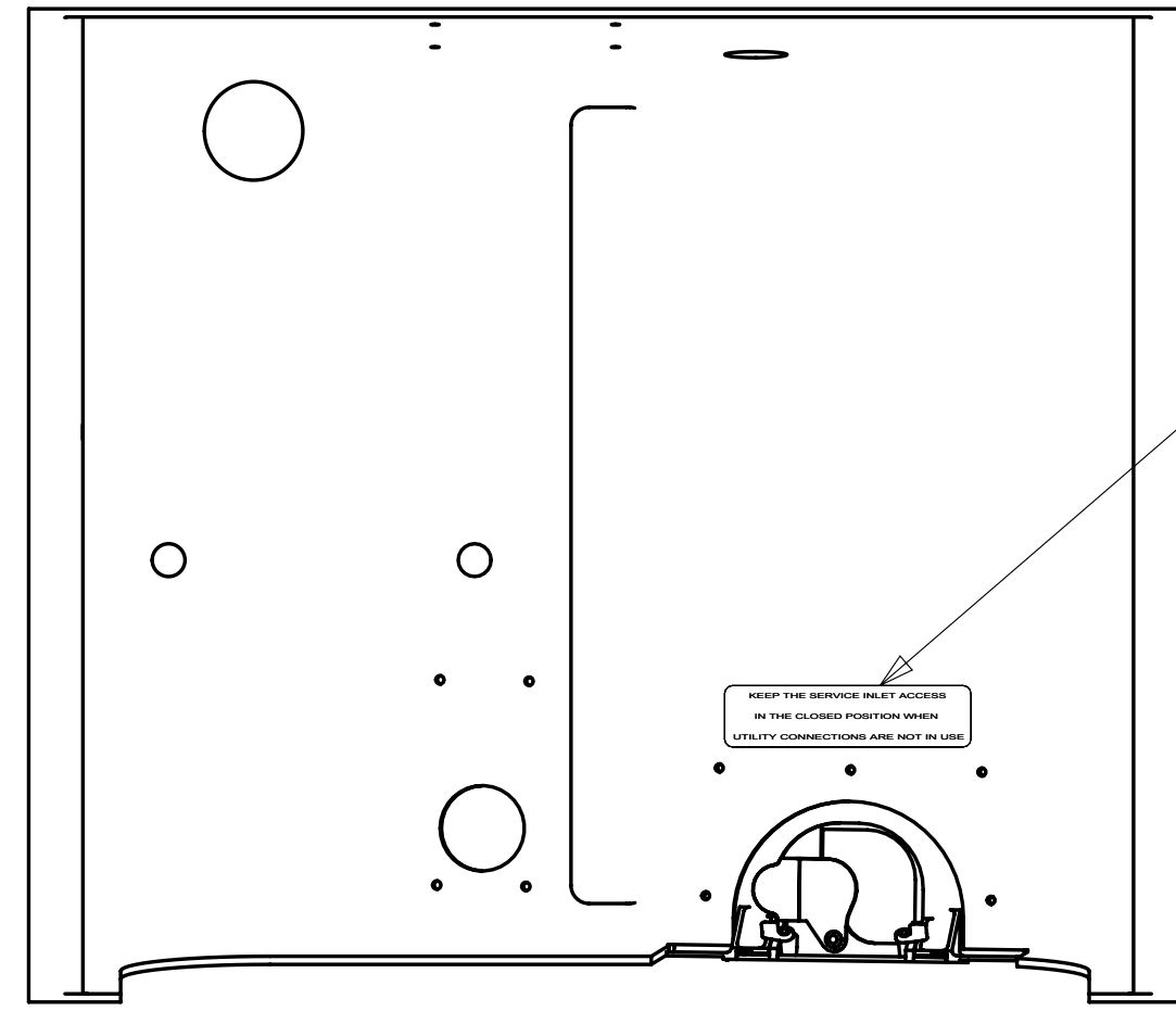
LABEL-SERVICE/UTILITY ACCESS 123562-01-000
