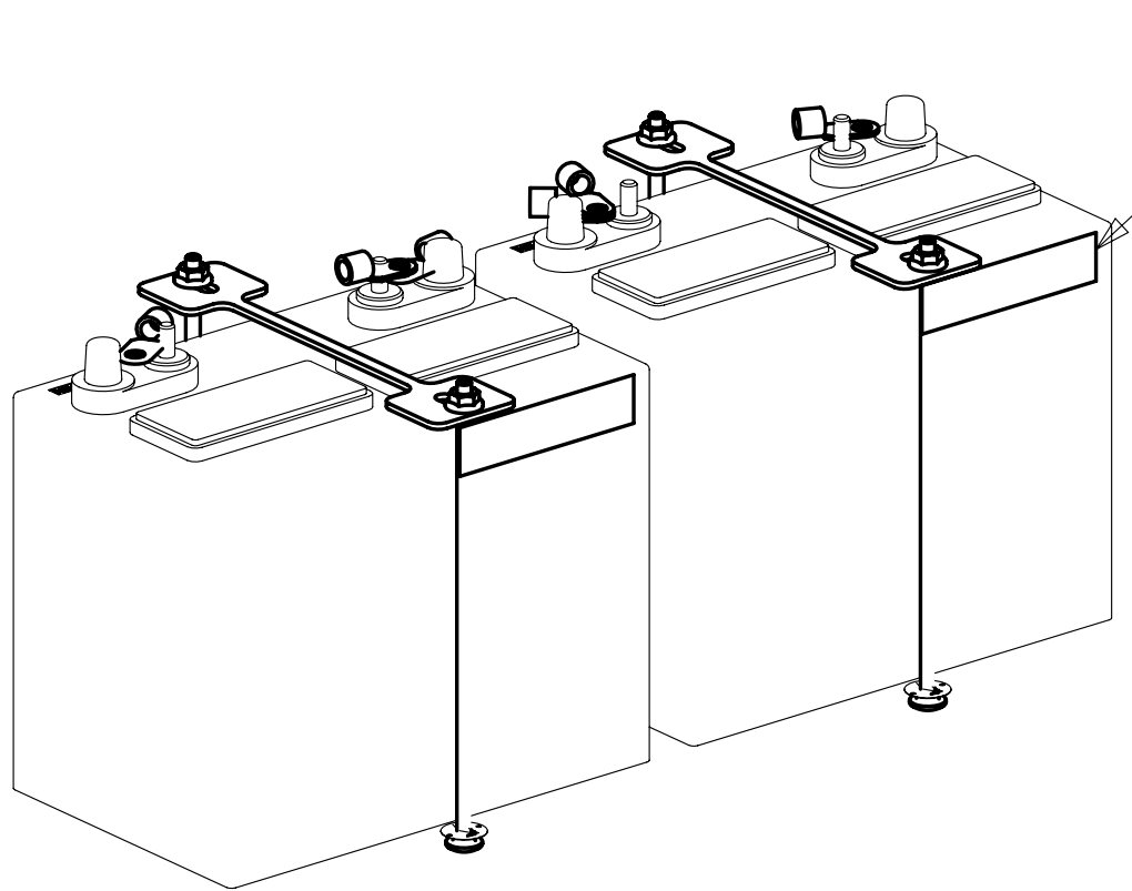
COACH BATTERIES
