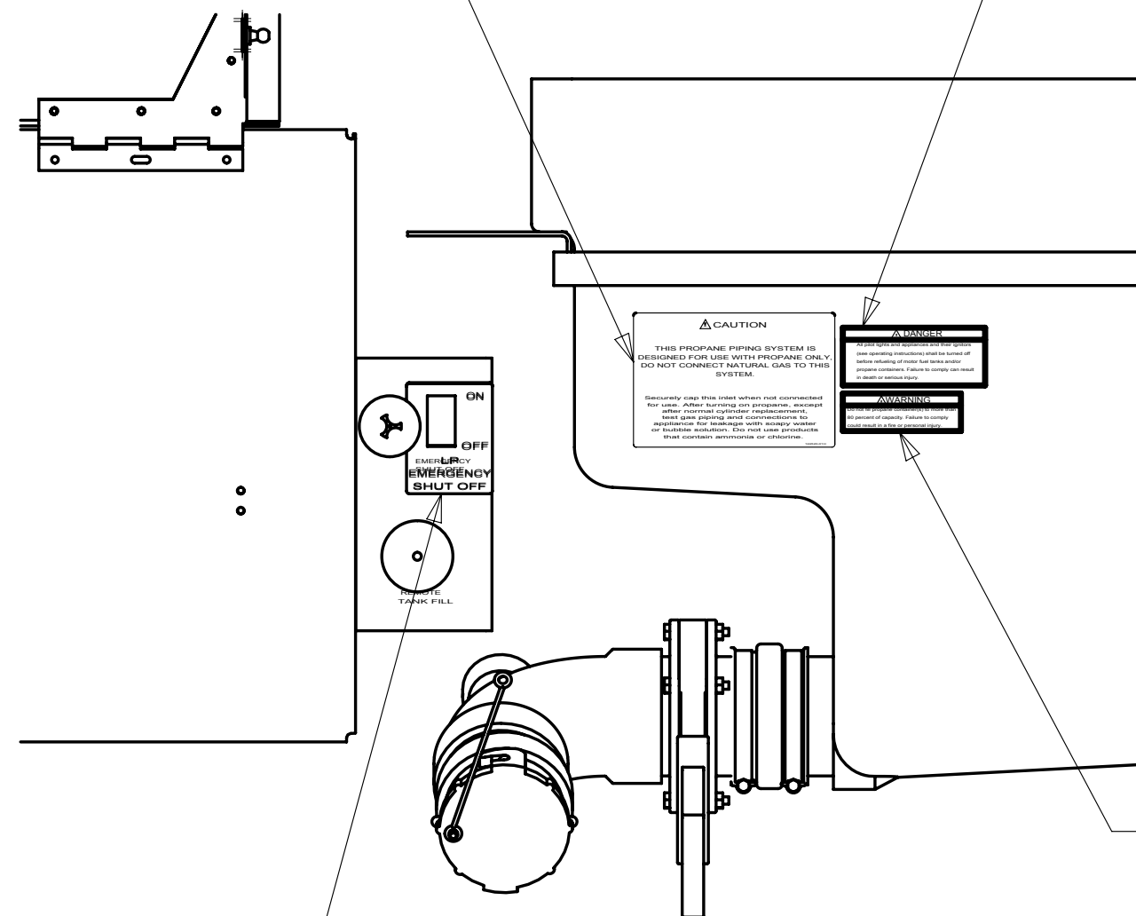
LABEL-LPG 80% CAPACITY 079965-02-000
