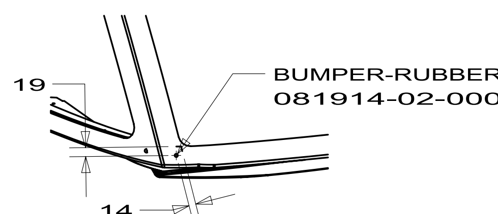
VIEW AD RH SHOWN (LH OPPOSITE)
