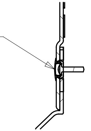
SECTION C-C
