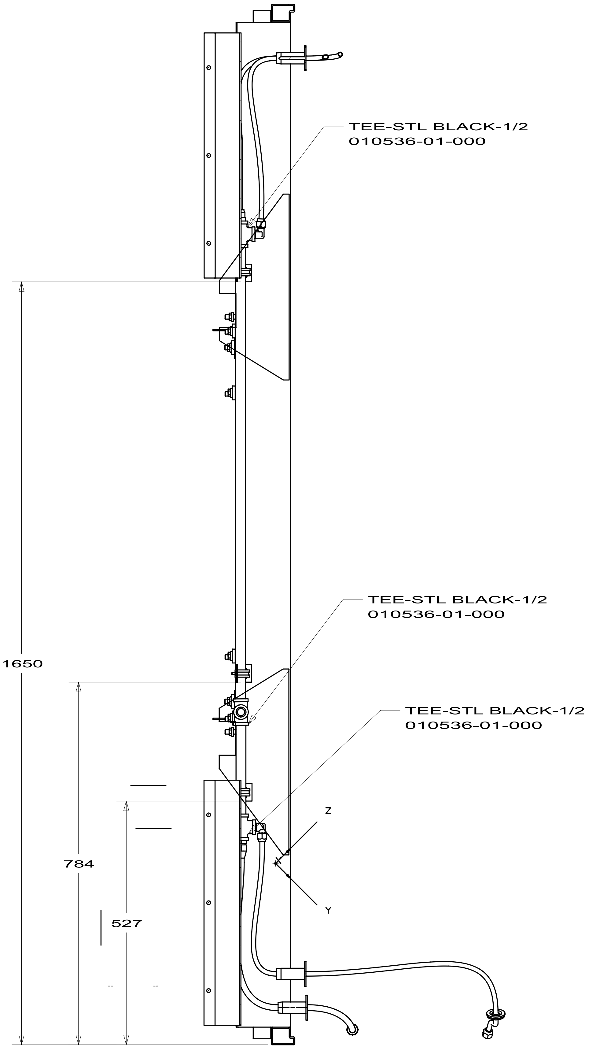
SECTION BB-BB
