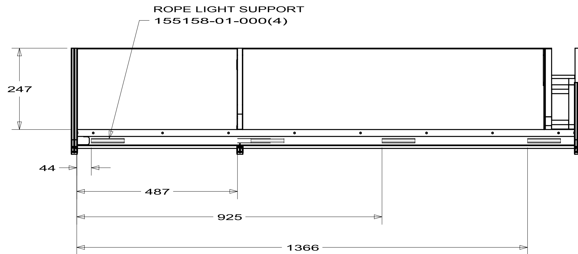
VIEW J
