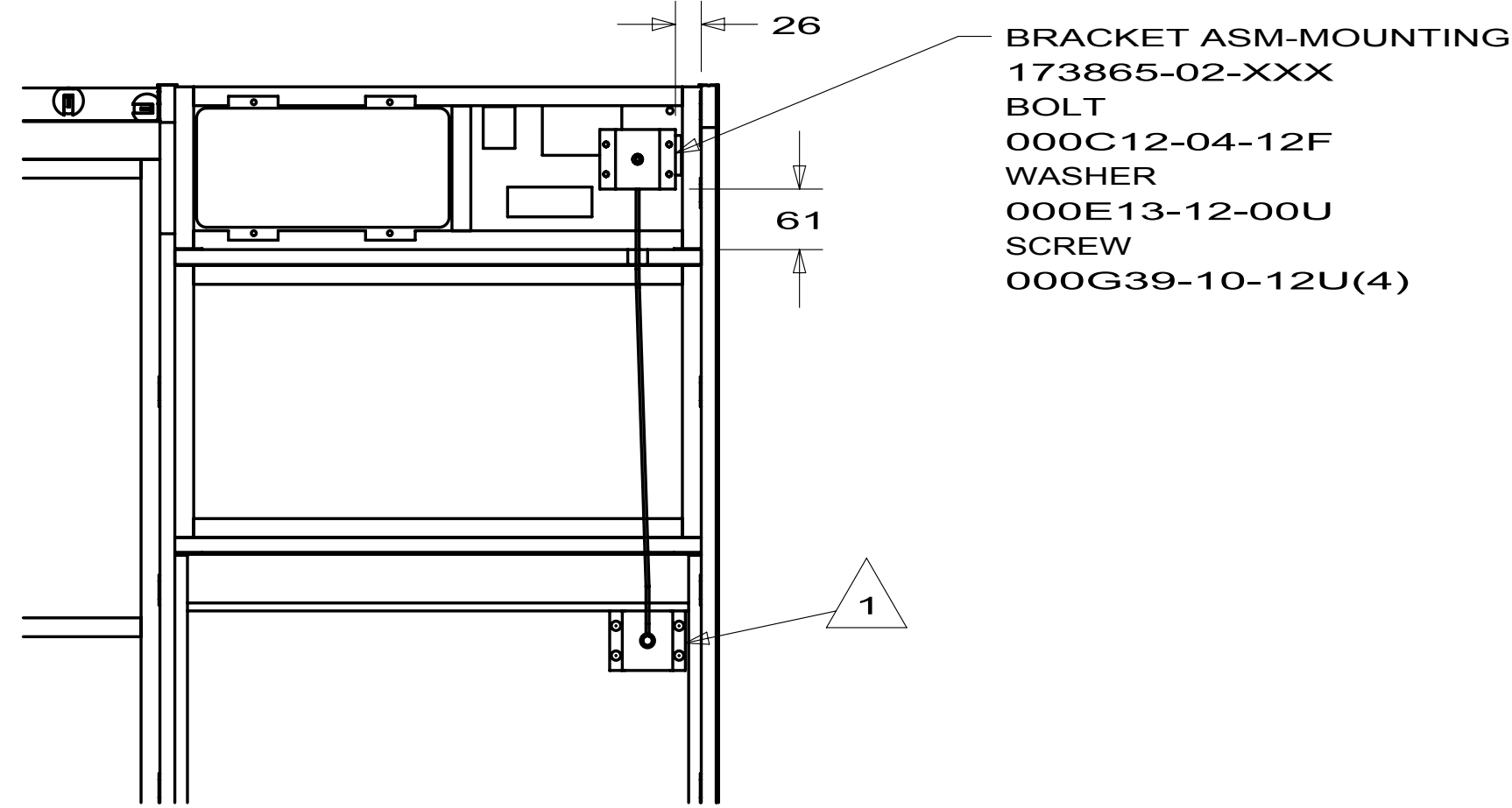
VIEW A
