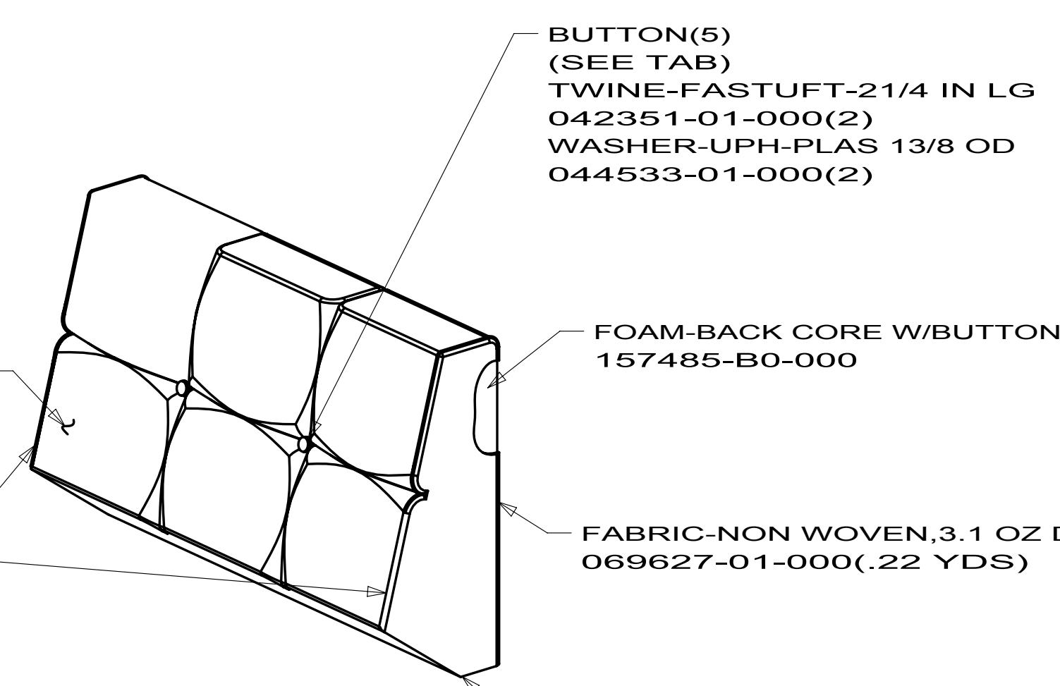
DETAIL B DINETTE-BACK ASM 171750-17 (2 REQ'D)
