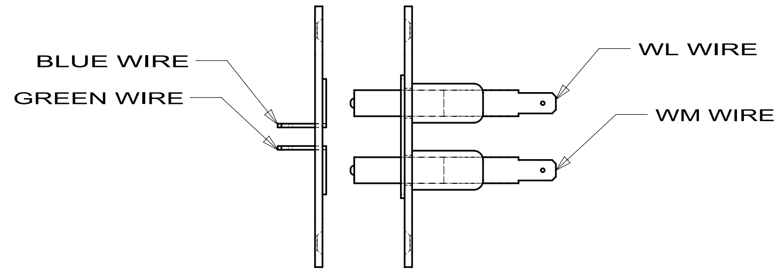
ELECTRIC LOCK CONTACT DETAIL
