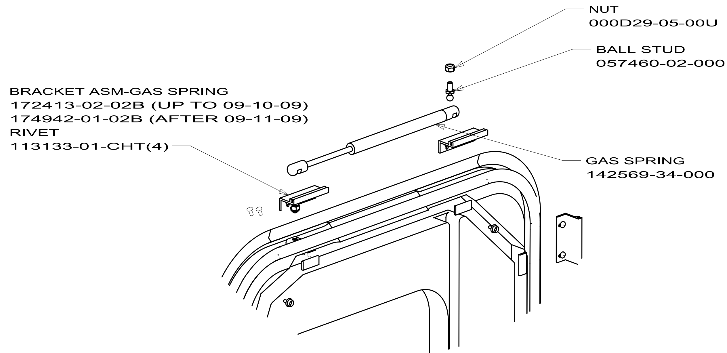
DETAIL CC
