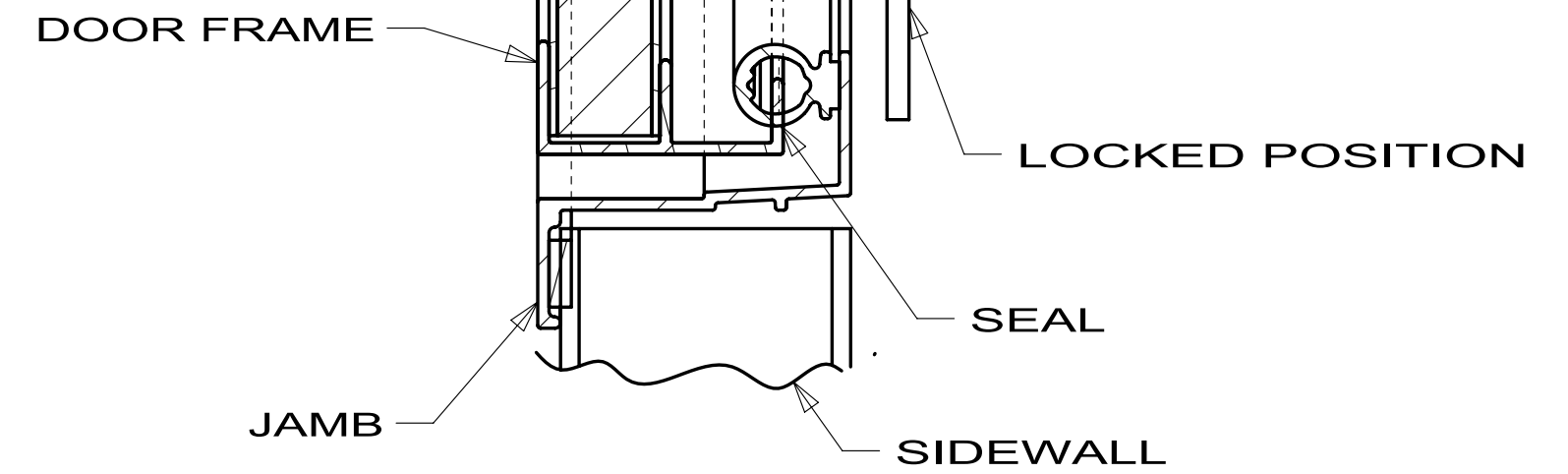
DETAIL V
