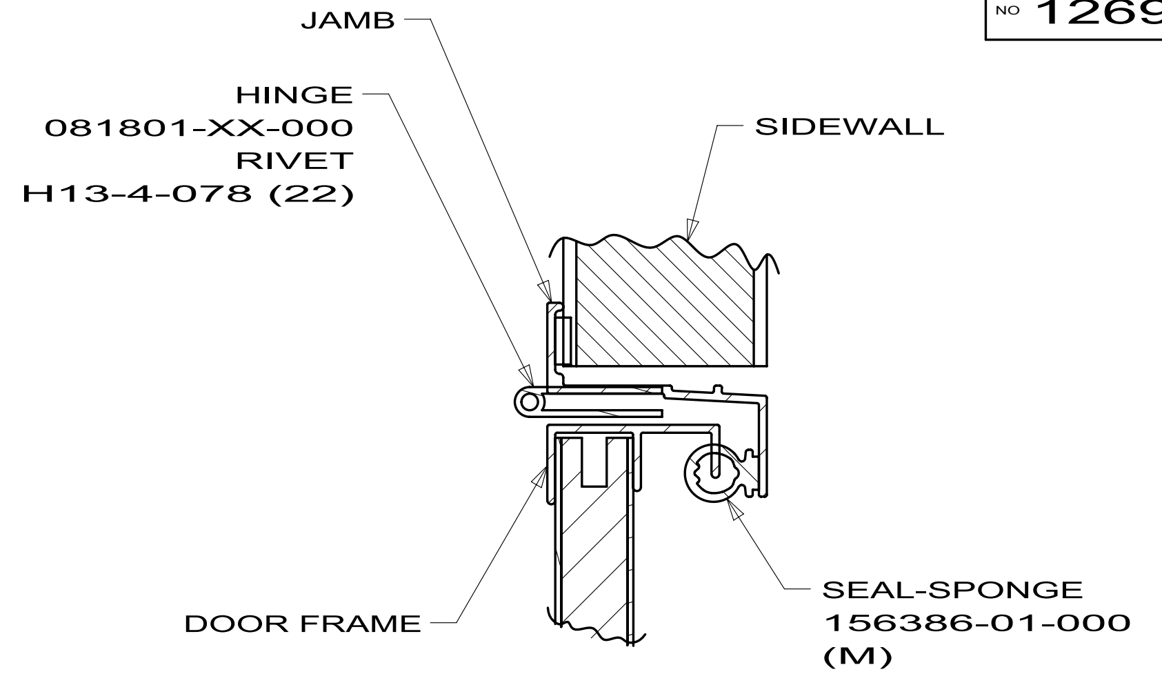
DETAIL Z
