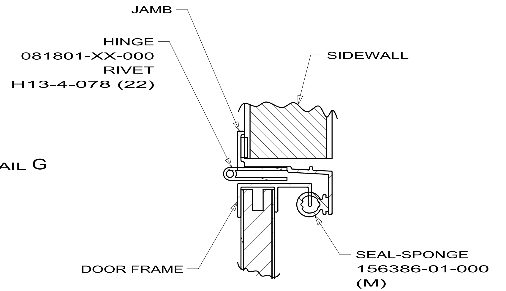
DETAIL G
