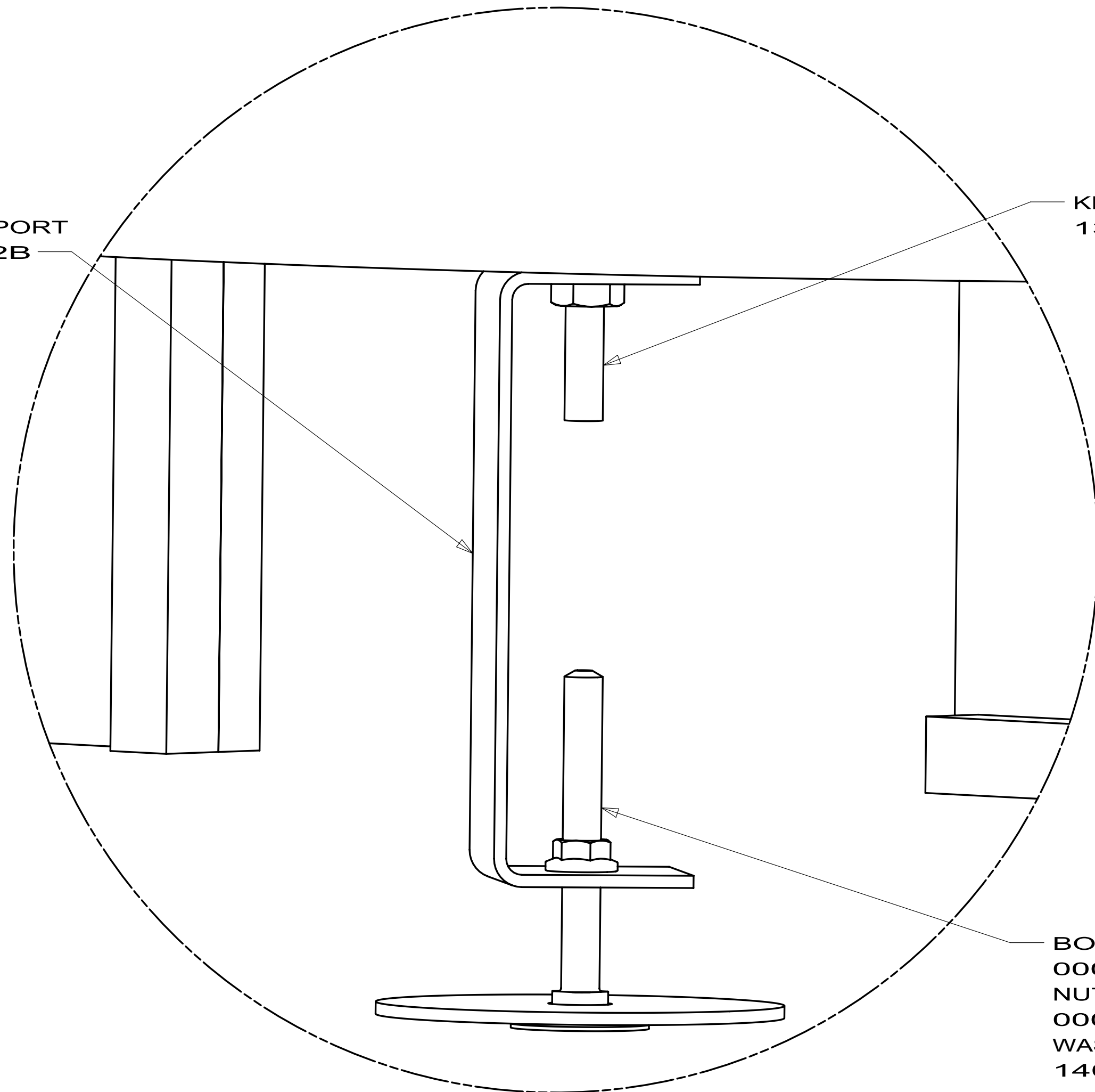
DETAIL A (SHOWN W/OUT CABINET ASM-PIPE COVER)
