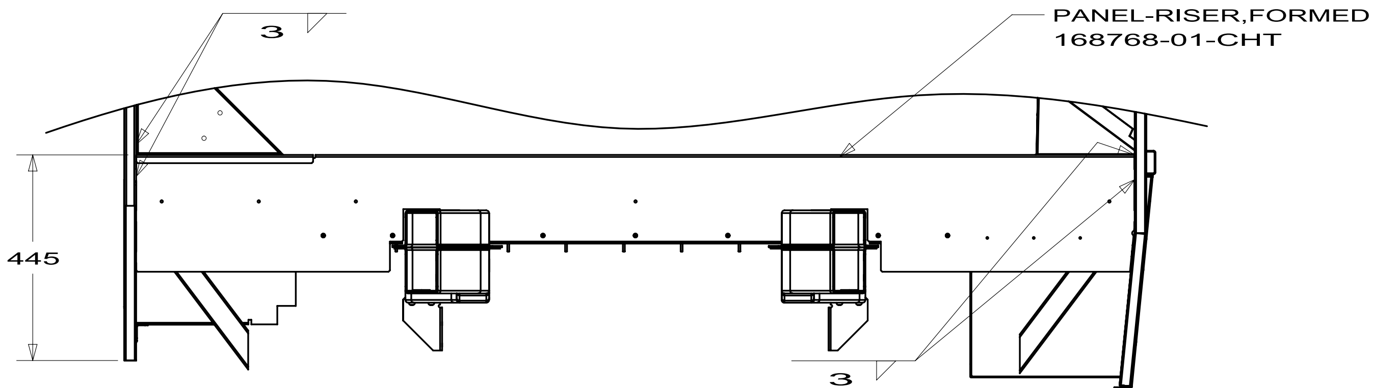
VIEW BB
