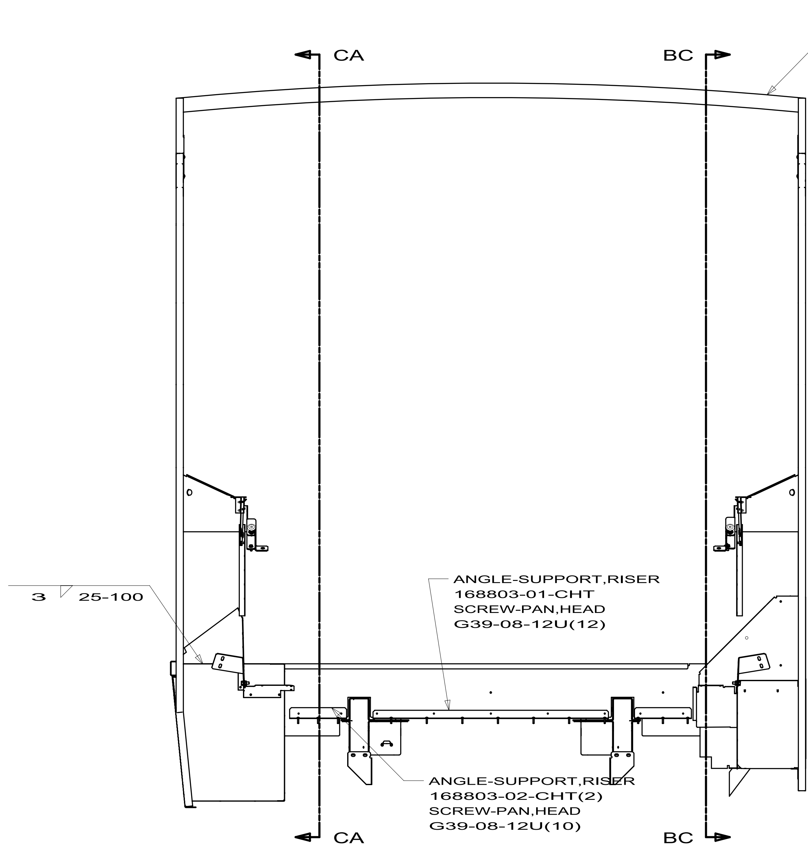
VIEW BA
