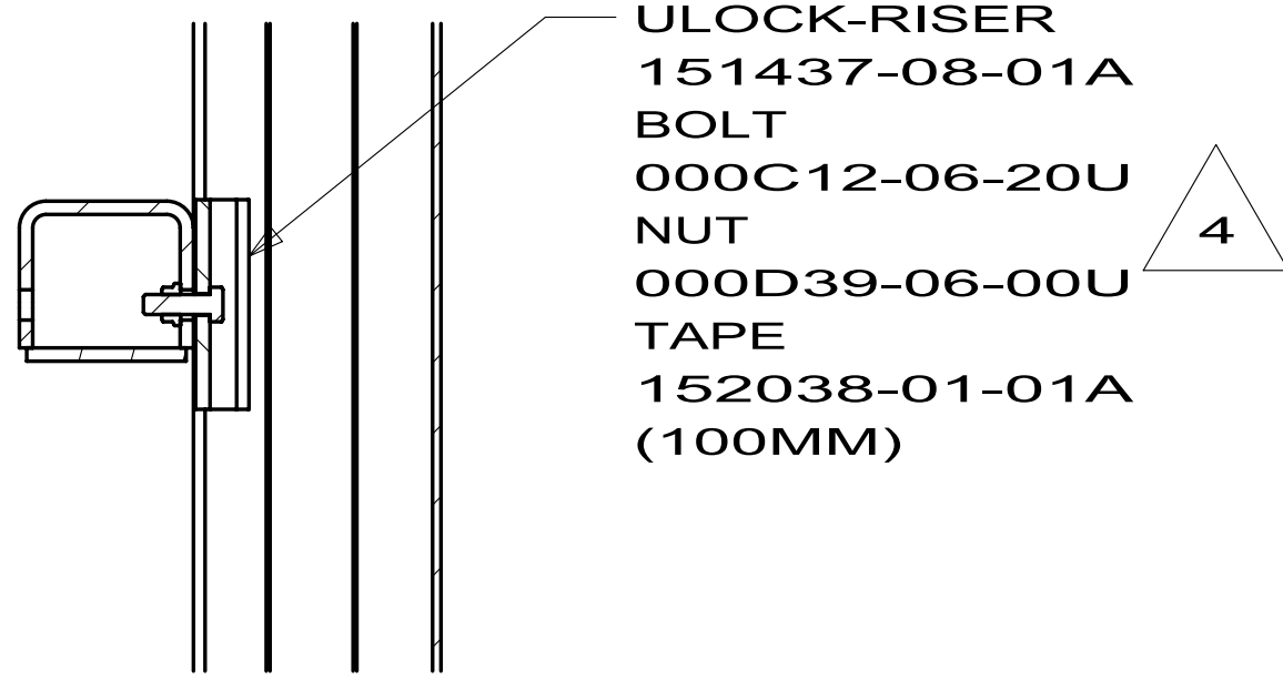
SECTION FA-FA
