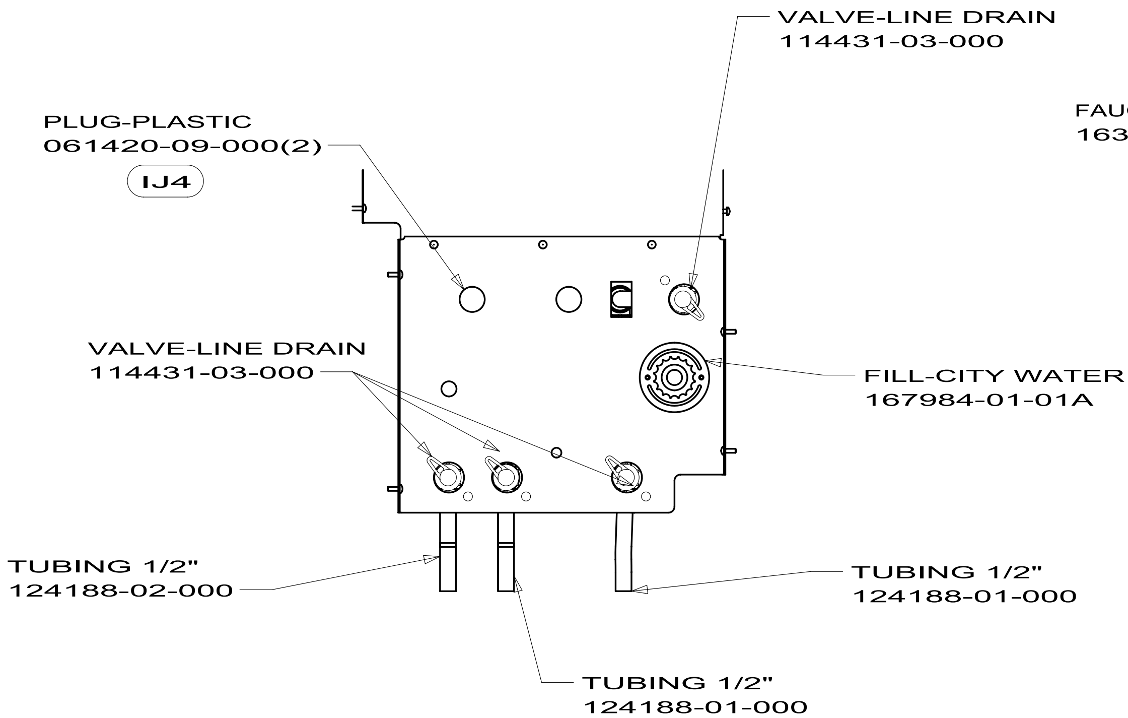
VIEW EA (EXTERIOR SHOWER WITHOUT SHOWN)
