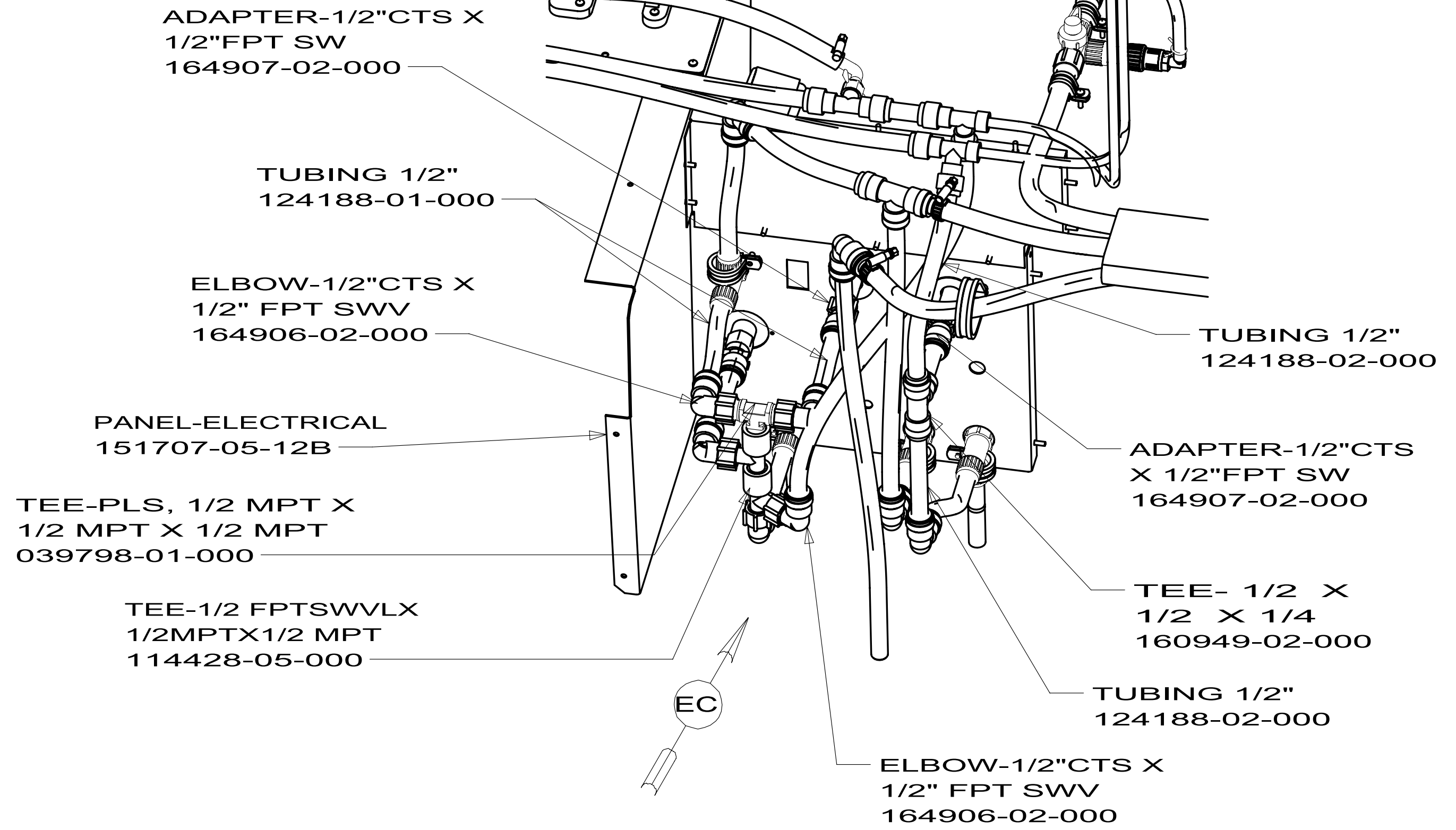
VIEW EB (EXTERIOR SHOWER SHOWN)
