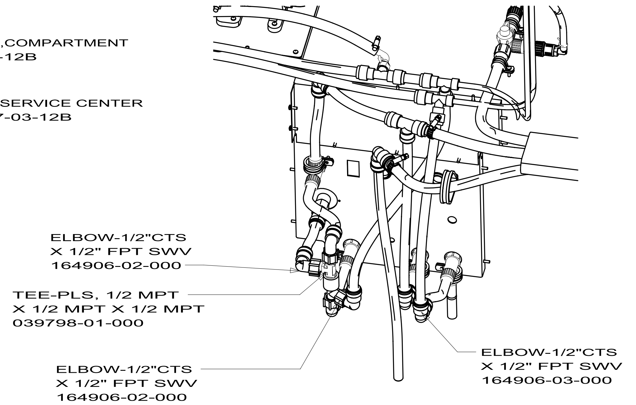
VIEW EB (EXTERIOR SHOWER WITHOUT SHOWN)
