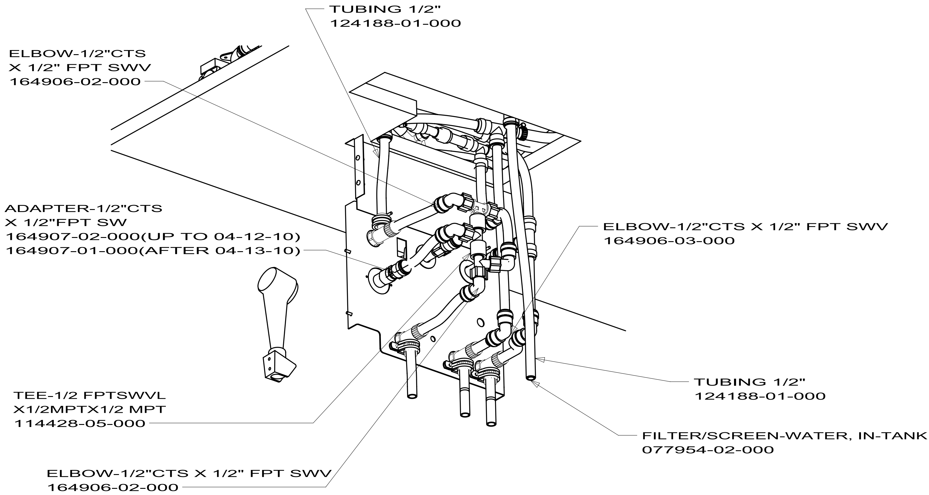
VIEW EC (EXTERIOR SHOWER SHOWN)
