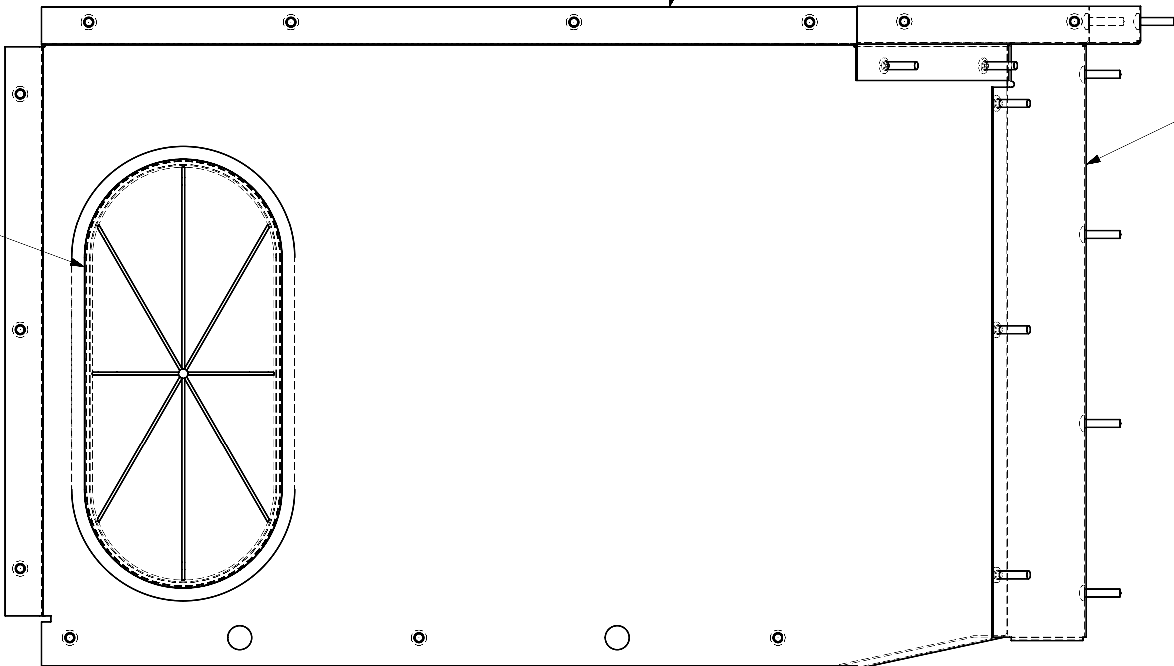
SECTION BA-BA
