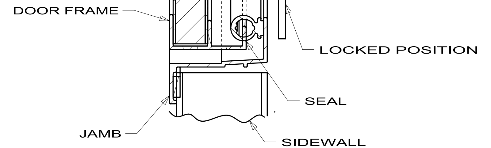
DETAIL V
