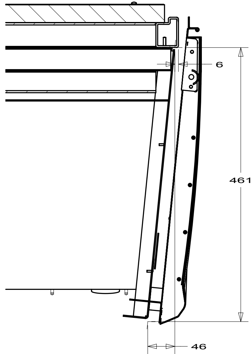
SECTION BH-BH
