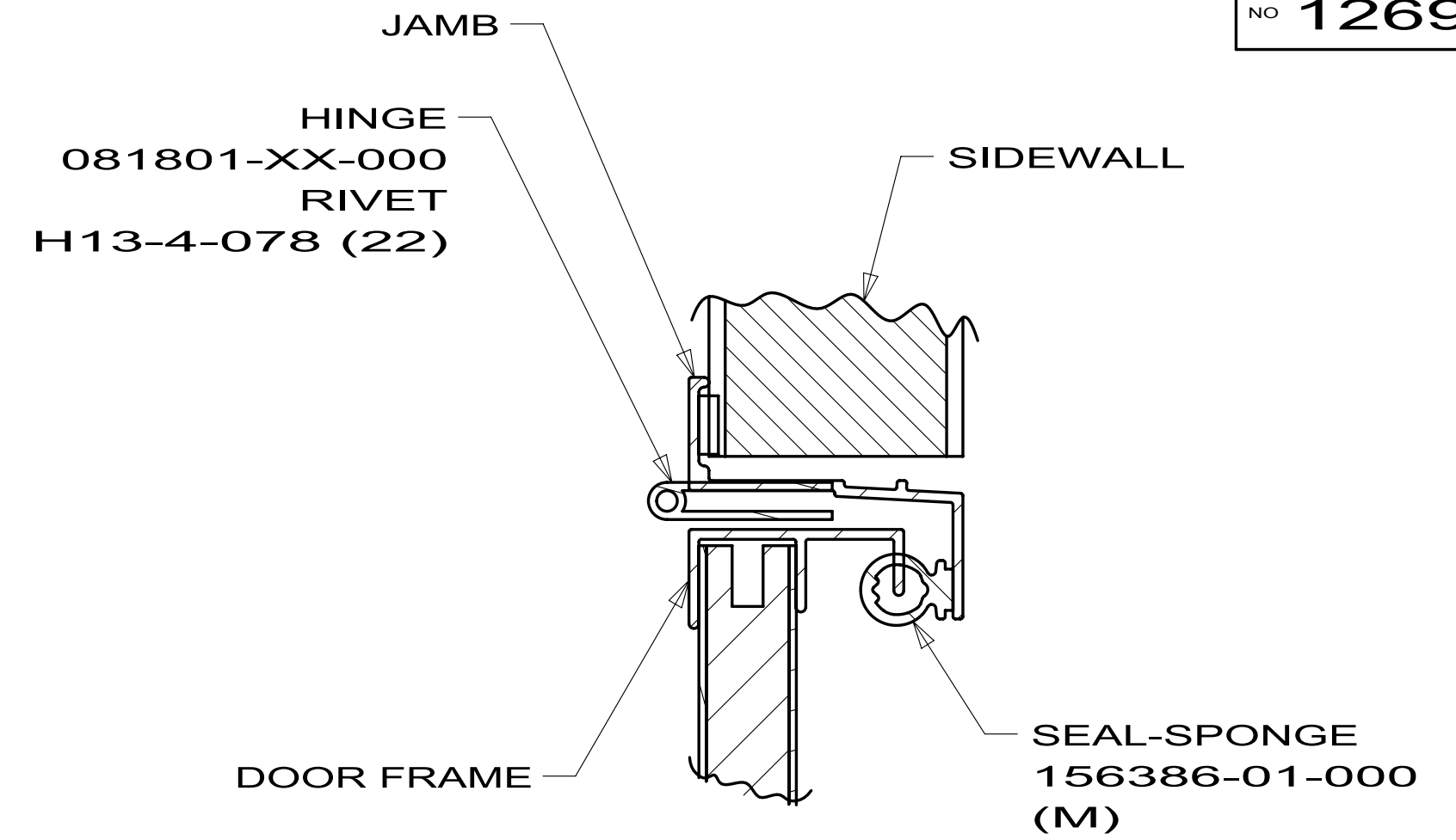
DETAIL Z
