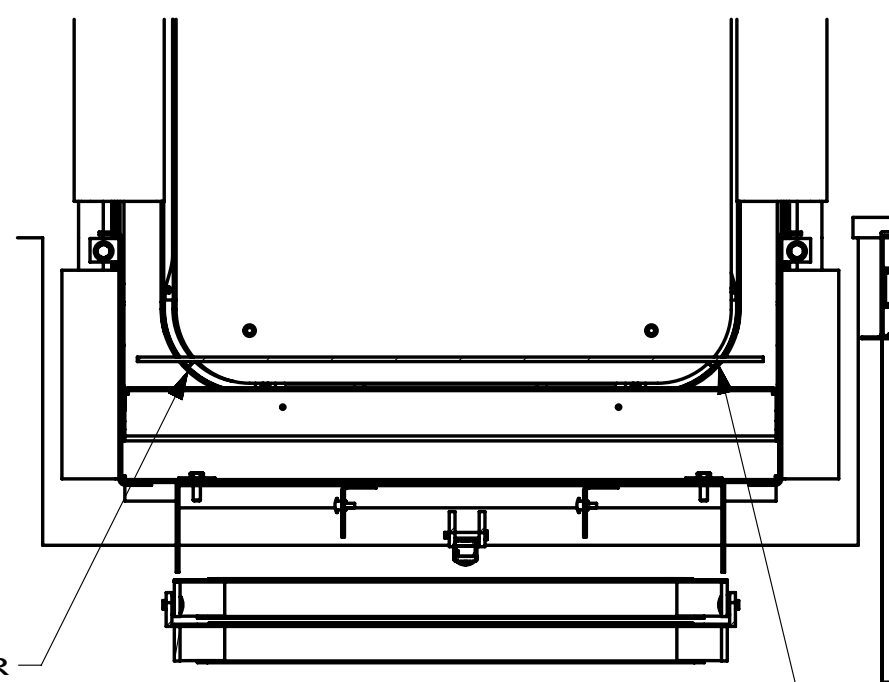
SECTION BB-BB
