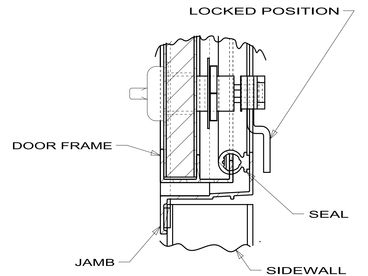
DETAIL F
