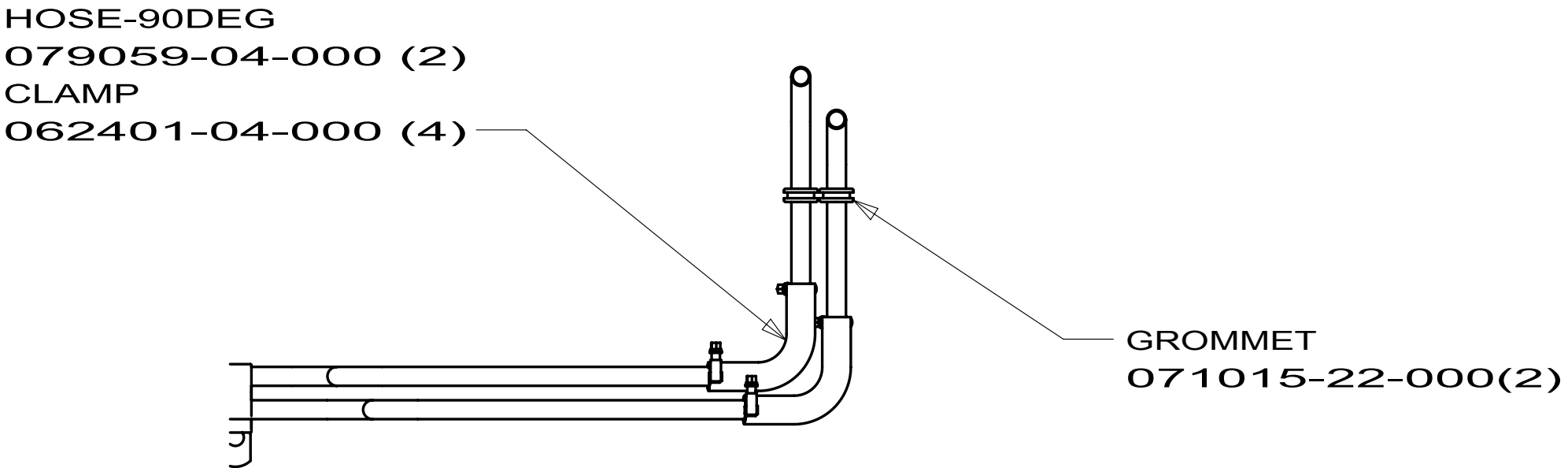
SECTION BA-BA
