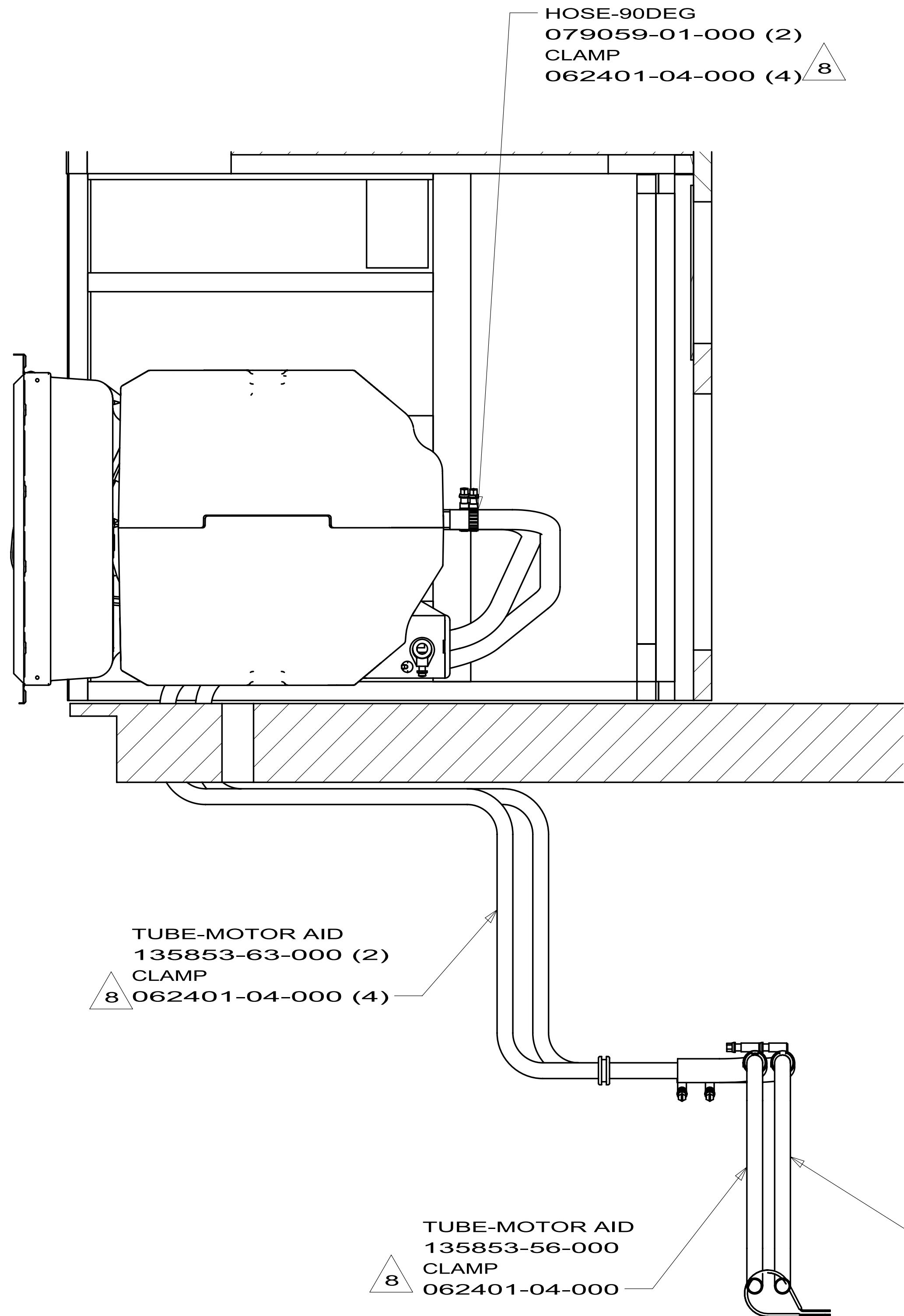
SECTION BB-BB (ROTATED)
