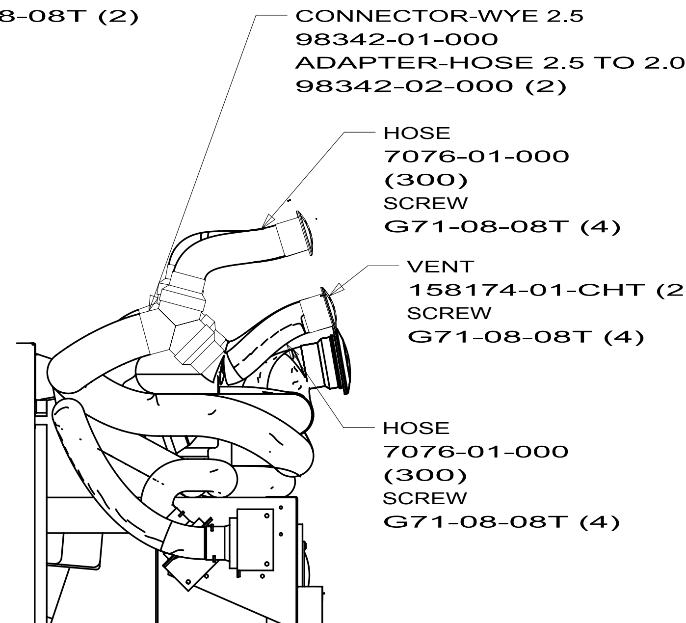
SECTION AC-AC (2 PLACES)
