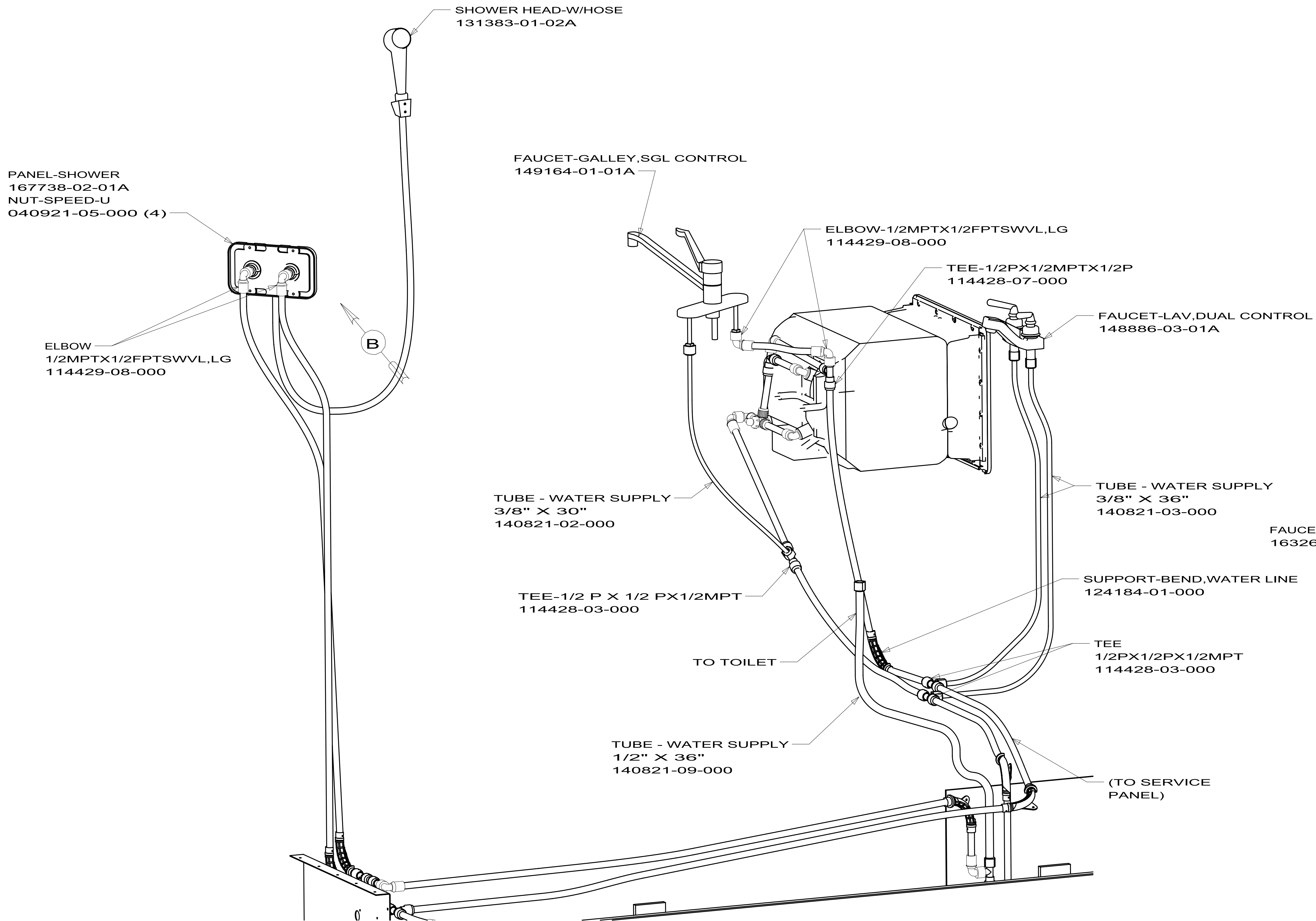
VIEW A
