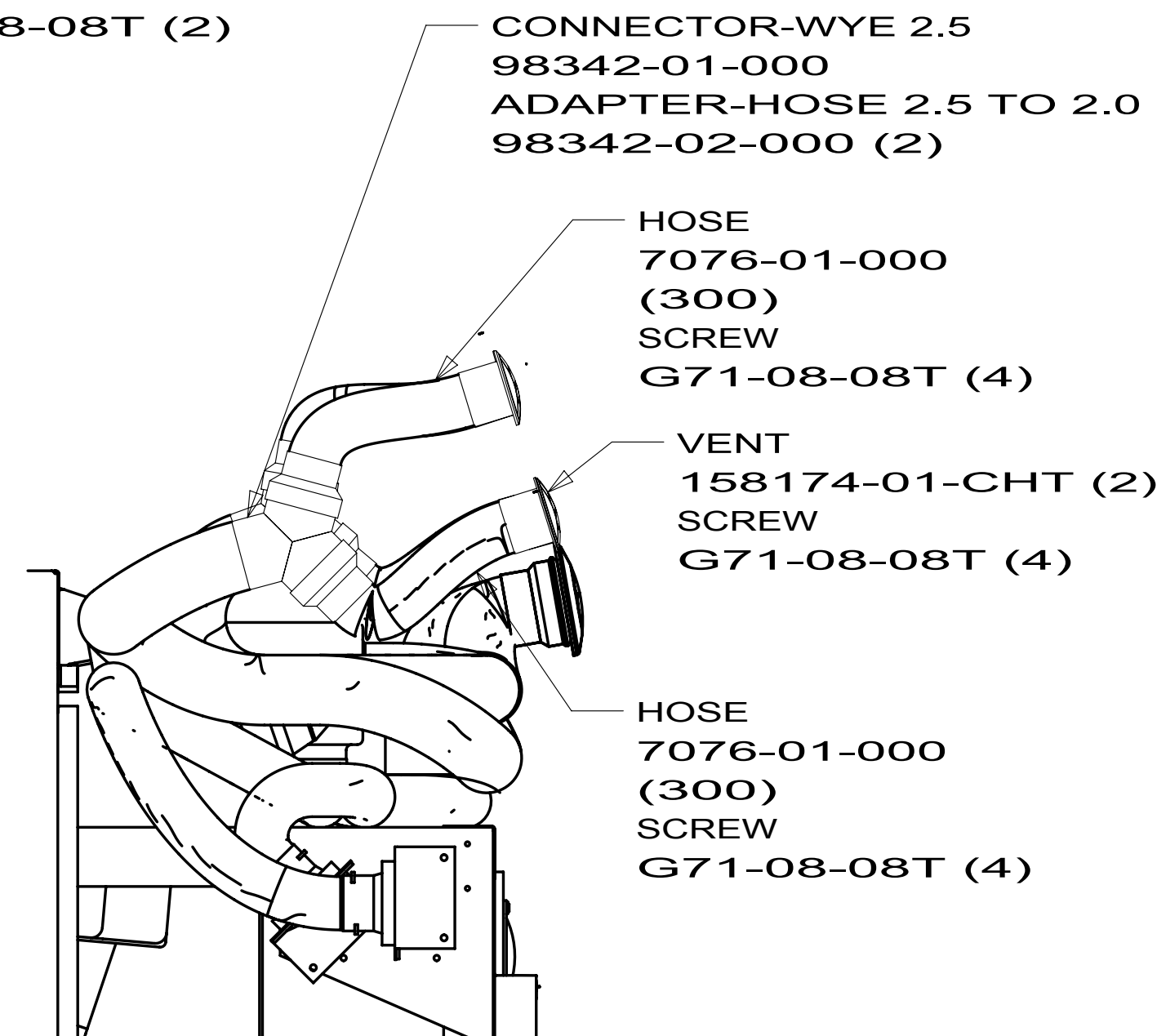
SECTION AC-AC (2 PLACES)
