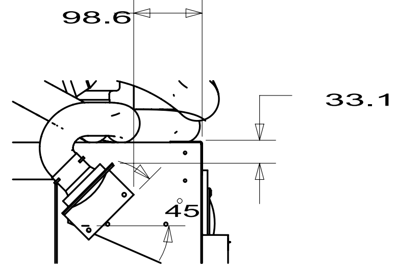
SECTION AB-AB
