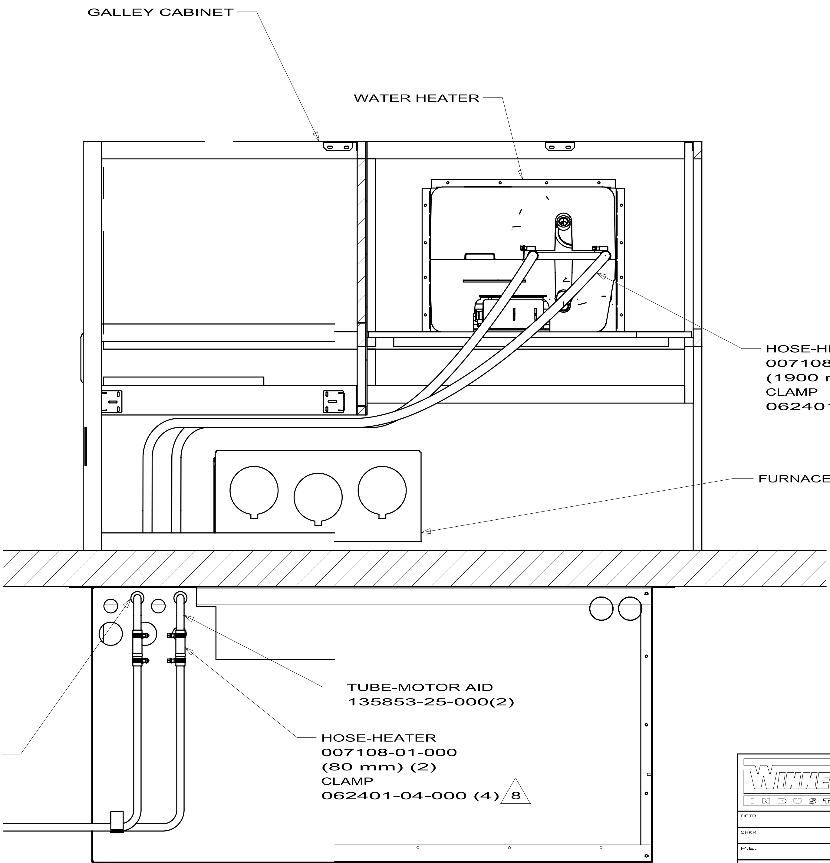
SECTION BA-BA
