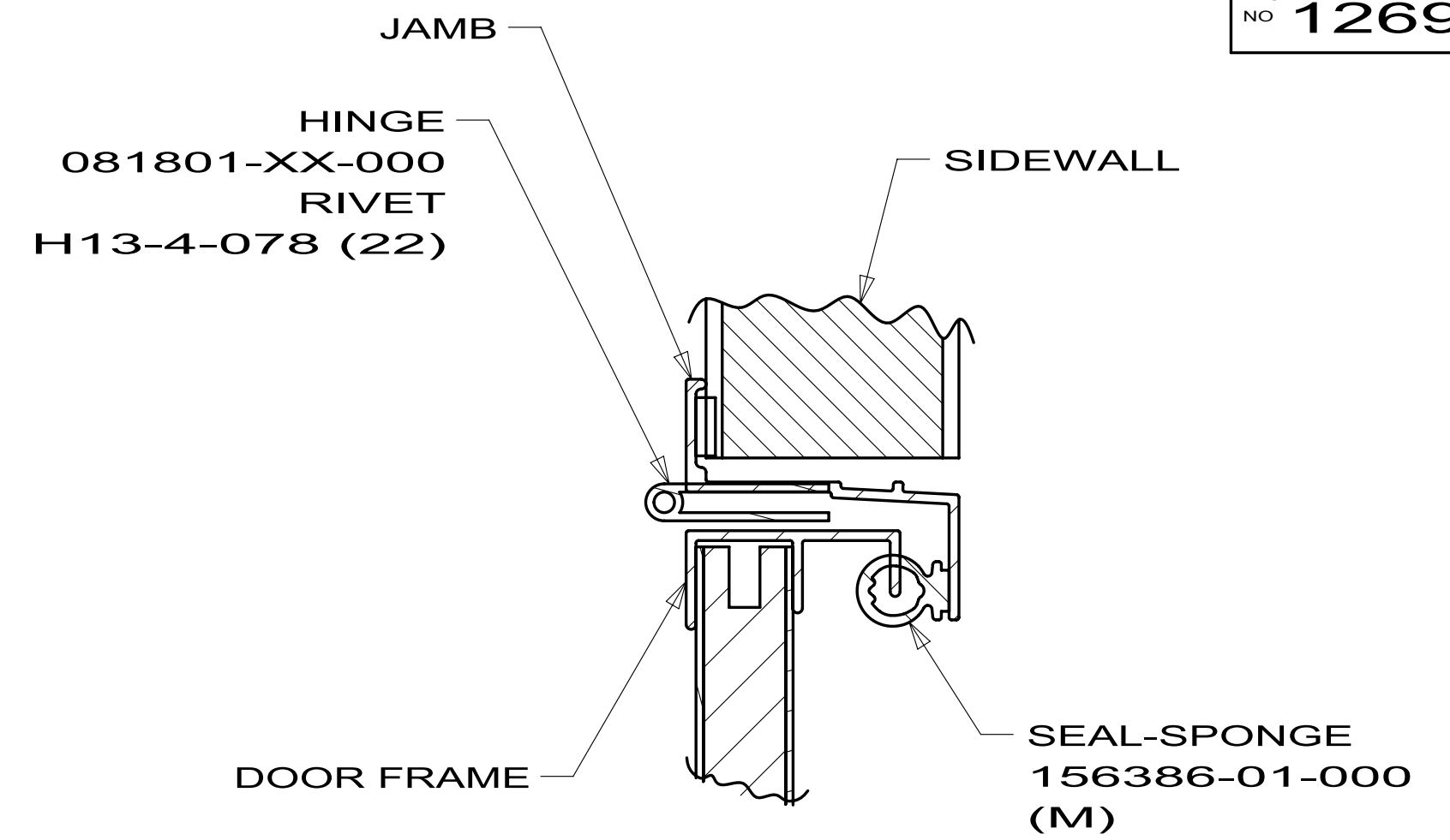
DETAIL Z
