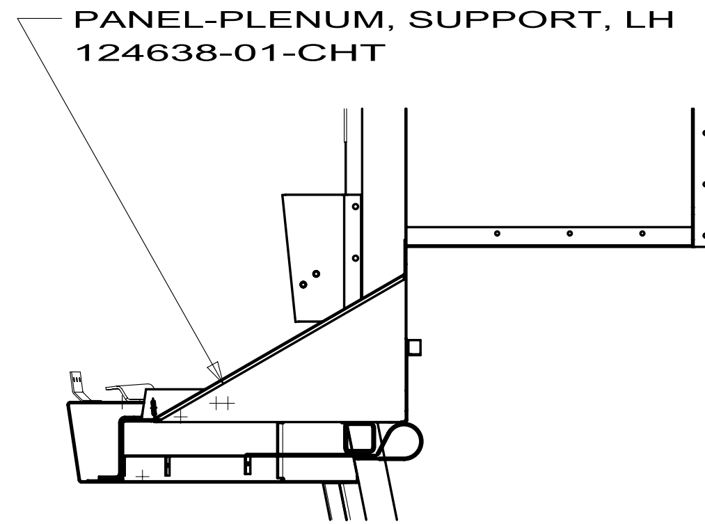
SECTION HB-HB
