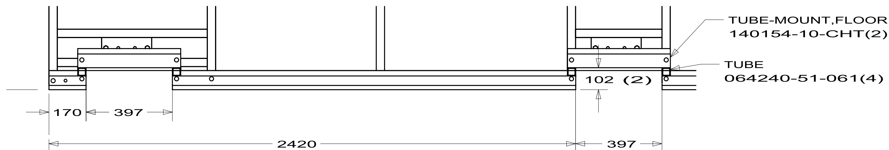
VIEW HL-HL
