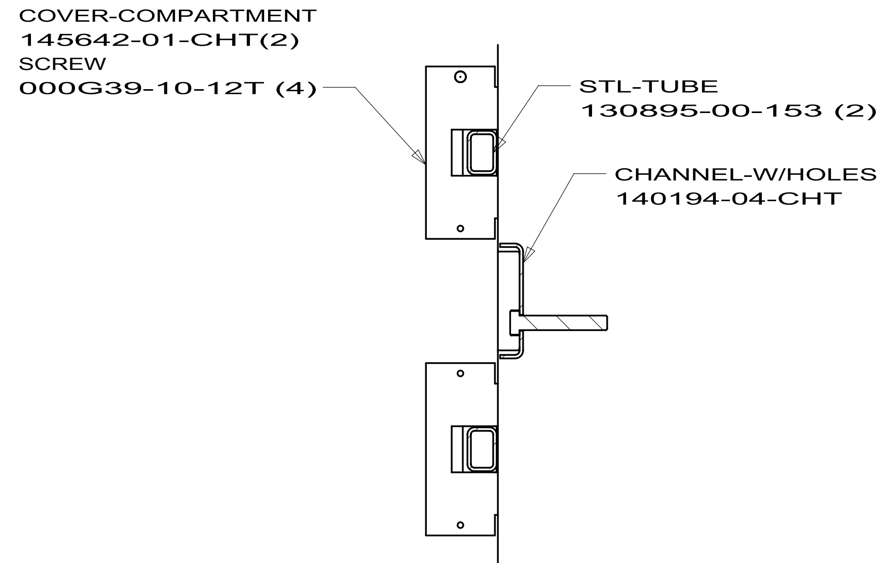
SECTION HH-HH
