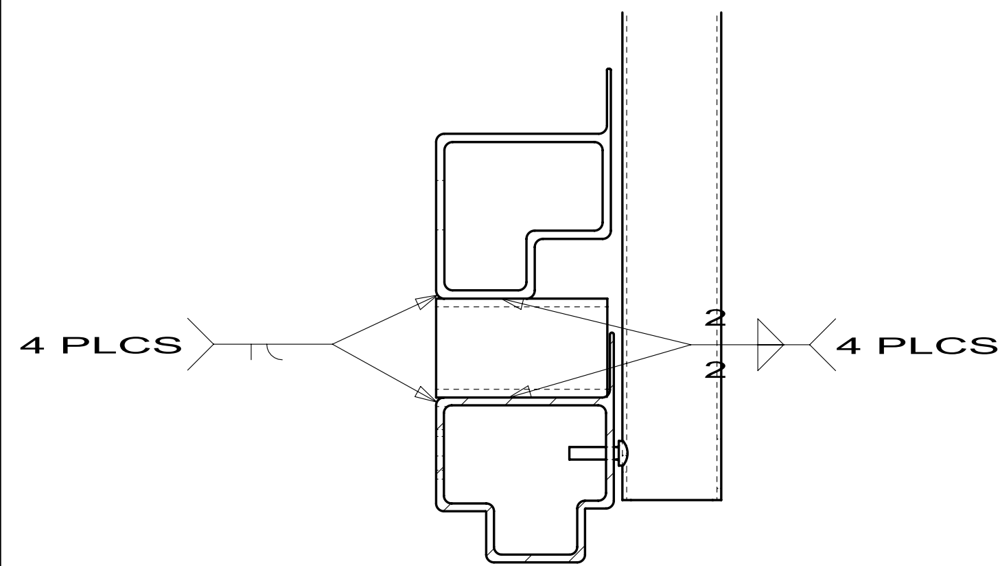
SECTION HA-HA
