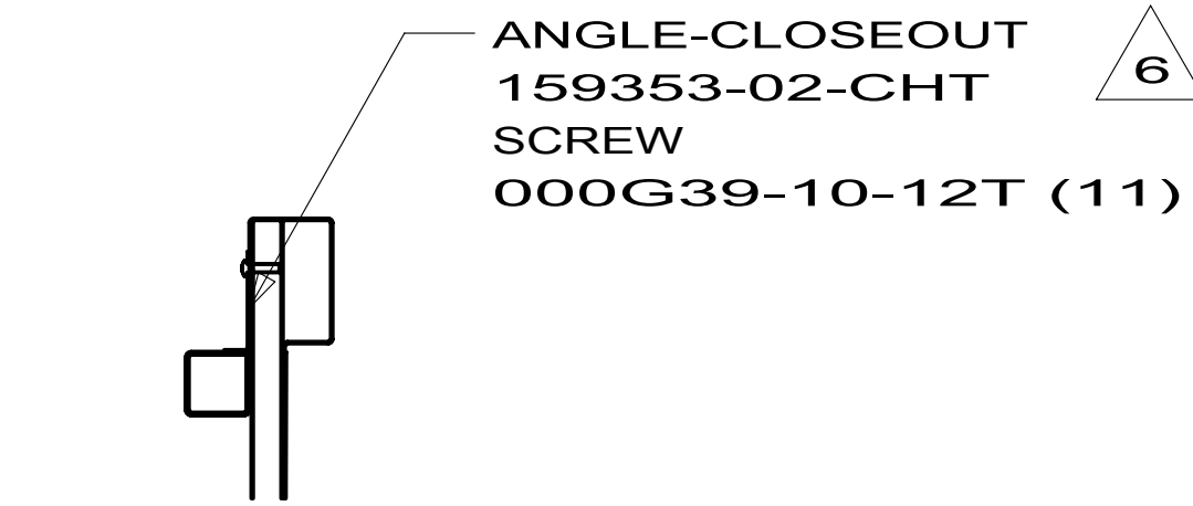
SECTION KB-KB
