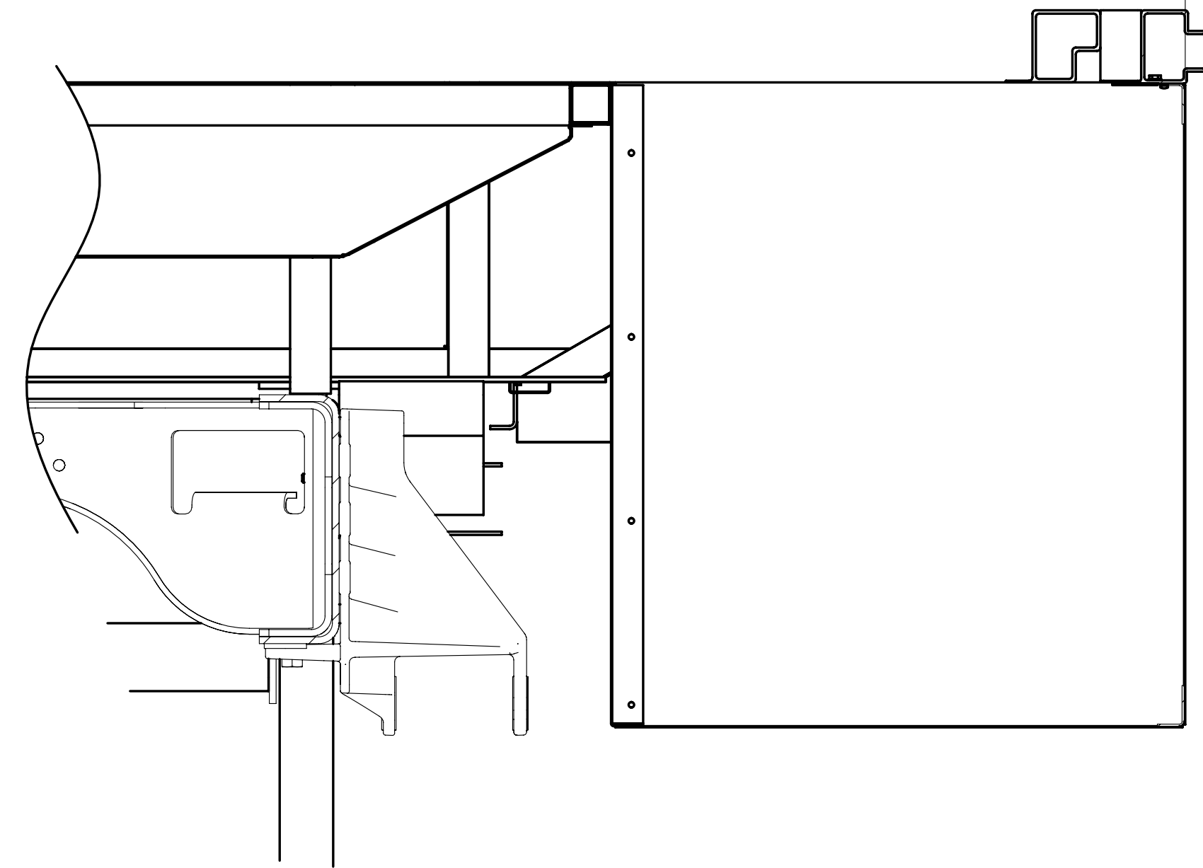
SECTION KC-KC
