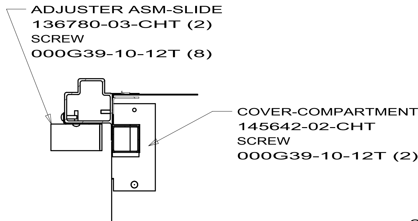
SECTION HF-HF
