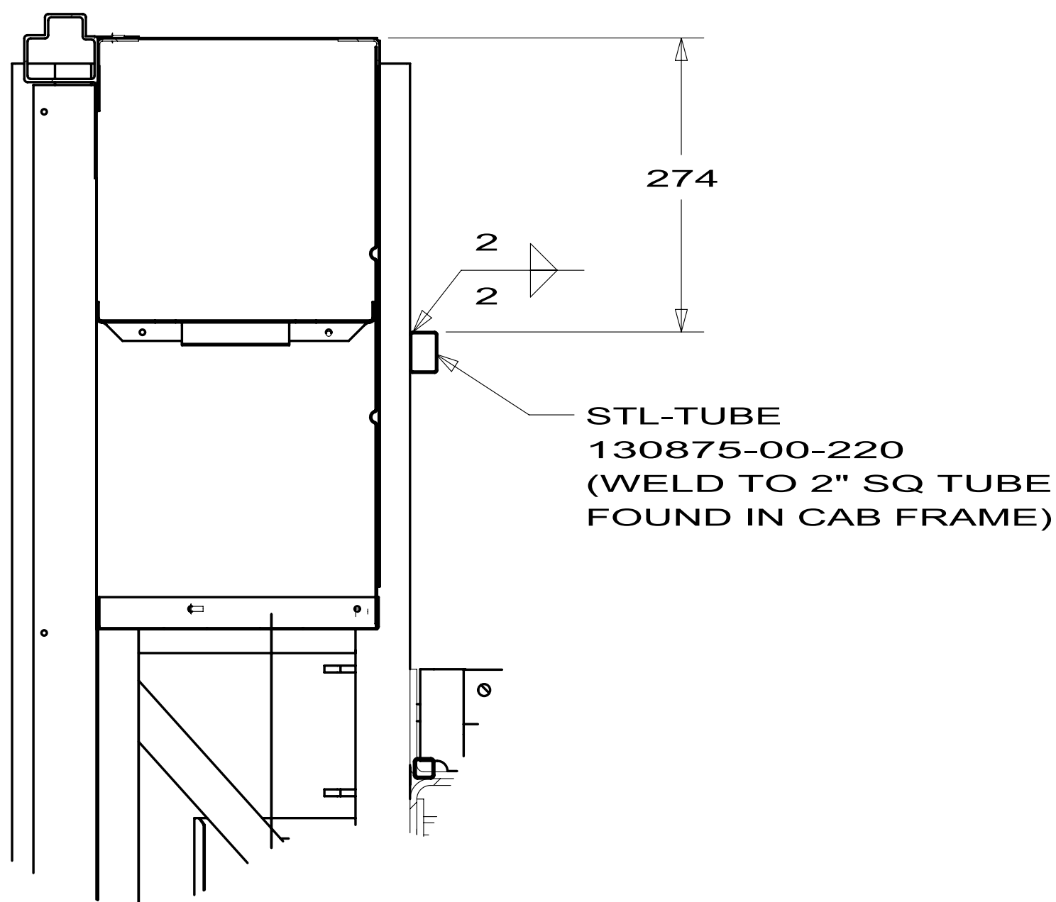
SECTION KD-KD
