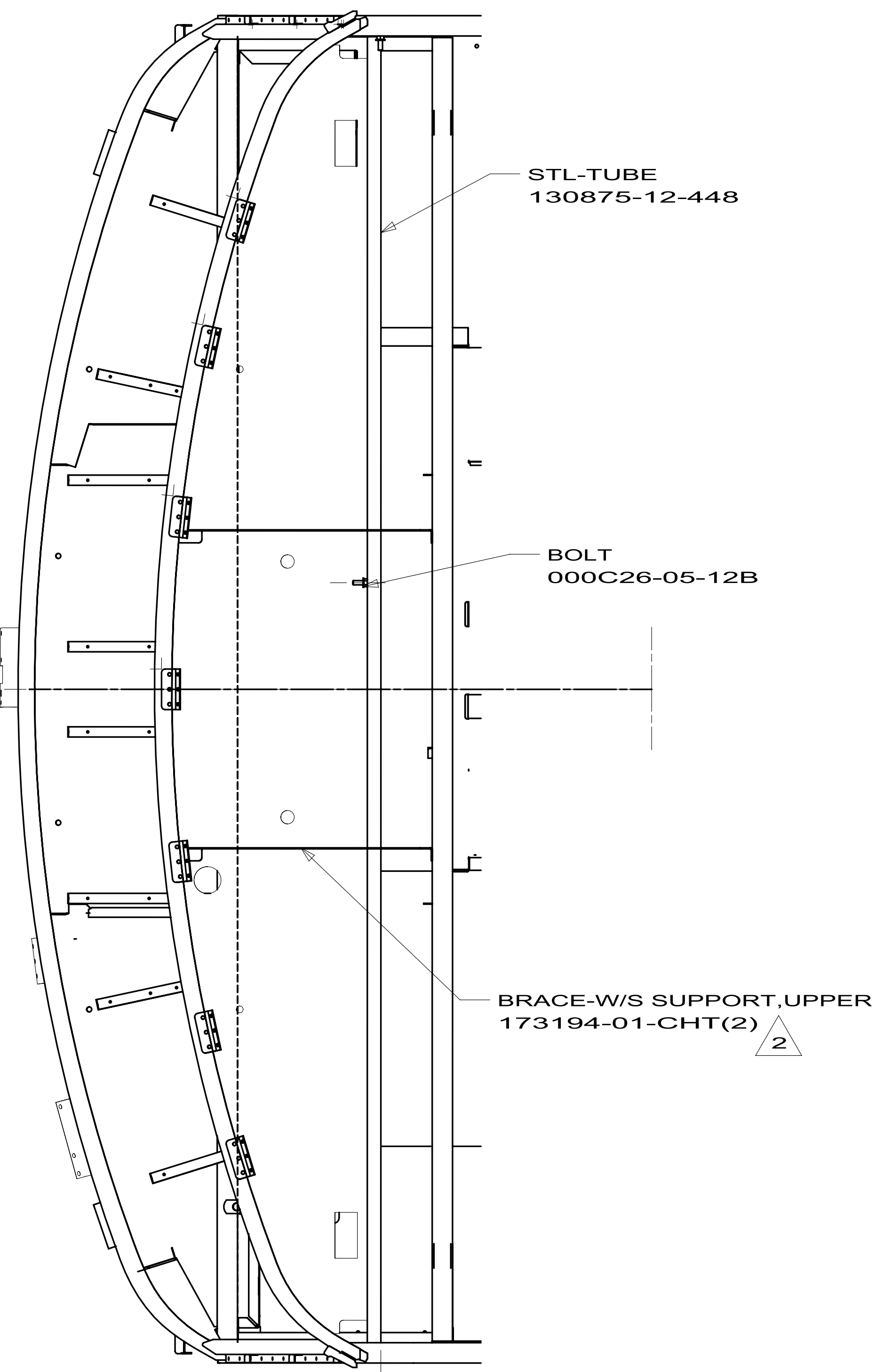
SECTION EB-EB
