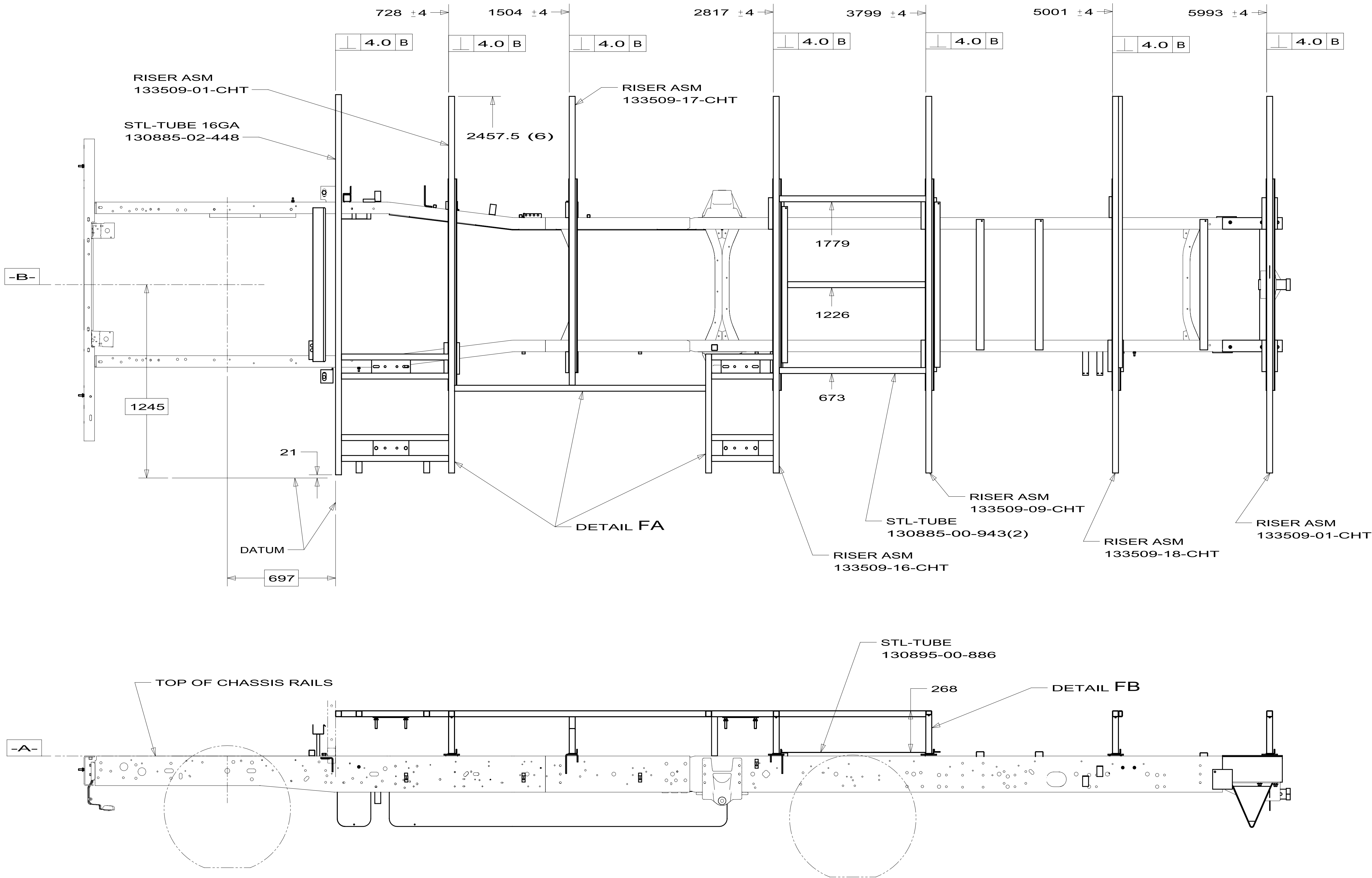
DETAIL EA FLOOR FRAME ASM 171767-12
