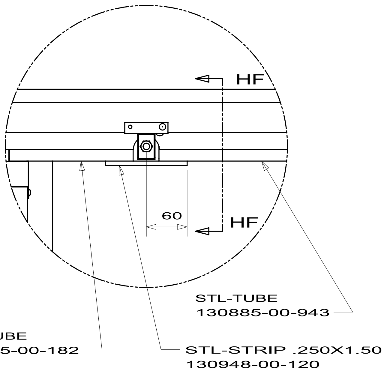
DETAIL HE
