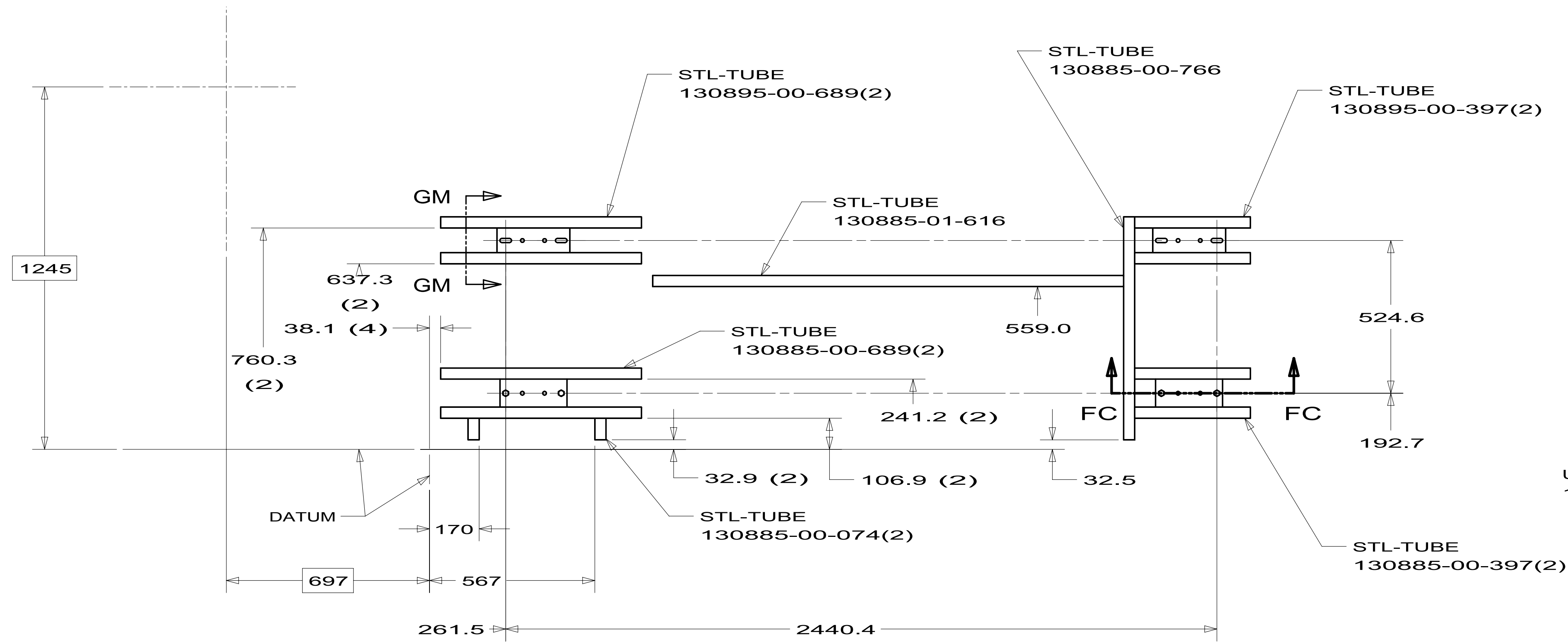
DETAIL FA FLOOR FRAME ASM 171767-13
