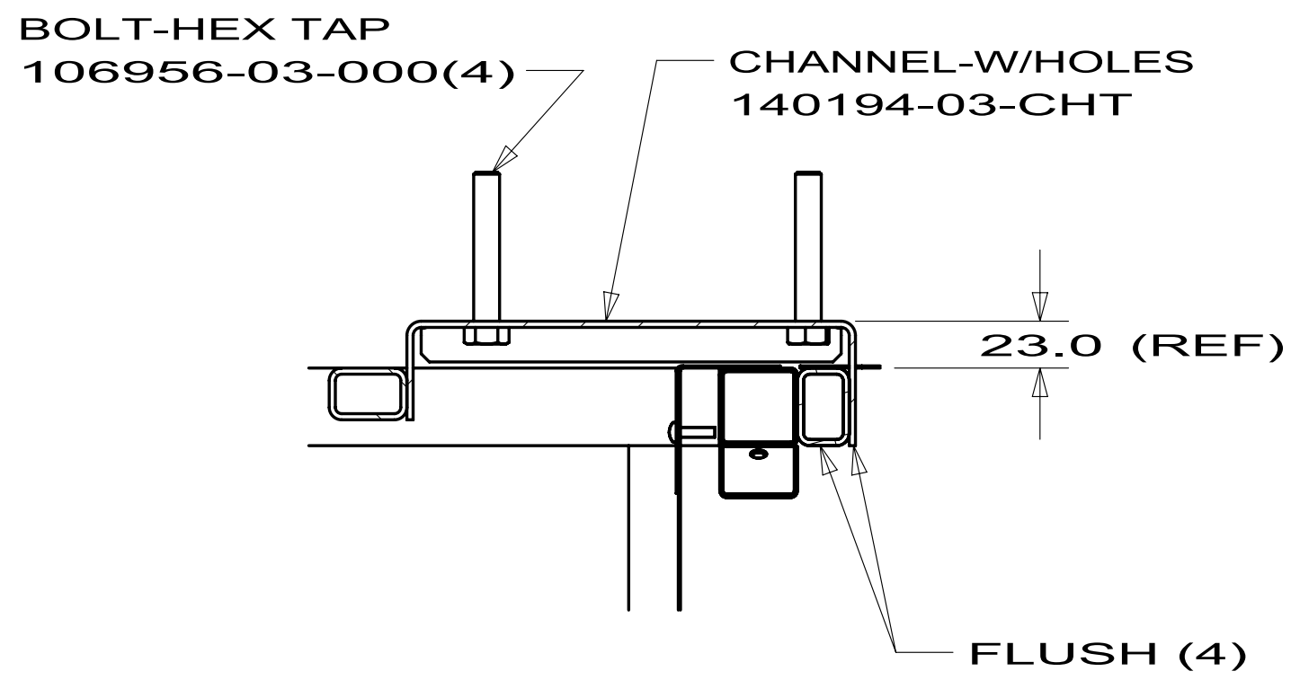
SECTION HK-HK
