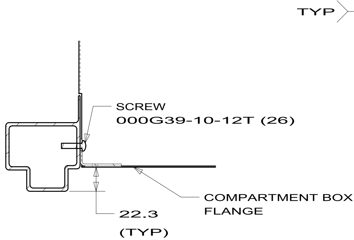
SECTION HB-HB
