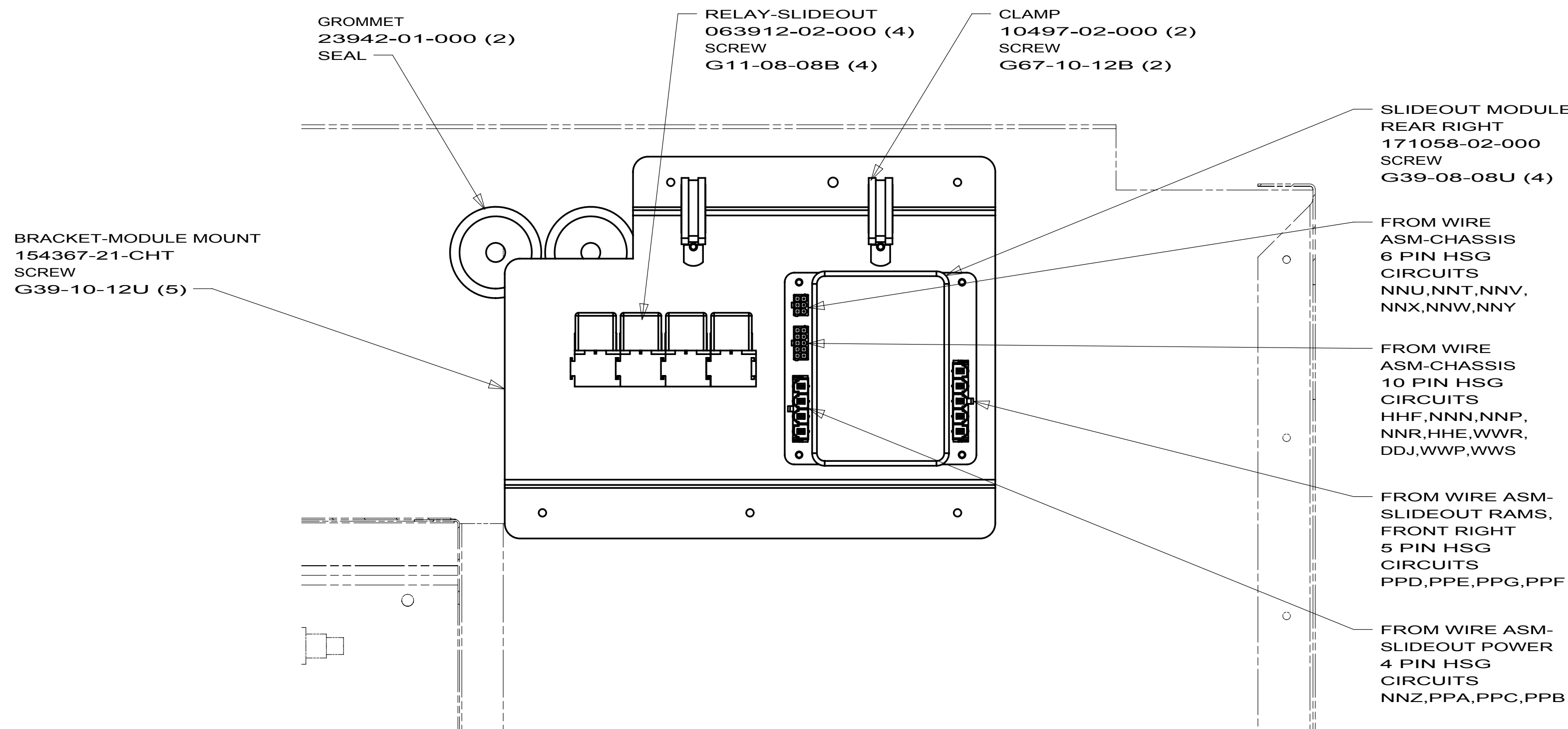
SECTION EA-EA
