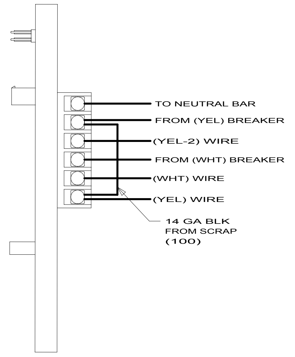
DETAIL CA 53Z
