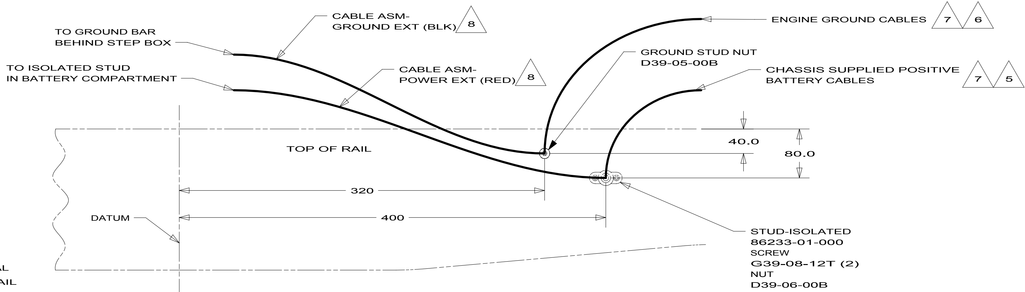
VIEW DC 16L
