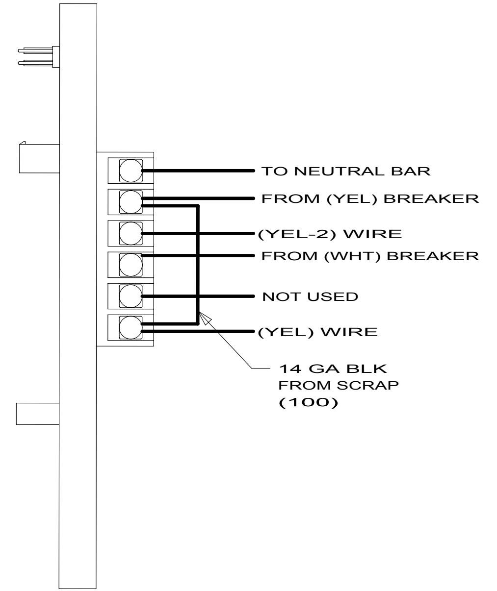
DETAIL CA 9
