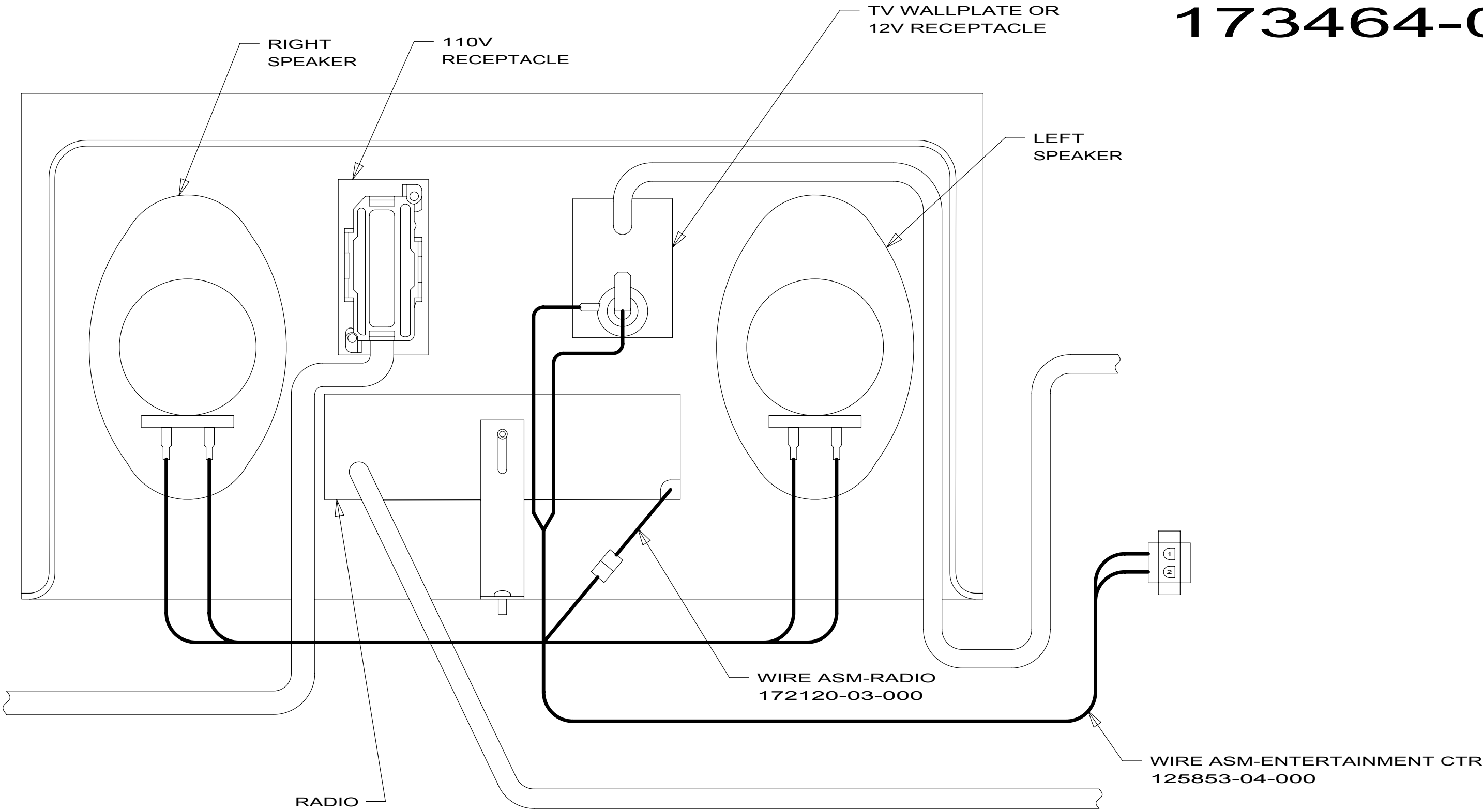
DETAIL EC 173464-03 173464-07 173464-08
