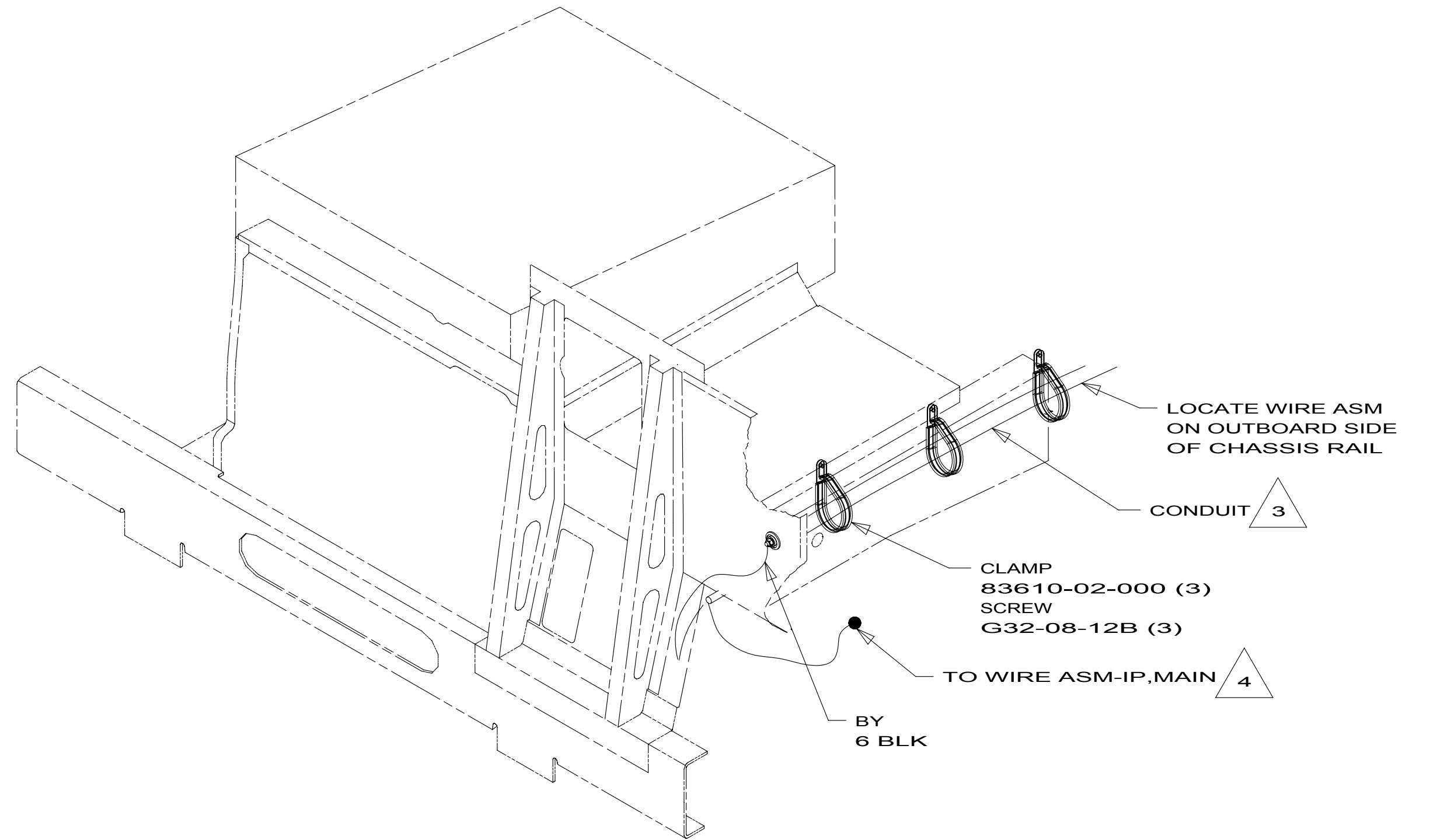
VIEW DB 16L
