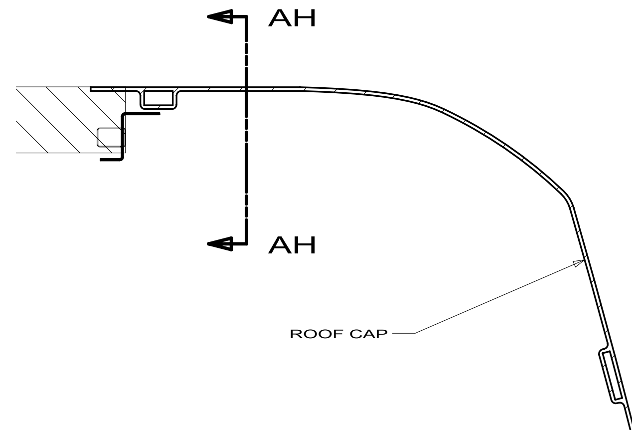
SECTION AC-AC
