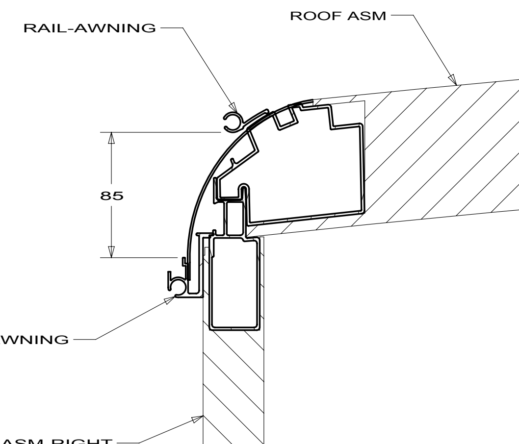
SECTION AL-AL
