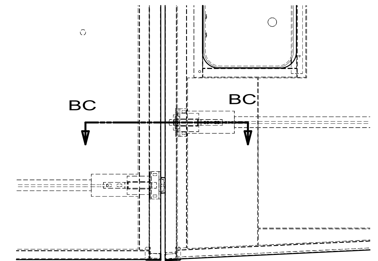
DETAIL BB
