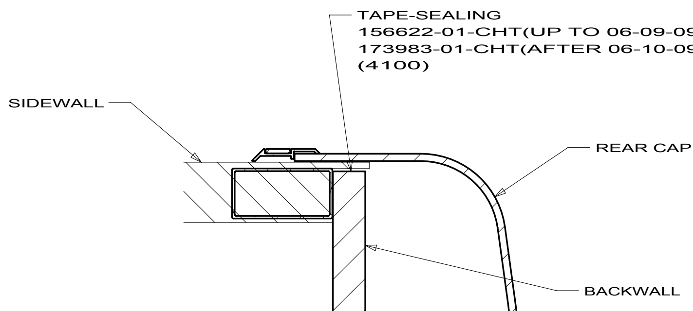
SECTION AE-AE
