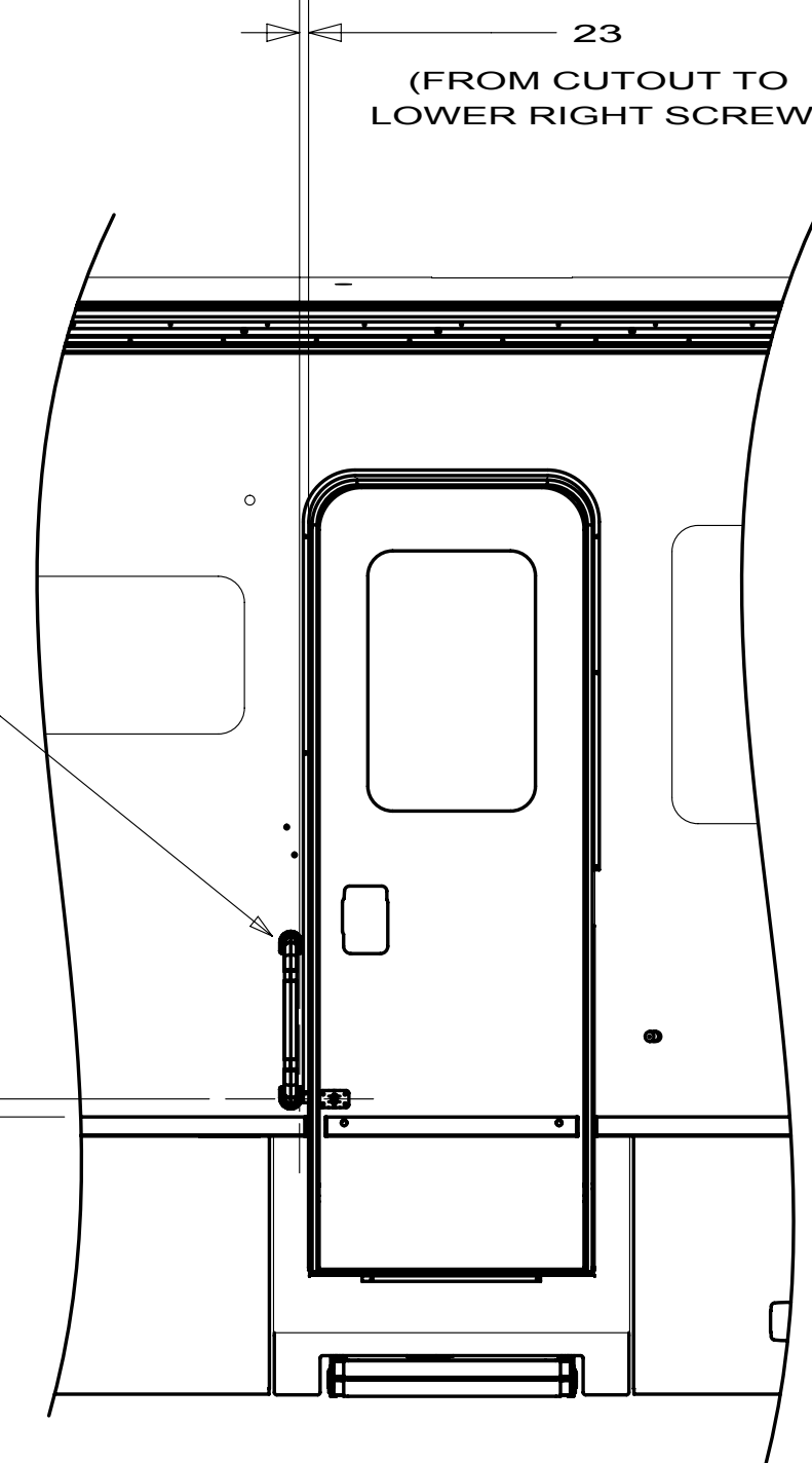
DETAIL AG
