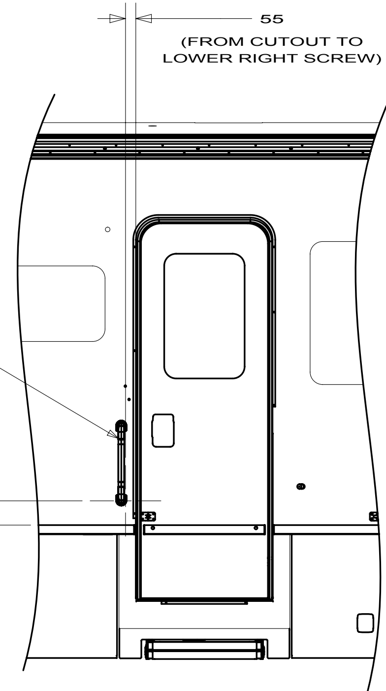
DETAIL AG
