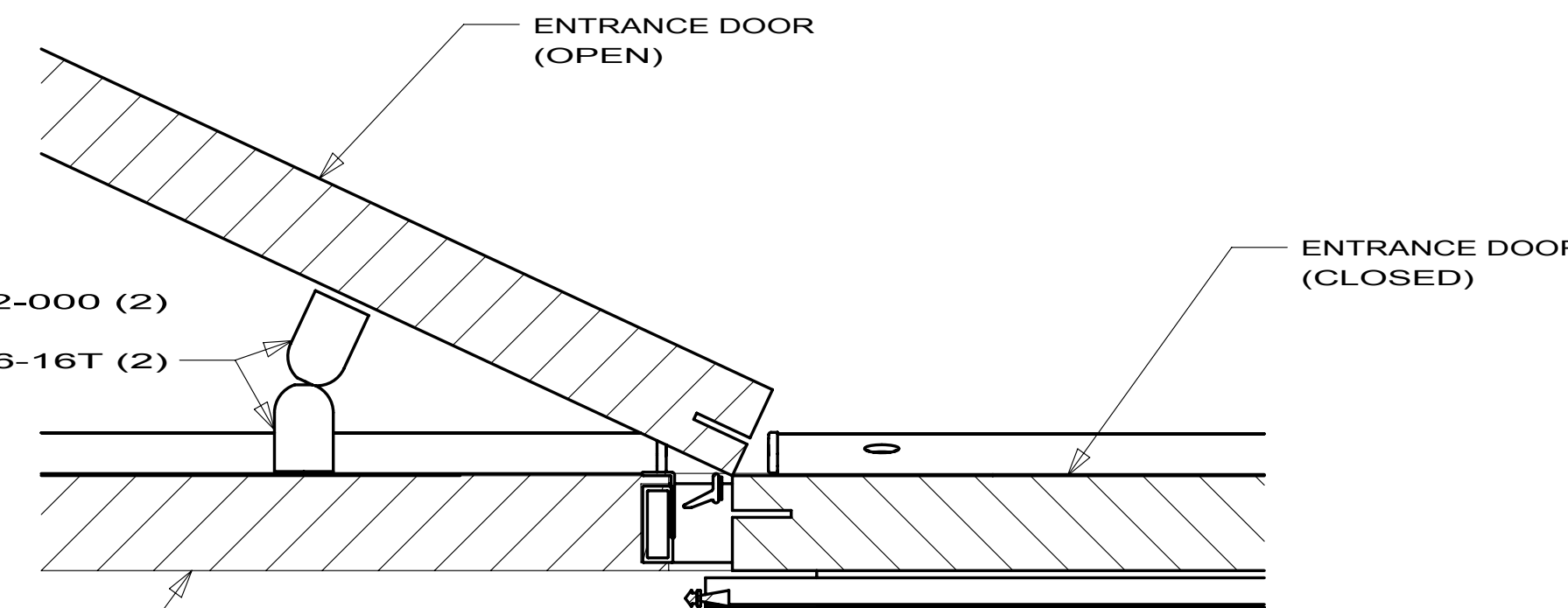
SECTION BA-BA
