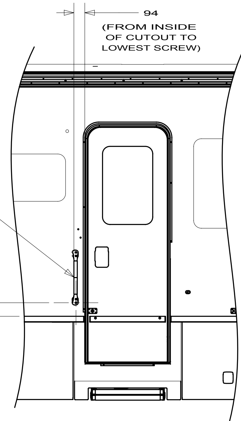
DETAIL AG
