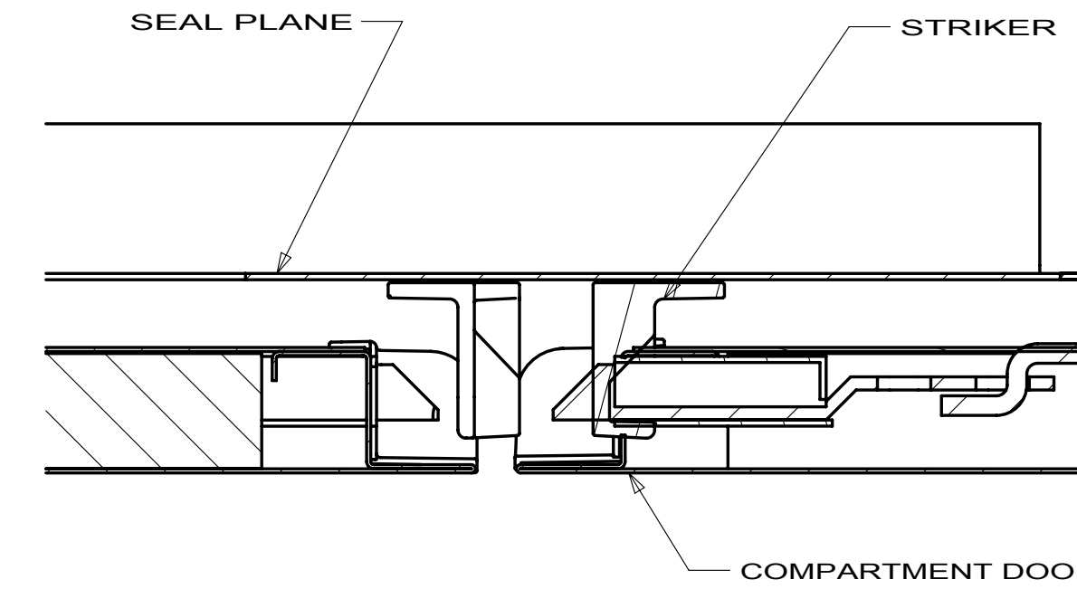
SECTION BC-BC
