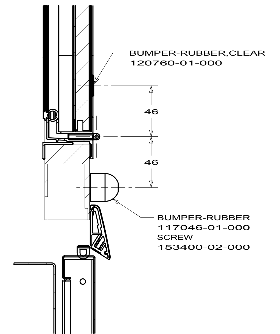
SECTION BD-BD
