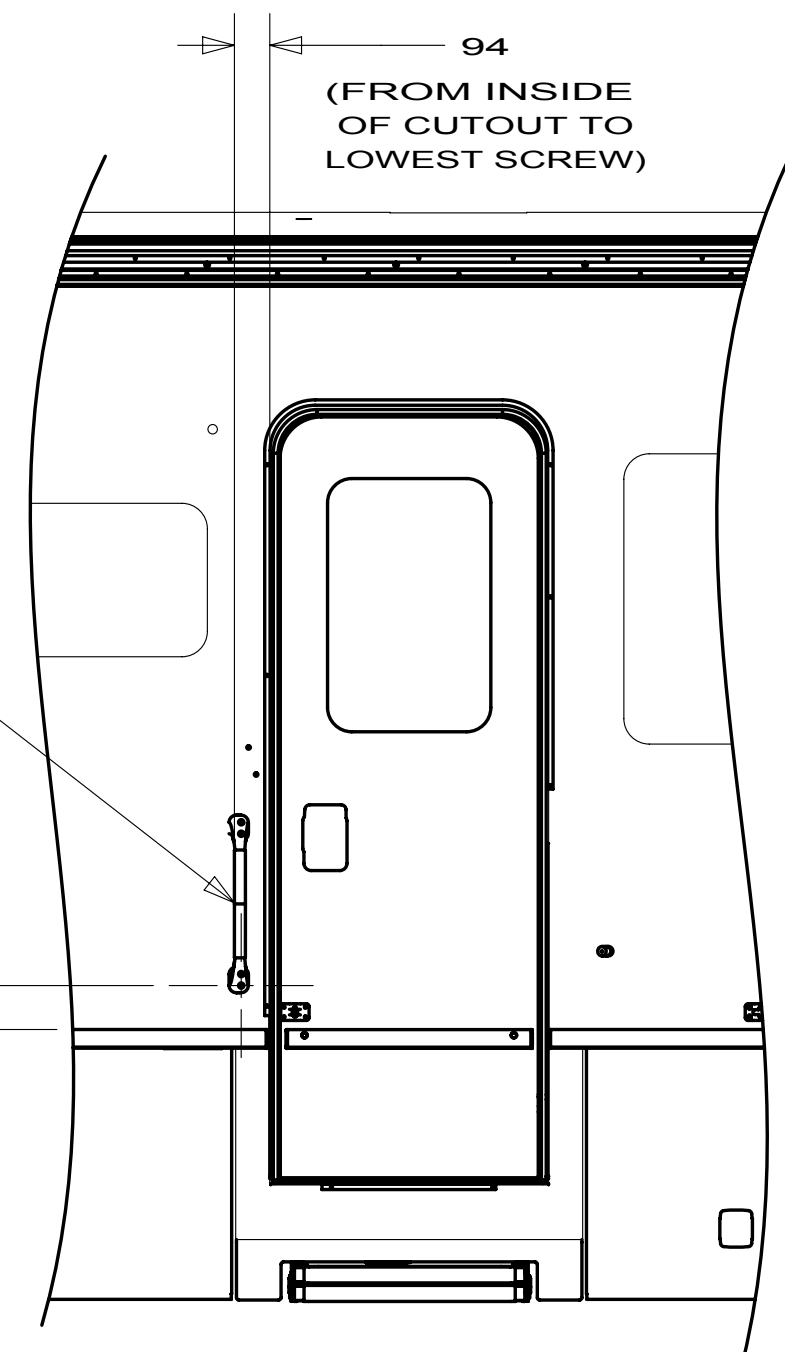
DETAIL AG
