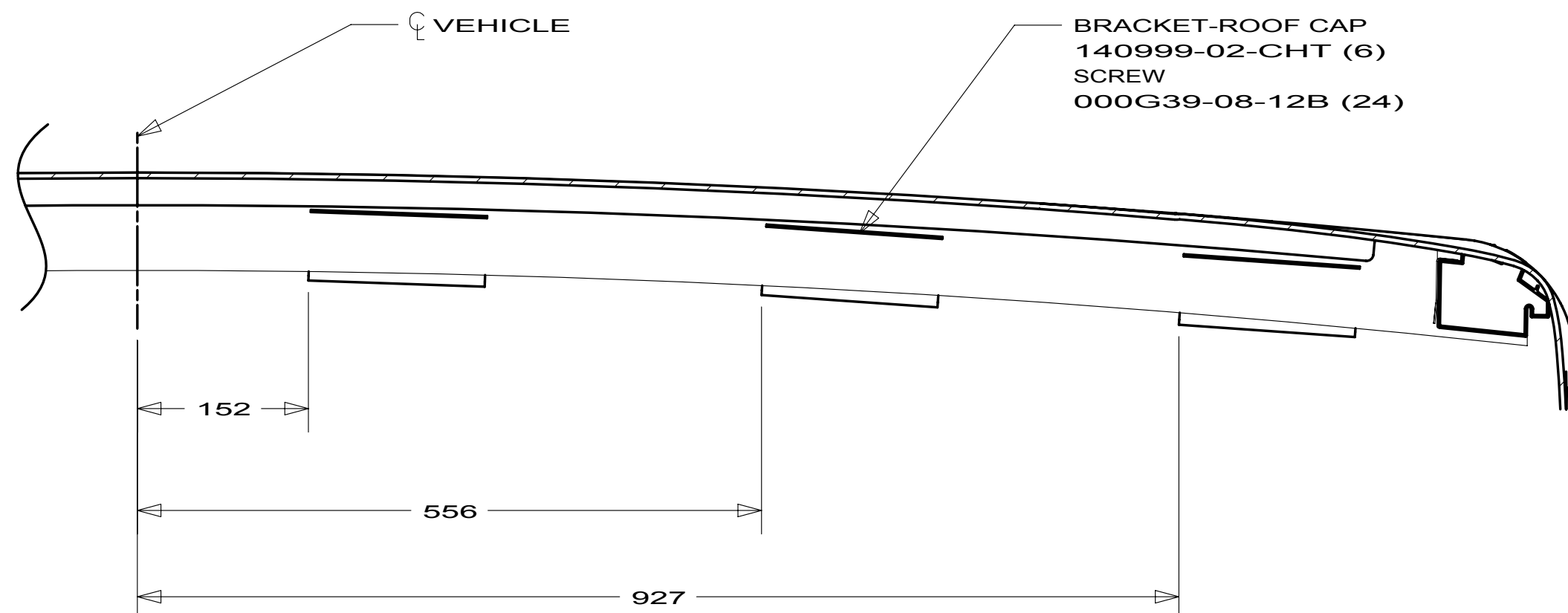
SECTION AH-AH
