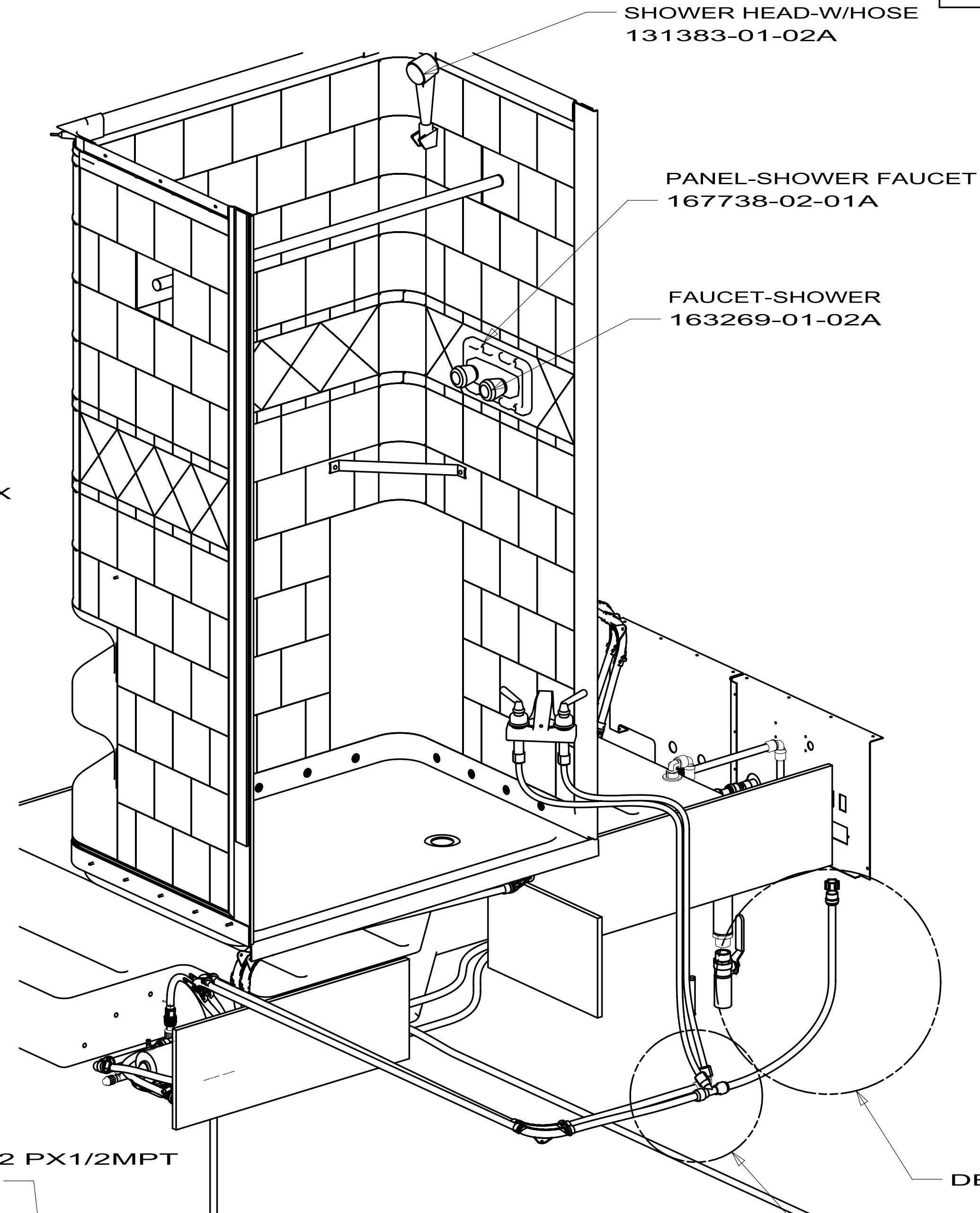
VIEW B
