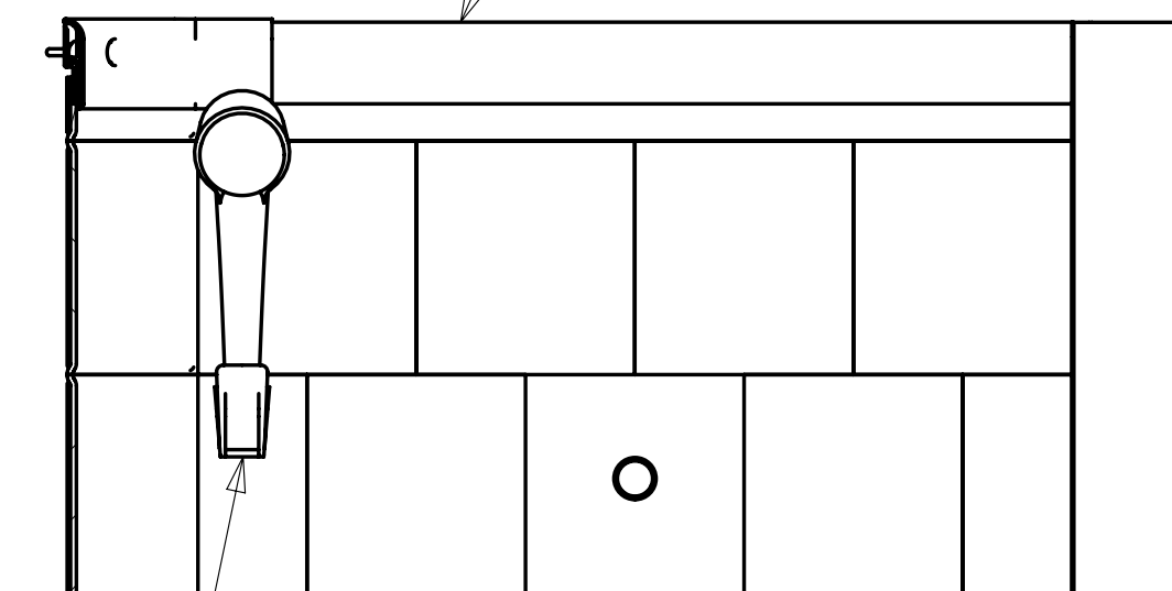
SECTION P-P
