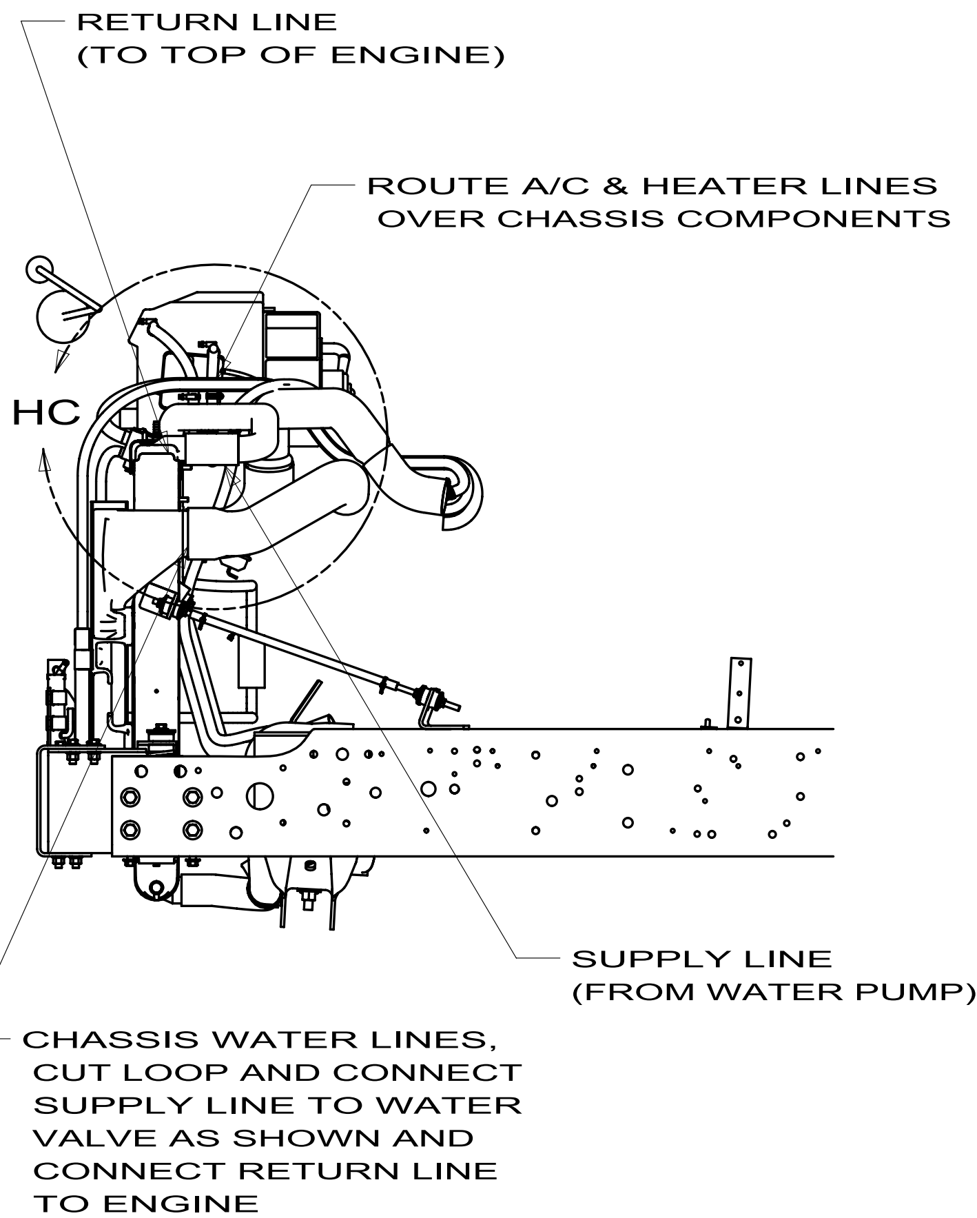
VIEW HA-HA
