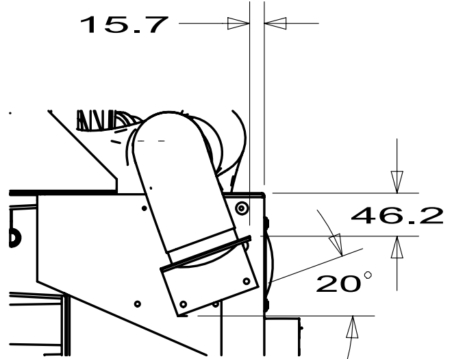
SECTION AB-AB
