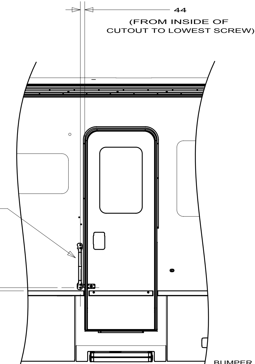
DETAIL AG
