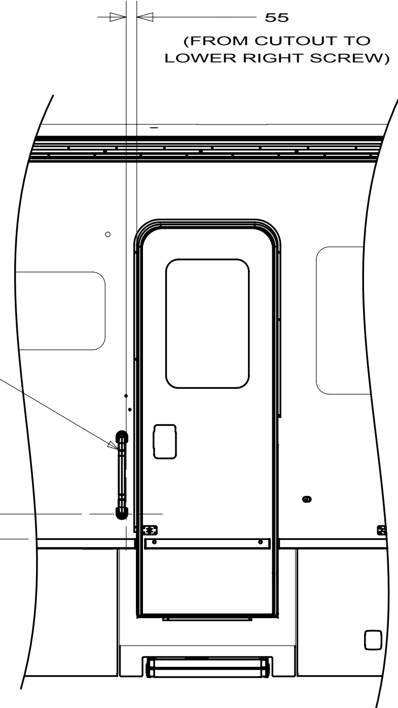
DETAIL AG
