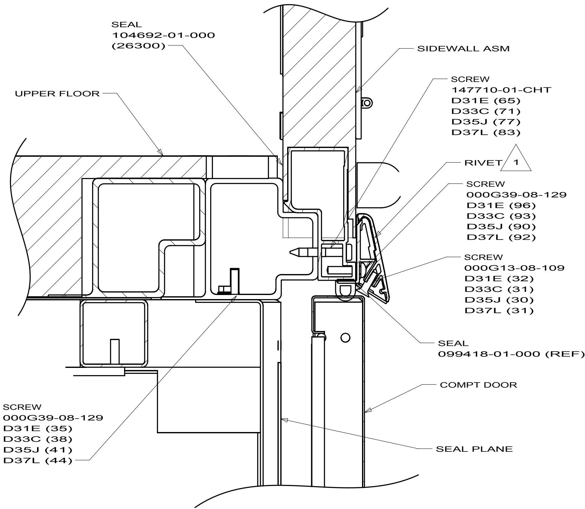
SECTION AB-AB
