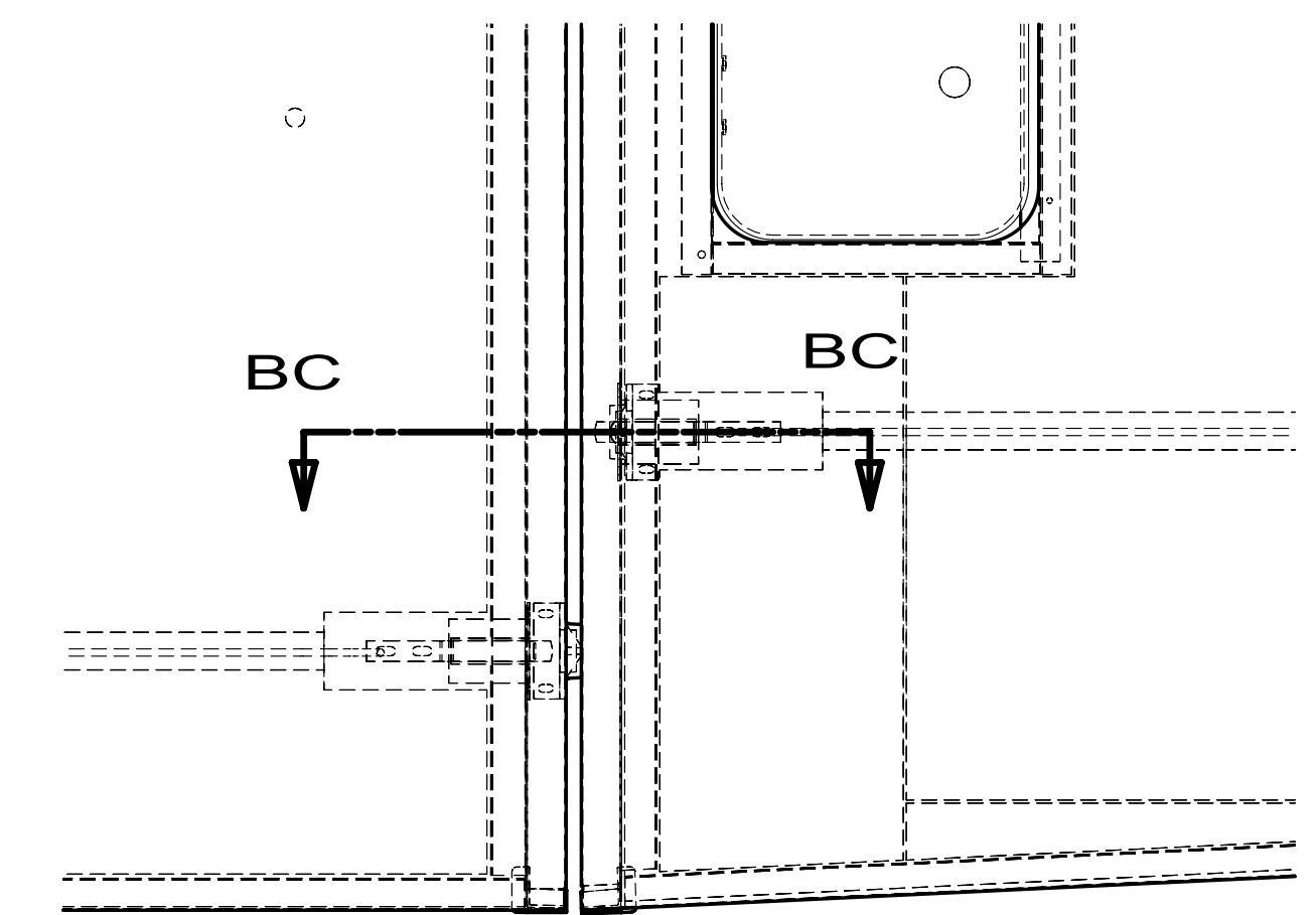
DETAIL BB
