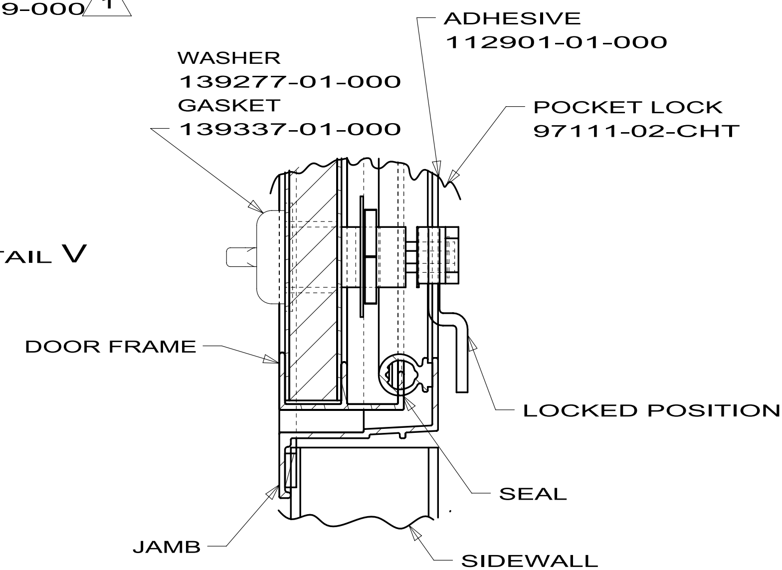
DETAIL V
