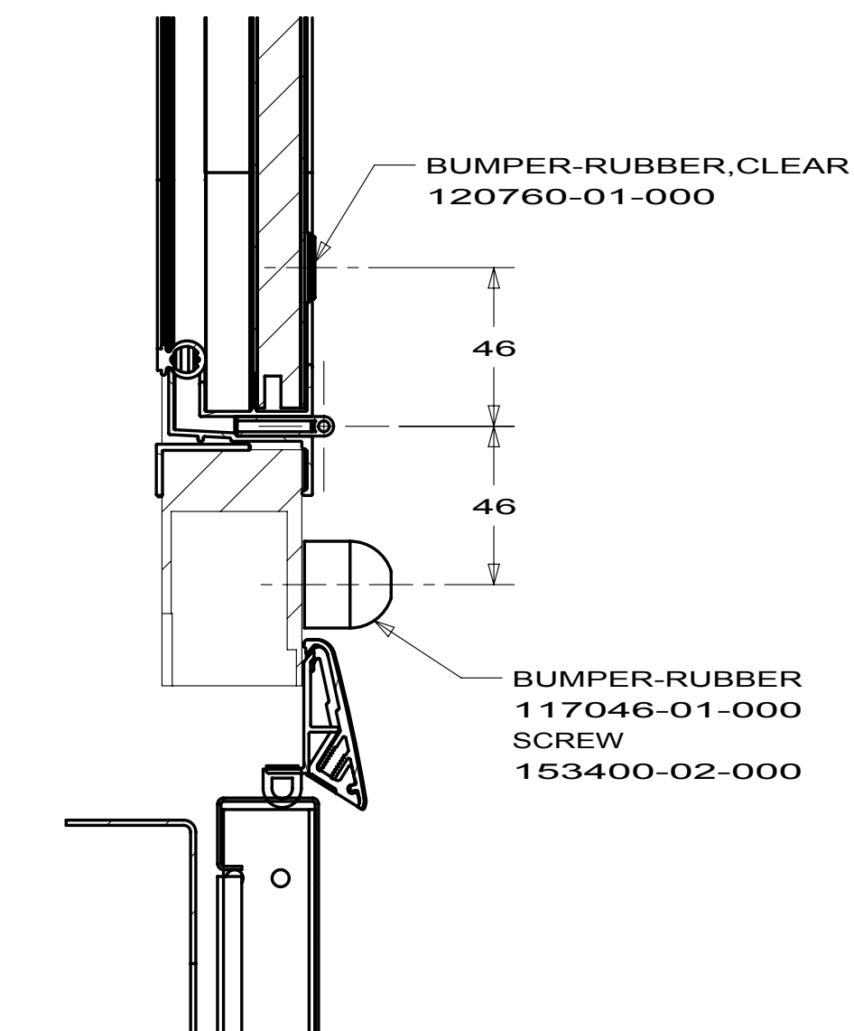
SECTION BD-BD
