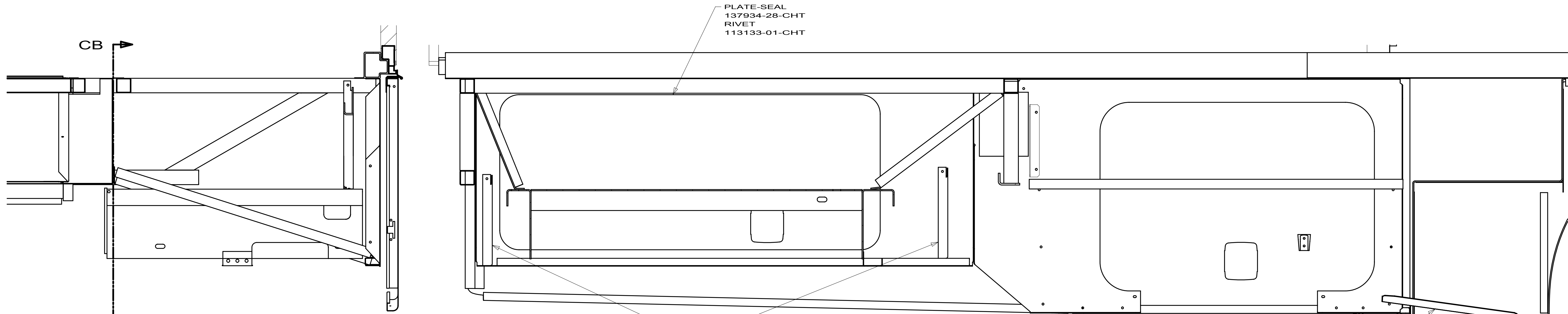
SECTION CA-CA
