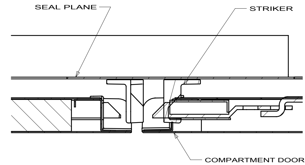
SECTION BC-BC
