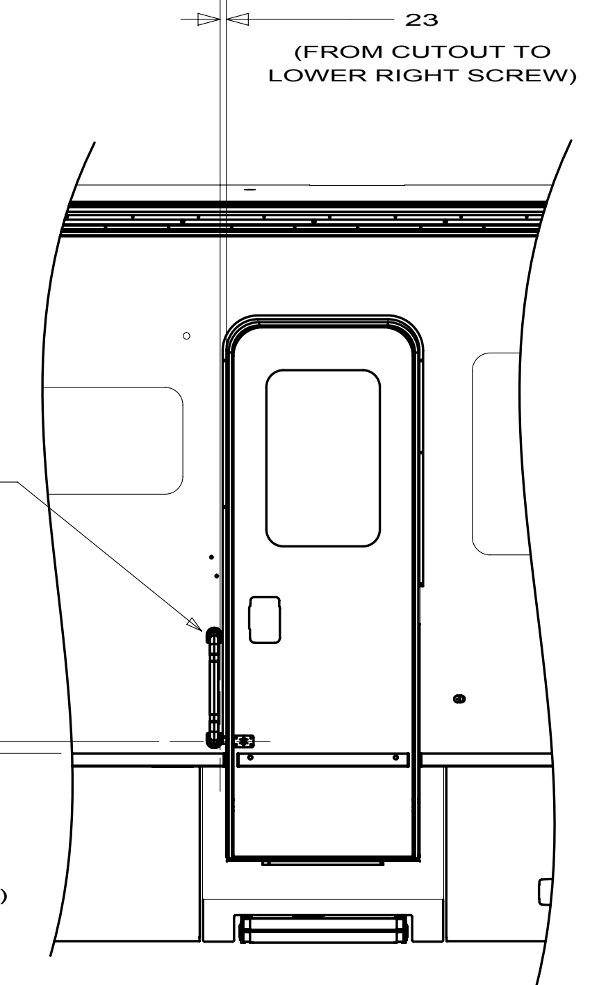
DETAIL AG
