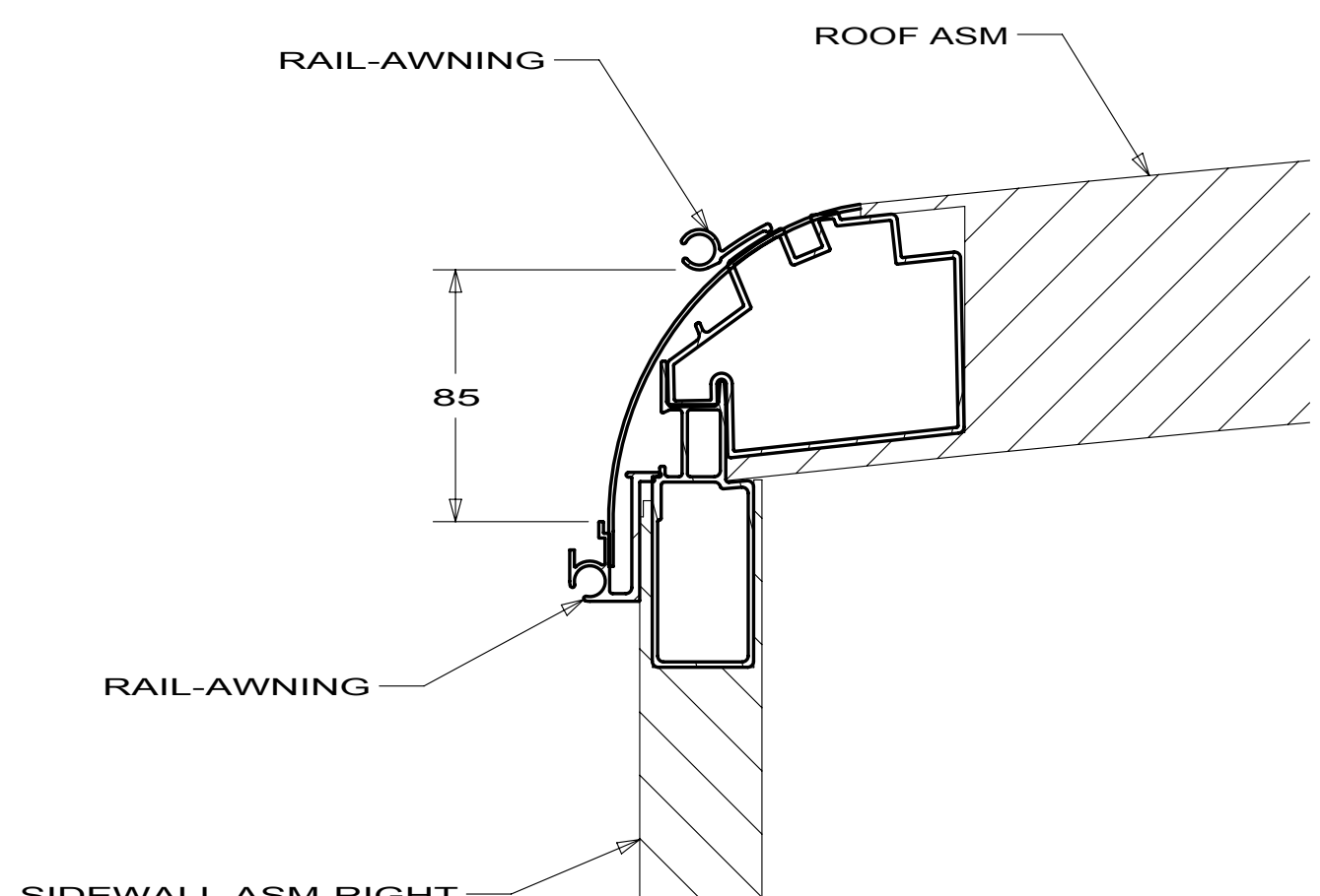
SECTION AL-AL
