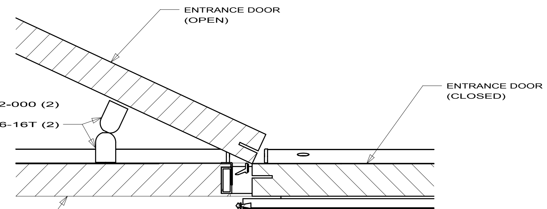
SECTION BA-BA
