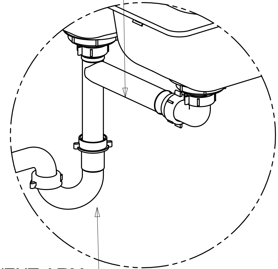
DETAIL D (SHOWN W/OUT CABINETS)
