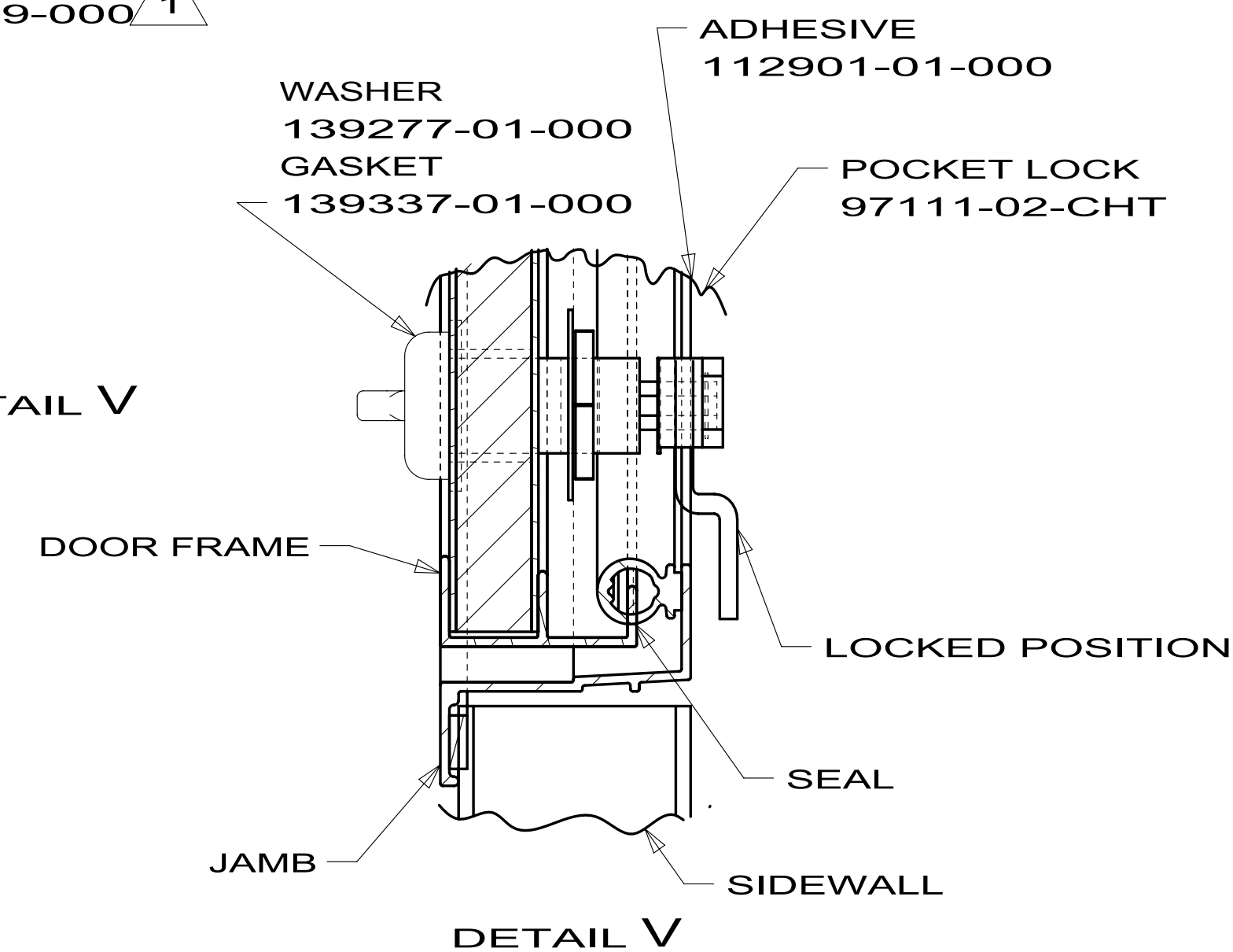
DETAIL V
